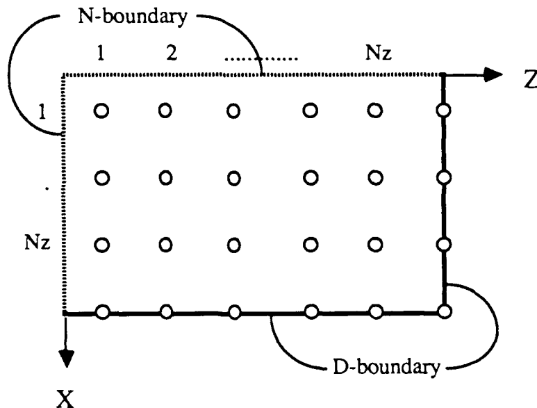
Fig. 2.5. A two-dimensional discretization example where N-D boundary condition is assumed along the x- and the z-axis.
