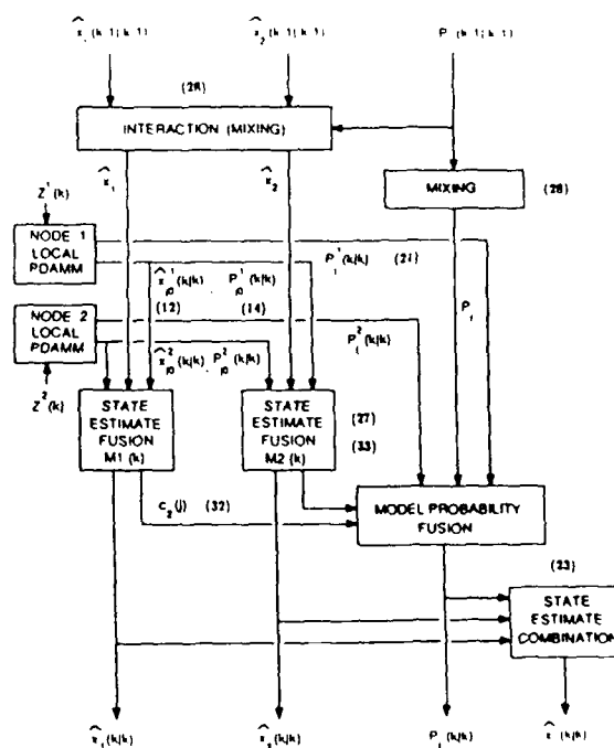
FIG. 2 Distributed MMPDA algorithm with r = 2 .
