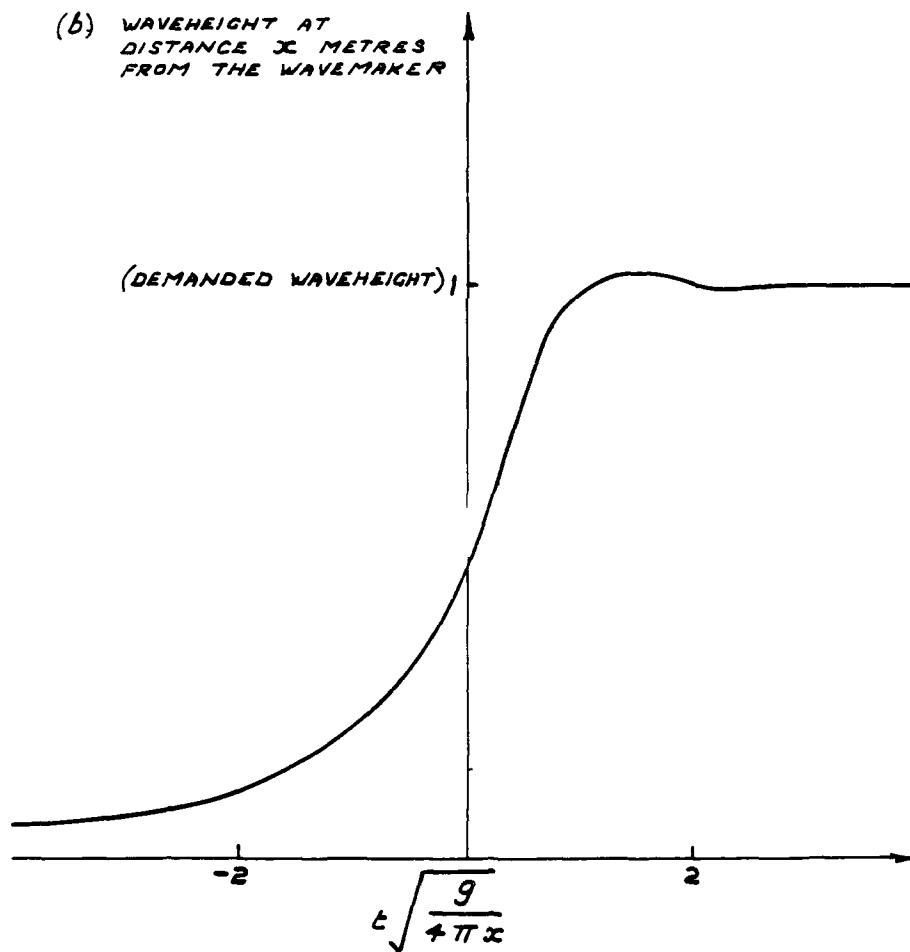
FIG 3.5 HISTORY OF WAVE AMPLITUDES - SLOW START
