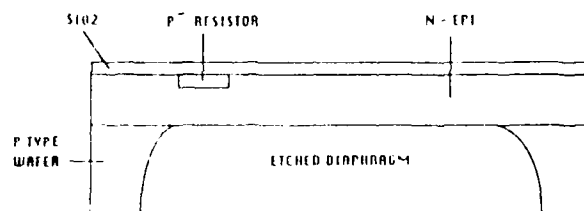
FIGURE 1. SILICON DIE AFTER ETCHING, P - IMPLANT, AND \text{SiO}_2 DEPOSITION
