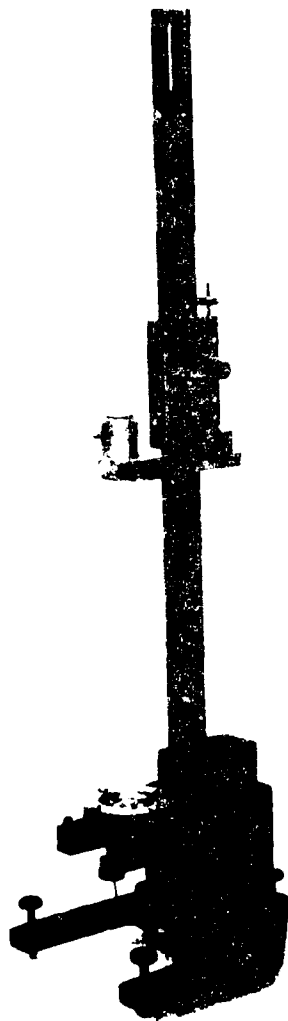
FIGURE 1 OVERALL VIEW OF THE CALIBRATION APPARATUS (NOT TO SCALE)
