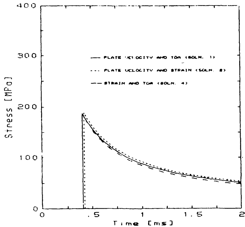
FIGURE 9. Soil Stress vs. Time at x_g = .381 m, FP 8-3
