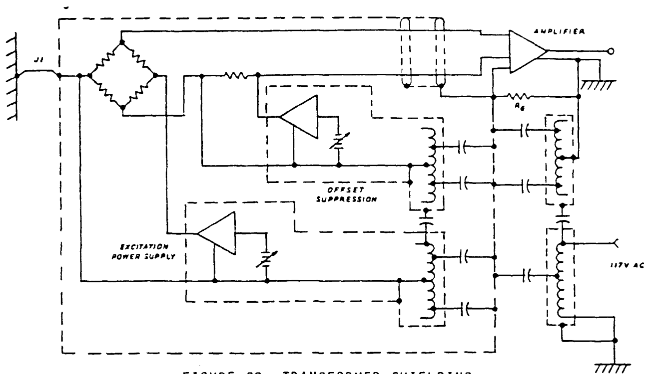
FIGURE 22 TRANSFORMER SHIELDING
