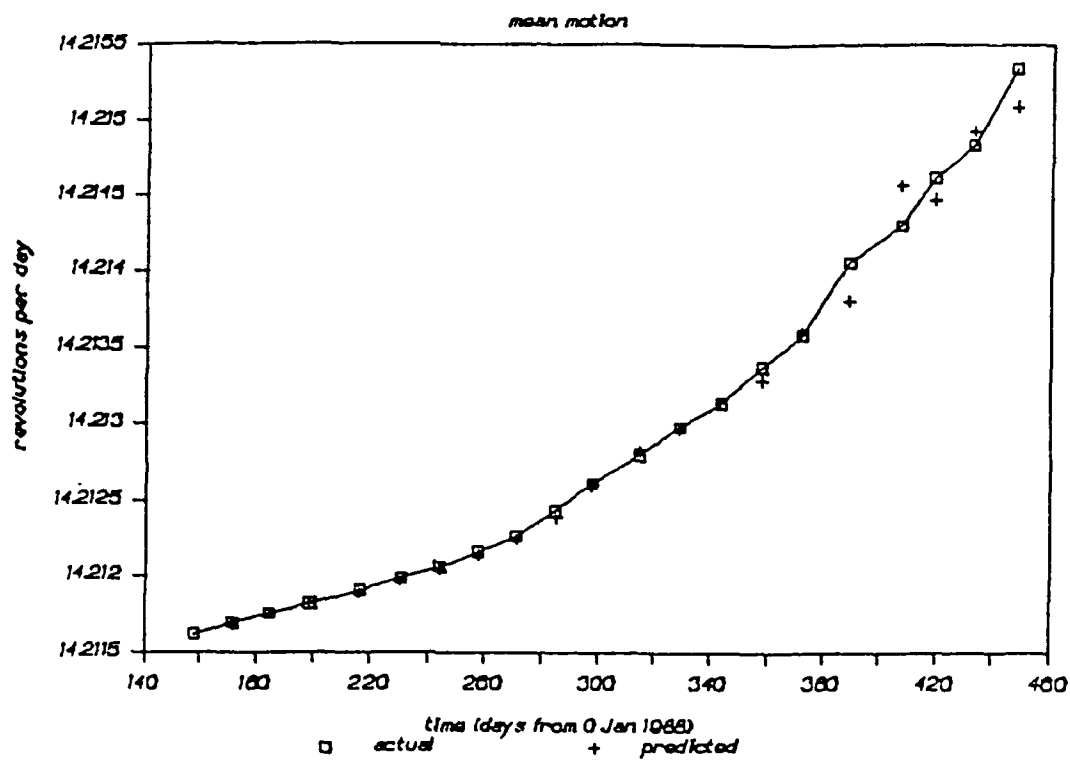
Figure 1.4. Mean motion
