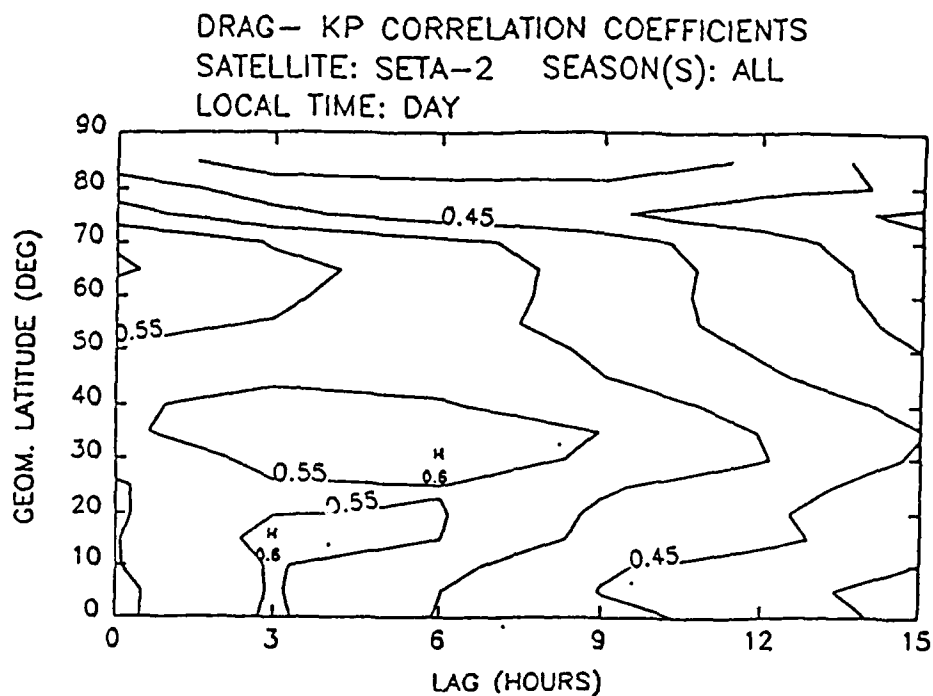
Figure 2.14. Same as Figure 2.6, except SETA-2, all seasons
