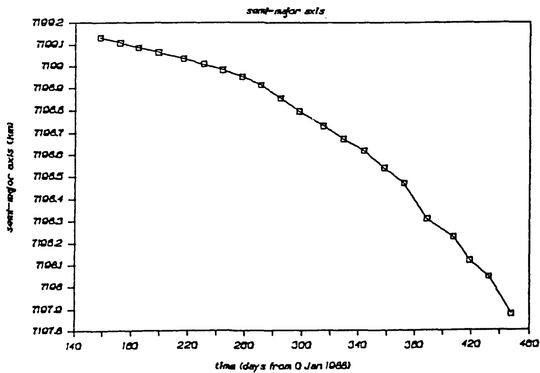
Figure 1.7. Semi-major axis
