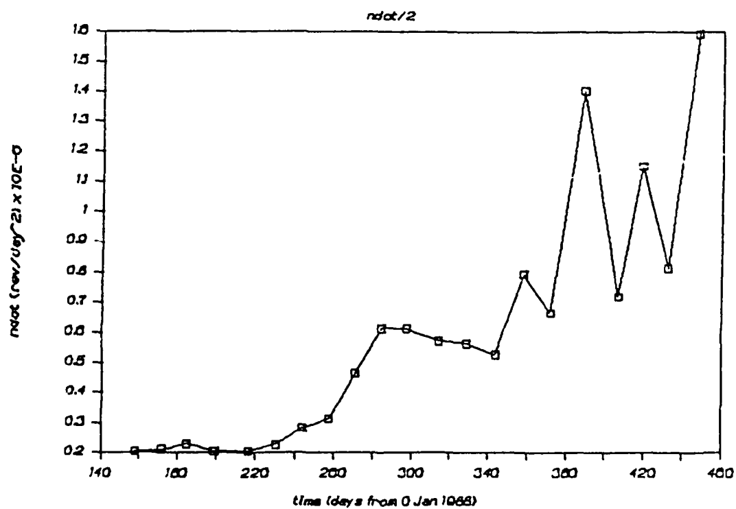
Figure 1.5. Derivative of mean motion
