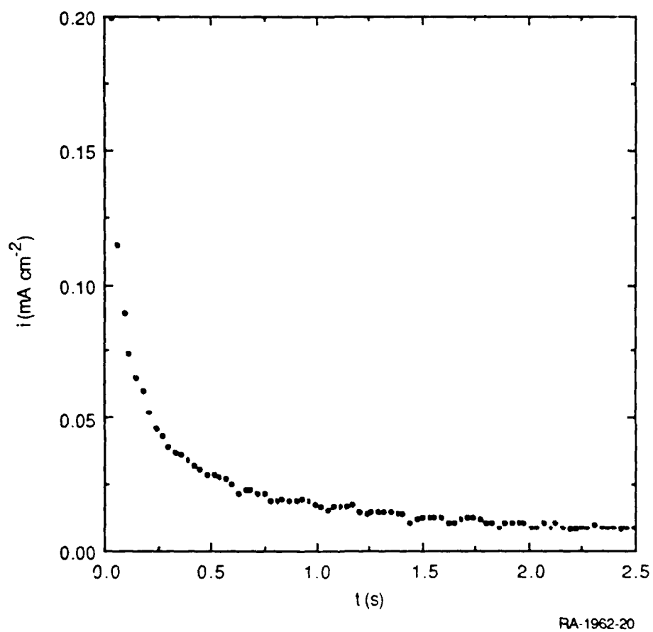
Figure 2. Anodic transient for titanium grade 2 in acetate buffer. t_c = 15 \text{ s} ; E_c = -0.742 \text{ V (SCE)} . The full transient is not shown.
