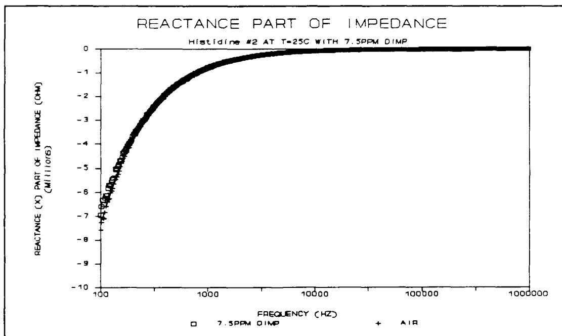
Figure F.10. Reactive Part of the Impedance for the L-Histidine Dihydrochloride Film upon Exposure to the 7.5 ppm DIMP Challenge at 25 °C.
