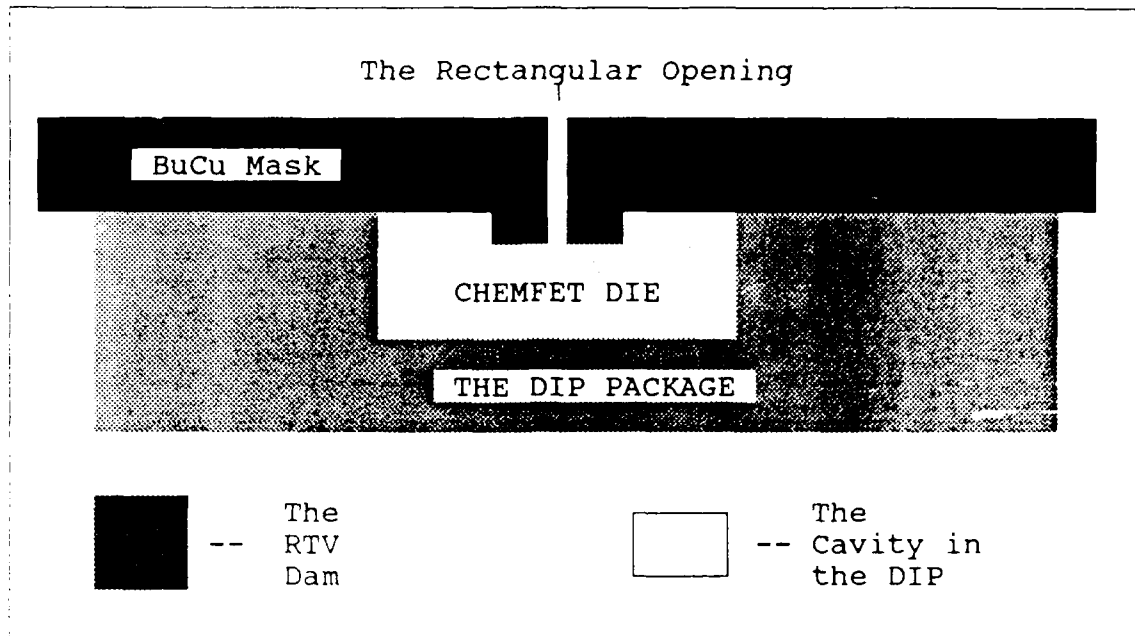
Figure C.3. CHEMFET Mask Arrangement for Thermal Evaporation.
