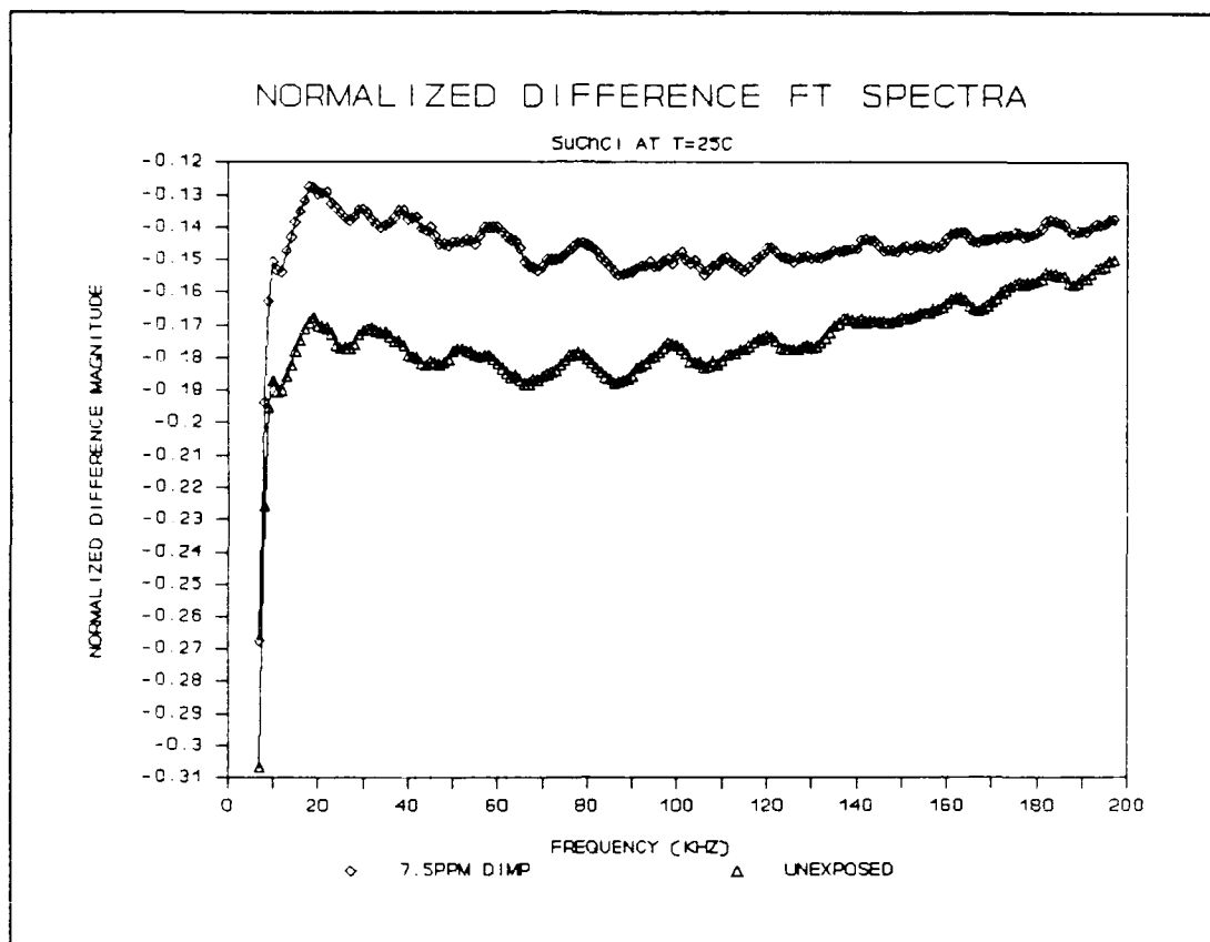
Figure V.41. Normalized Difference Fourier Transform Spectra of the CHEMFET Sensor Coated with the Succinylcholine Chloride Film upon Exposure to the 7.5 ppm DIMP Challenge at 25 °C.
