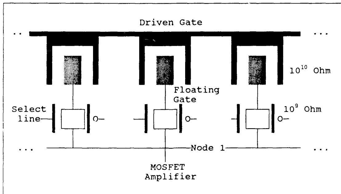
Figure III.11. Floating Gates Connected to Multiplexer.
