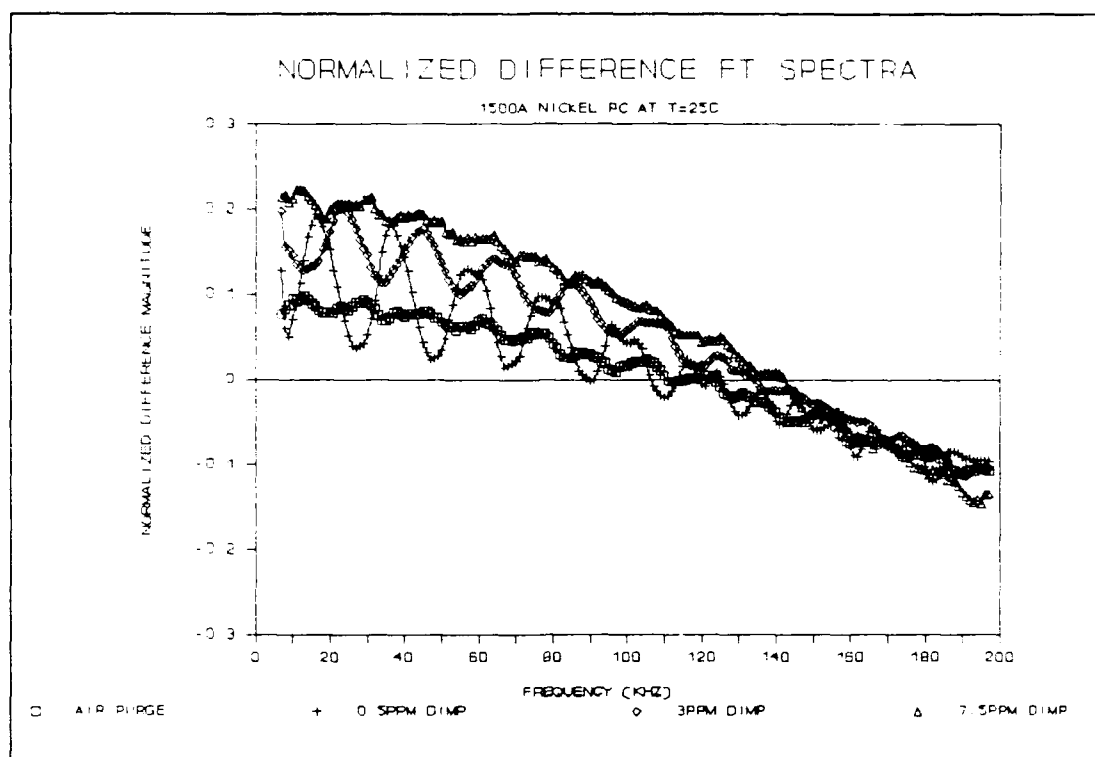
Figure V.13. Normalized Difference Fourier Transform Spectra of the CHEMFET Sensor Coated with the 1500Å Thick NiPc Film upon Exposure to the DIMP Challenge at 25 °C.
