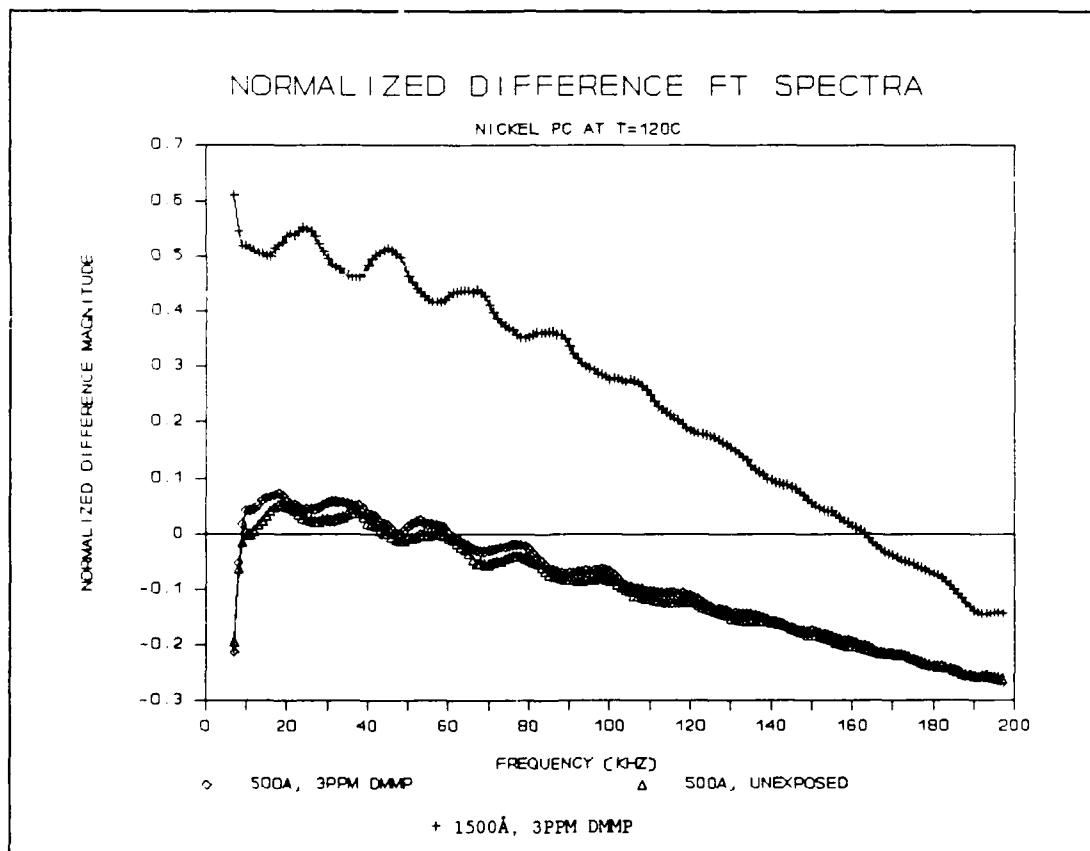
Figure V.18. Normalized Difference Fourier Transform Spectra of the CHEMFET Sensors Coated with the 500Å and 1500Å Thick NiPc Films upon Exposure to the 3 ppm DMMP Challenge at 120 °C.
