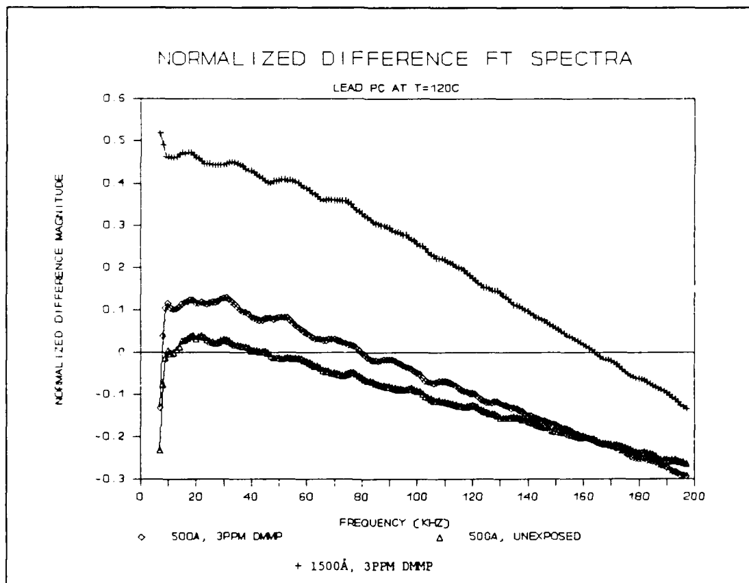
Figure V.24. Normalized Difference Fourier Transform Spectra of the CHEMFET Sensors Coated with the 500Å and 1500Å Thick PbPc Films upon Exposure to the 3 ppm DMMP Challenge at 120 °C.
