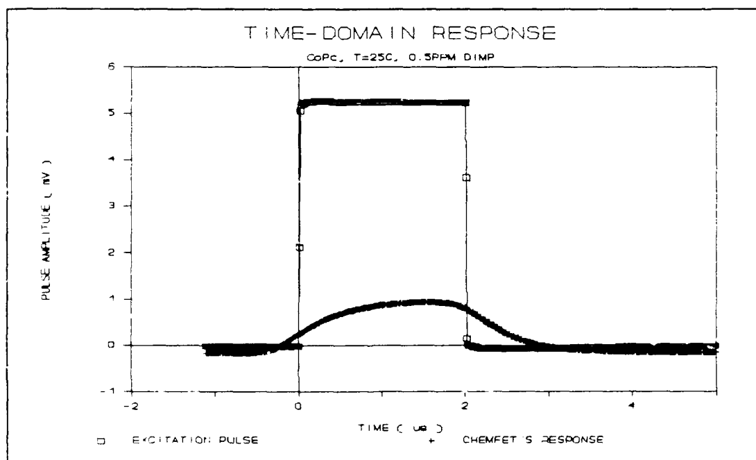
Figure V.3. Time-Domain Response of the CHEMFET Sensor Coated with a 1500Å Thick CoPc Film upon Exposure to a 0.5 ppm DIMP Challenge at 25 °C.
