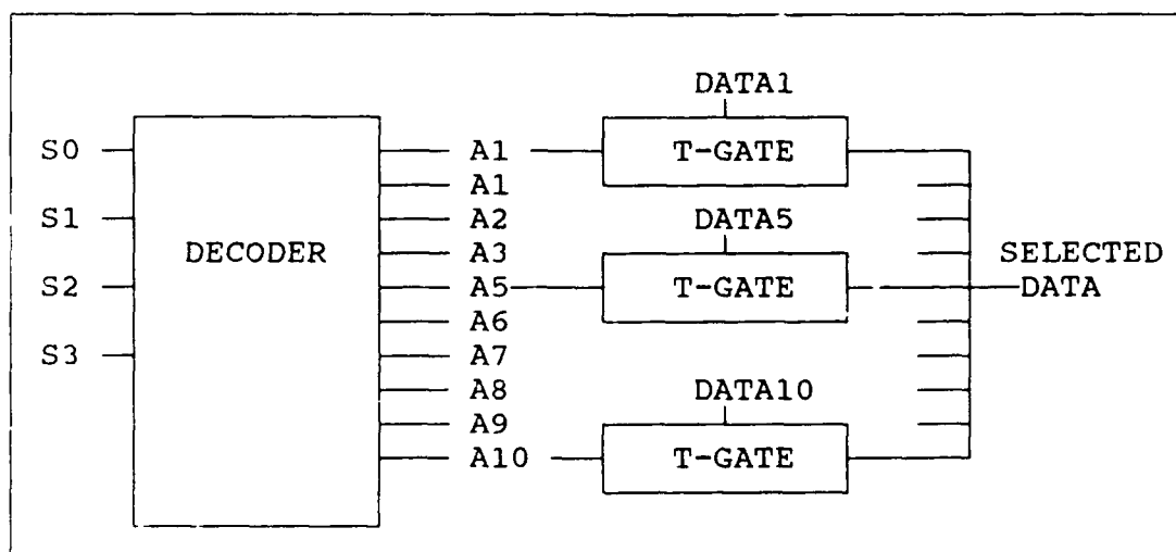
Figure III.1. CHEMFET Multiplexer.
