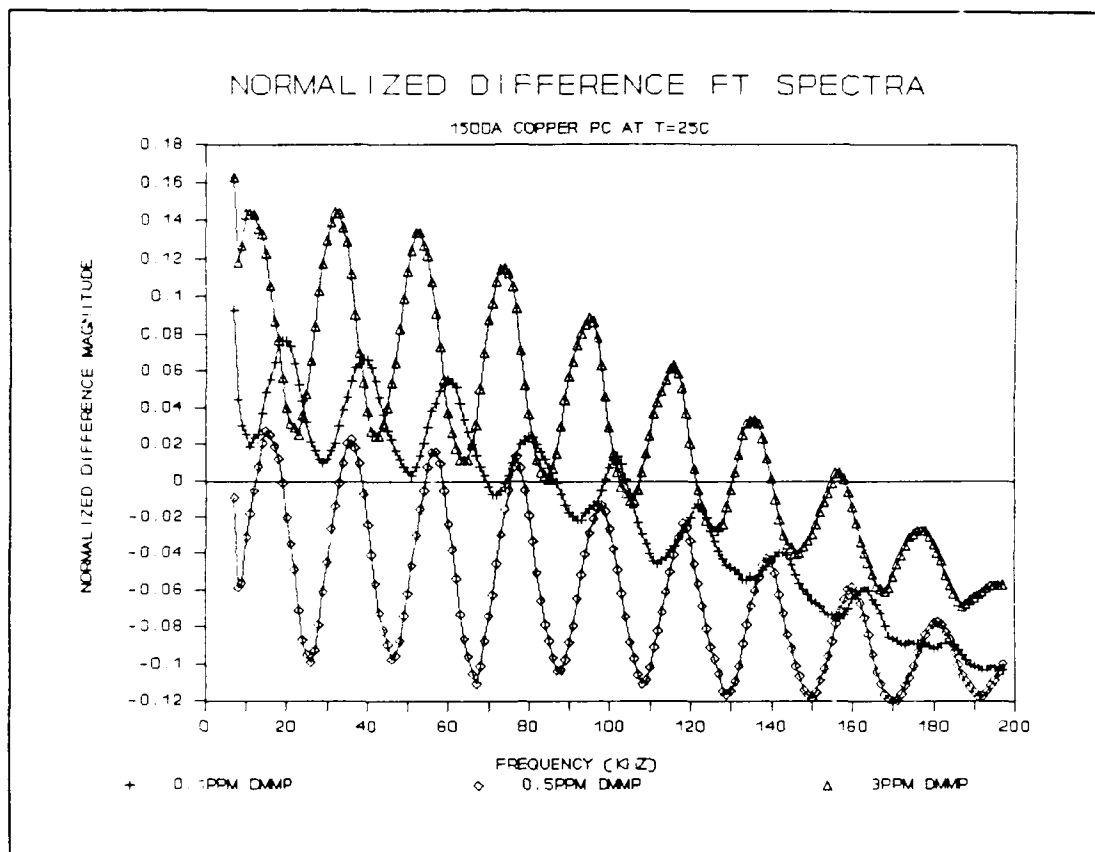
Figure V.28. Normalized Difference Fourier Transform Spectra of the CHEMFET Sensor Coated with the 1500Å Thick CuPc Film upon Exposure to the DMMP Challenge at 25 °C.
