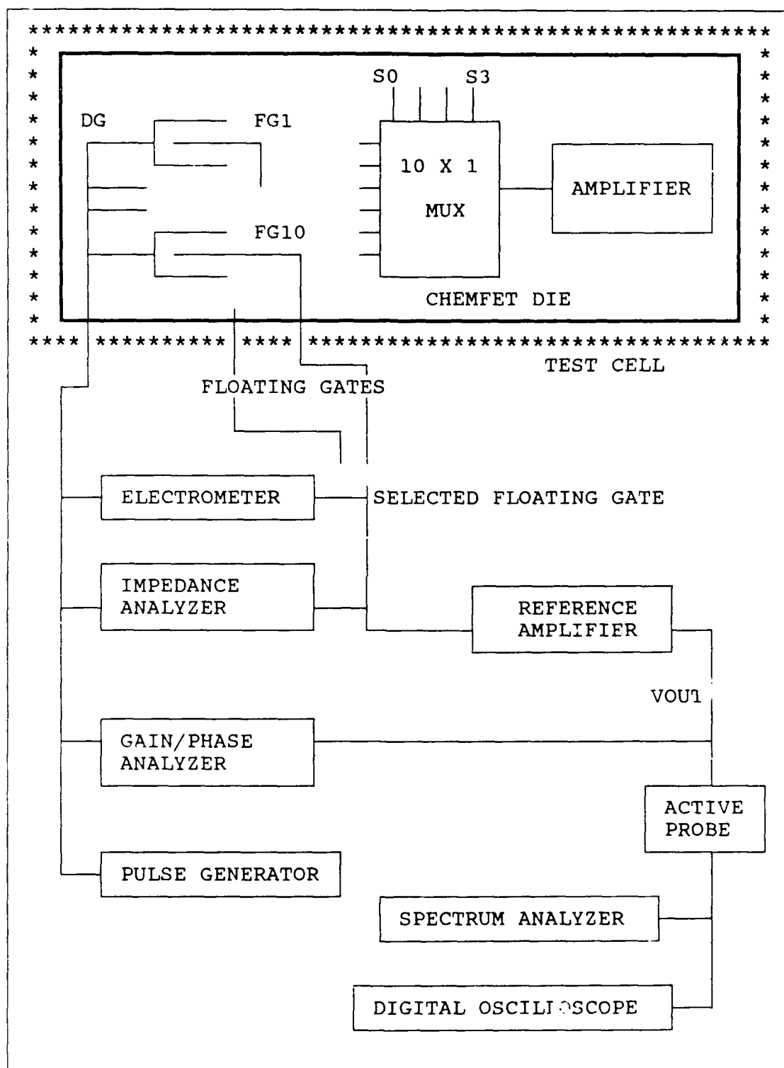
Figure IV.4. Instrumentation Configuration.
