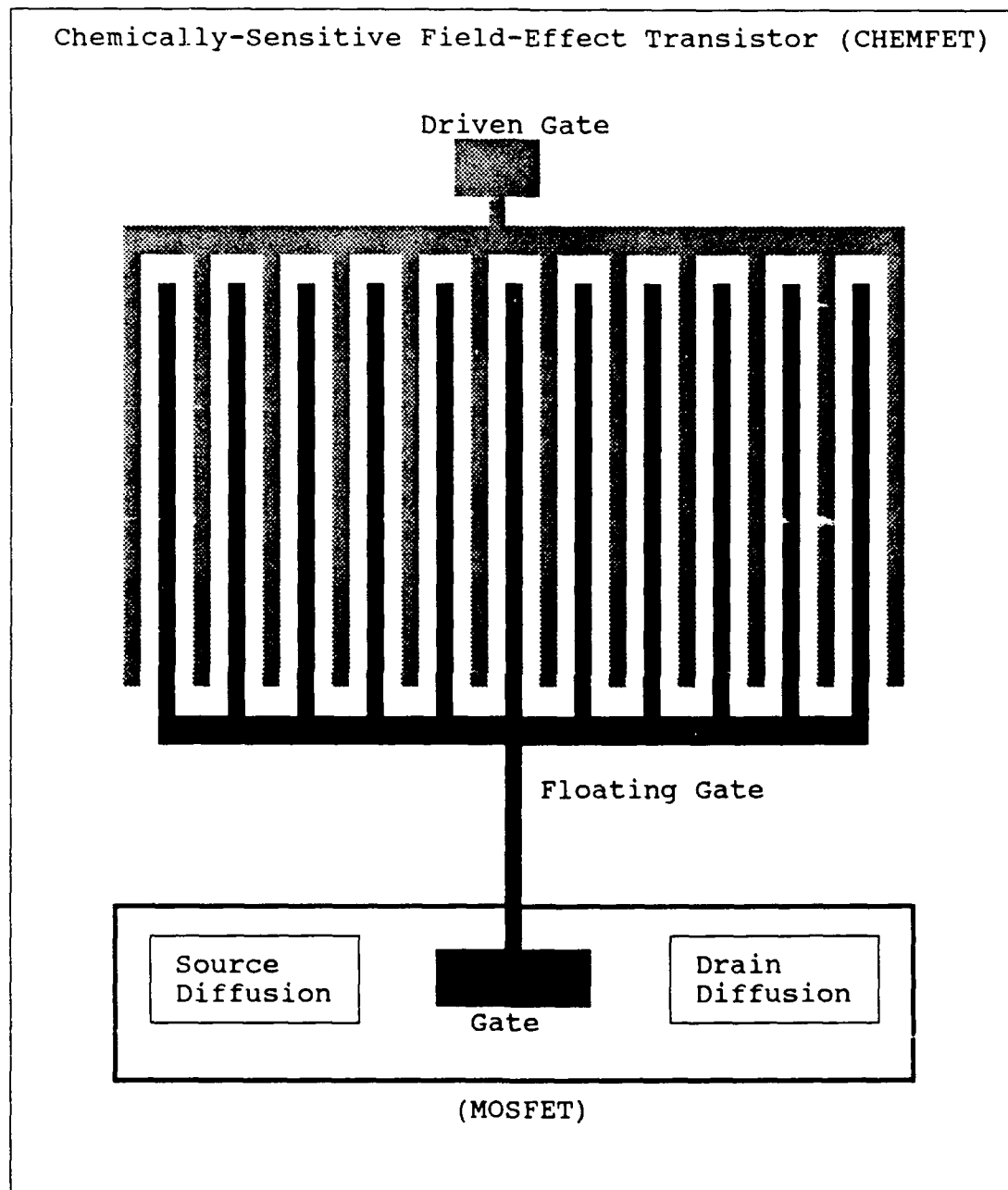
Figure I.1. Interdigitated Gate Electrode CHEMFET (1:1-3).
