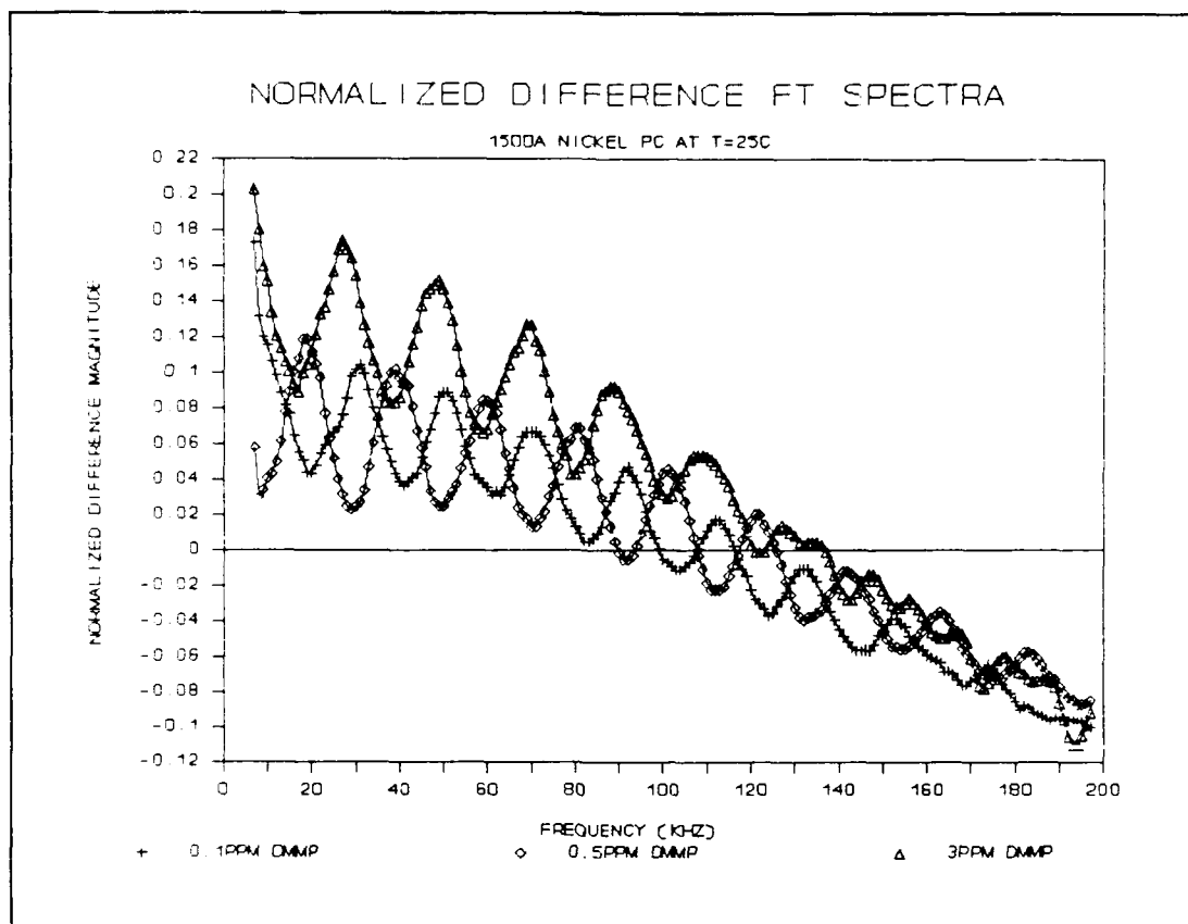
Figure V.16. Normalized Difference Fourier Transform Spectra of the CHEMFET Sensor Coated with the 1500Å Thick NiPc Film upon Exposure to the DMMP Challenge at 25 °C.
