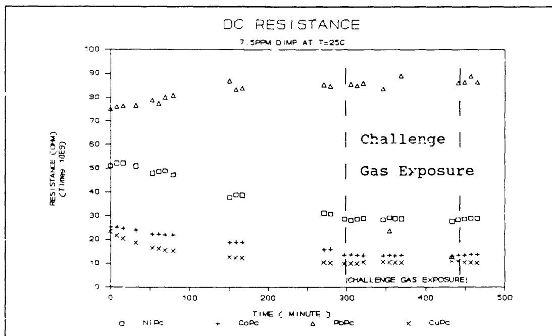
Figure V.7. DC Resistance of the 1500Å Thick Metal-Doped Phthalocyanine Films upon Exposure to the 7.5 ppm DIMP Challenge at 25 °C.
