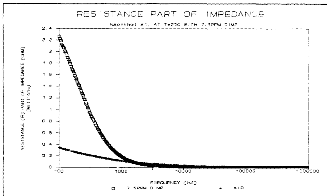
Figure F.1. Resistive Part of the Impedance for the 2-Naphthol( \beta ) Film upon Exposure to the 7.5 ppm DIMP Challenge at 25°C.
