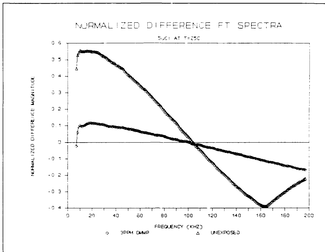
Figure V.37. Normalized Difference Fourier Transform Spectra of the CHEMFET Sensor Coated with the Succinylchloride Film upon Exposure to the 3 ppm DMMP challenge at 25 °C.
