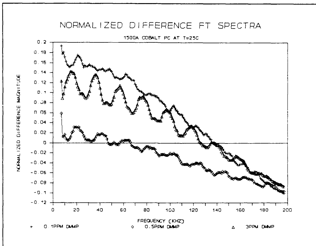
Figure V.10. Normalized Difference Fourier Transform Spectra of the CHEMFET Sensor Coated with the 1500Å Thick CoPc Film upon Exposure to DMMP at 25 °C.
