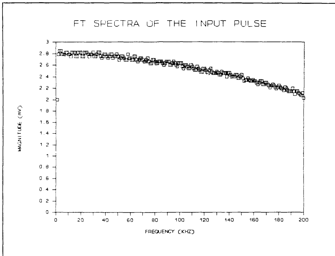
Figure IV.8. Fourier Transform Spectra of the Excitation Pulse.
