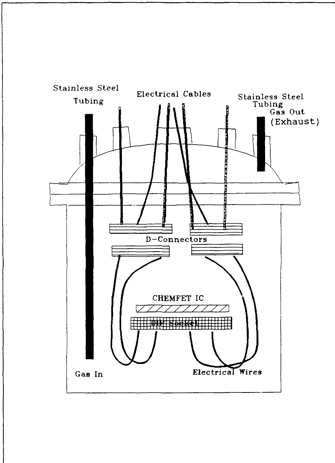
Figure D.7. Schematic Drawing of the Test Cell.
