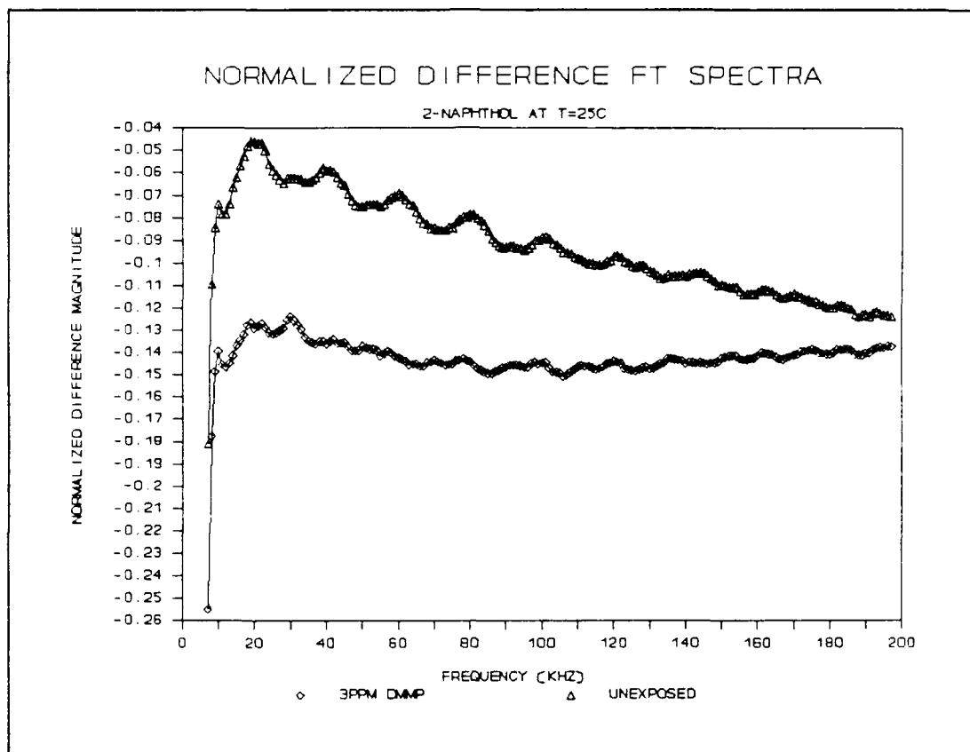
Figure V.33. Normalized Difference Fourier Transform Spectra of the CHEMFET Sensor Coated with the 2-Naphthol( \beta ) upon Exposure to the 3 ppm DMMP Challenge at 25 °C.
