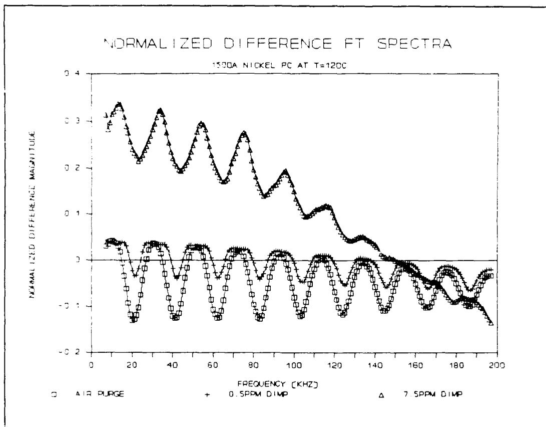
Figure V.14. Normalized Difference Fourier Transform Spectra of the CHEMFET Sensor Coated with the 1500Å Thick NiPc Film upon Exposure to the DIMP Challenge at 120 °C.
