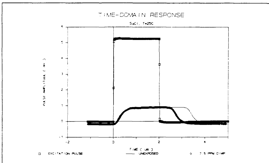
Figure V.36. Time-Domain Response of the CHEMFET Sensor Coated with the Succinylchloride Film upon Exposure to the 7.5 ppm DIMP Challenge at 25 °C.
