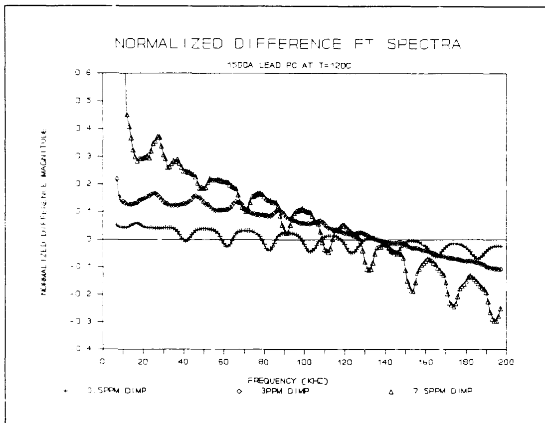
Figure V.20. Normalized Difference Fourier Transform Spectra of the CHEMFET Sensor Coated with 1500Å Thick PbPc upon Exposure to DIMP at 120 °C.
