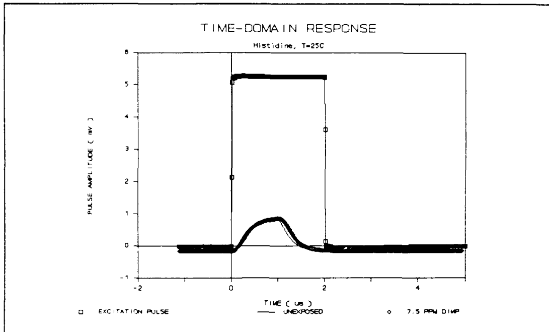
Figure V.39. Time-Domain Response of the CHEMFET Sensor Coated with the L-Histidine Dihydrochloride Film upon Exposure to the 7.5 ppm DIMP Challenge at 25 °C.
