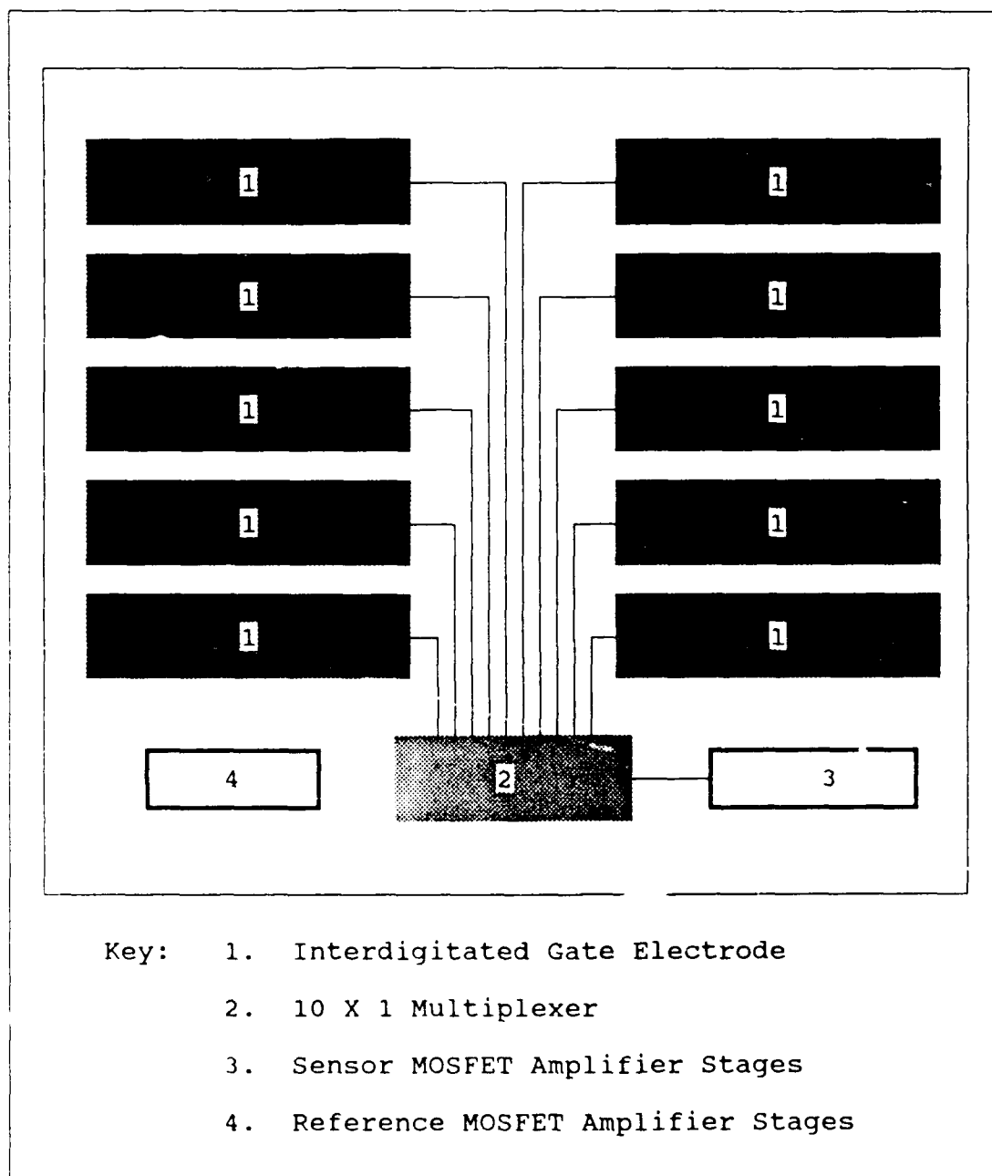
Figure I.2. 2 X 5 CHEMFET Array Layout.
