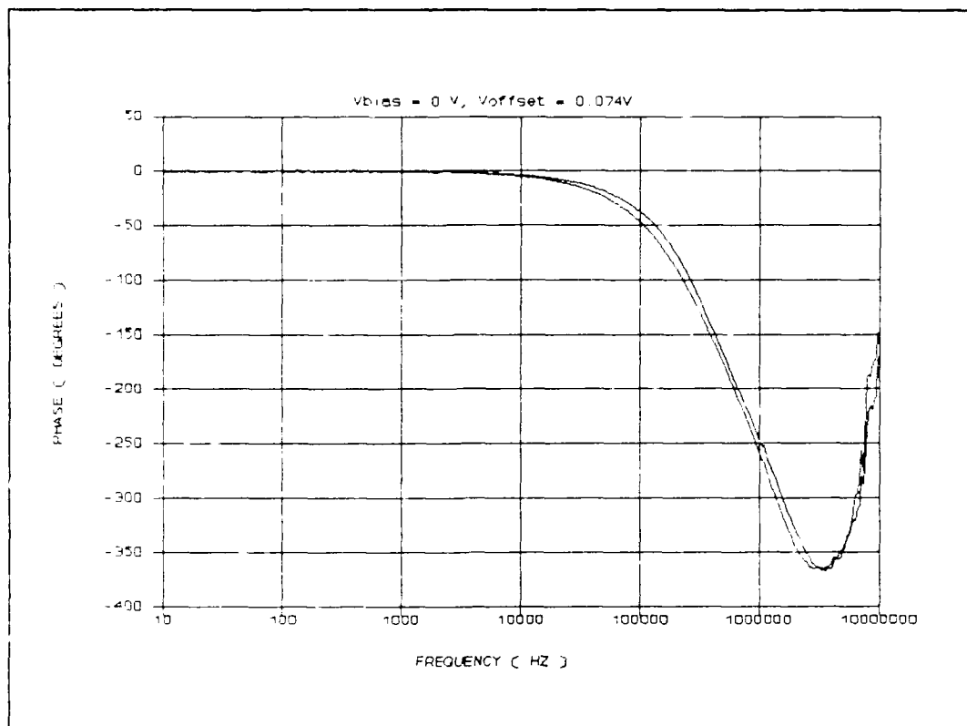
Figure III.10. Phase of the Interdigitated Gate Electrode CHEMFET's Amplifier versus Frequency.
