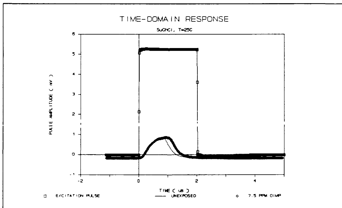
Figure V.42. Time-Domain Response of the CHEMFET Sensor Coated with the Succinylcholine Chloride Film upon Exposure to the 7.5 ppm DIMP Challenge at 25 °C.
