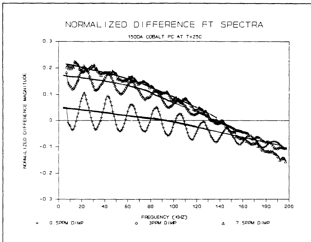
Figure V.1. Normalized Difference Fourier Transform Spectra of the CHEMFET Sensor Coated with a 1500Å Thick CoPc Film upon Exposure to DIMP at 25 °C.
