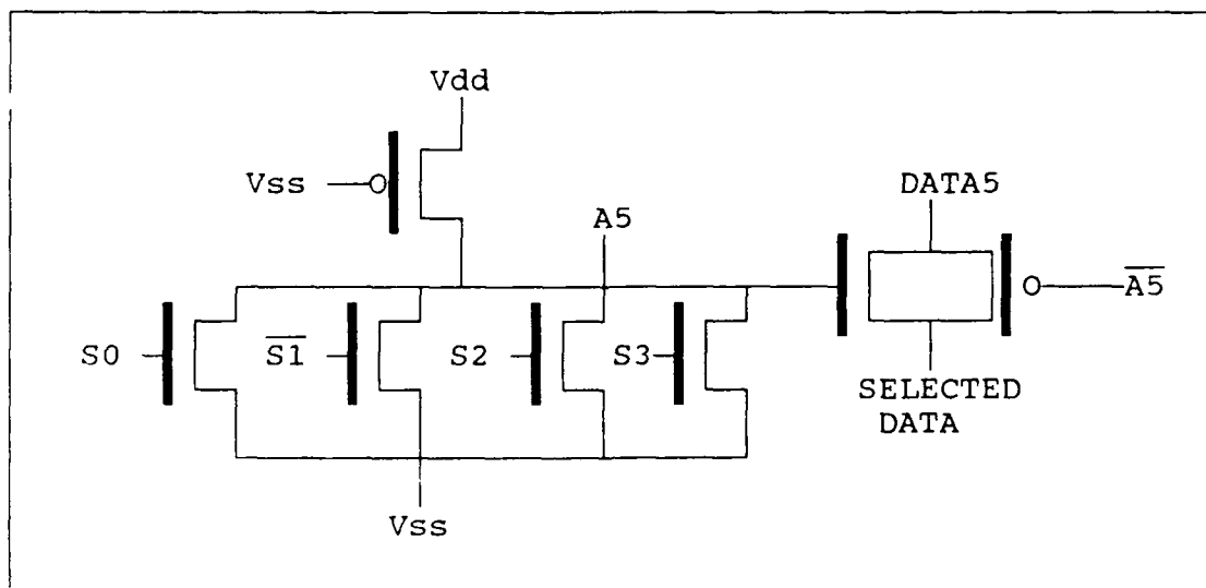
Figure III.2. Decoder and Transmission Gates.
