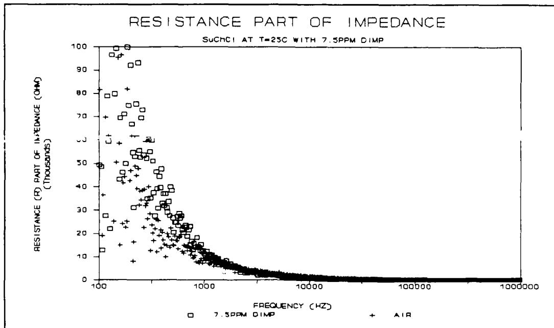
Figure F.13. Resistive Part of the Impedance for the Succinylcholine Chloride Film upon Exposure to the 7.5 ppm DIMP Challenge at 25 °C.
