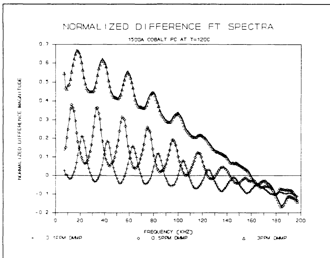
Figure V.11. Normalized Difference Fourier Transform Spectra of the CHEMFET Sensor Coated with the 1500Å Thick CoPc Film upon Exposure to DMMP at 120 °C.
