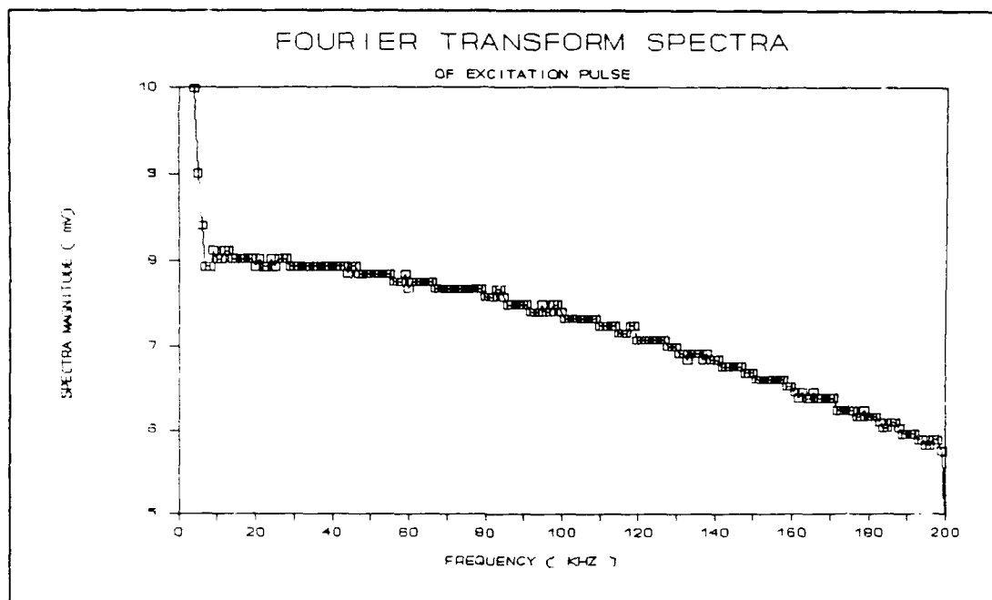
Figure V.2. Fourier Transform Spectra of the Excitation Pulse Offset at -40 mV.
