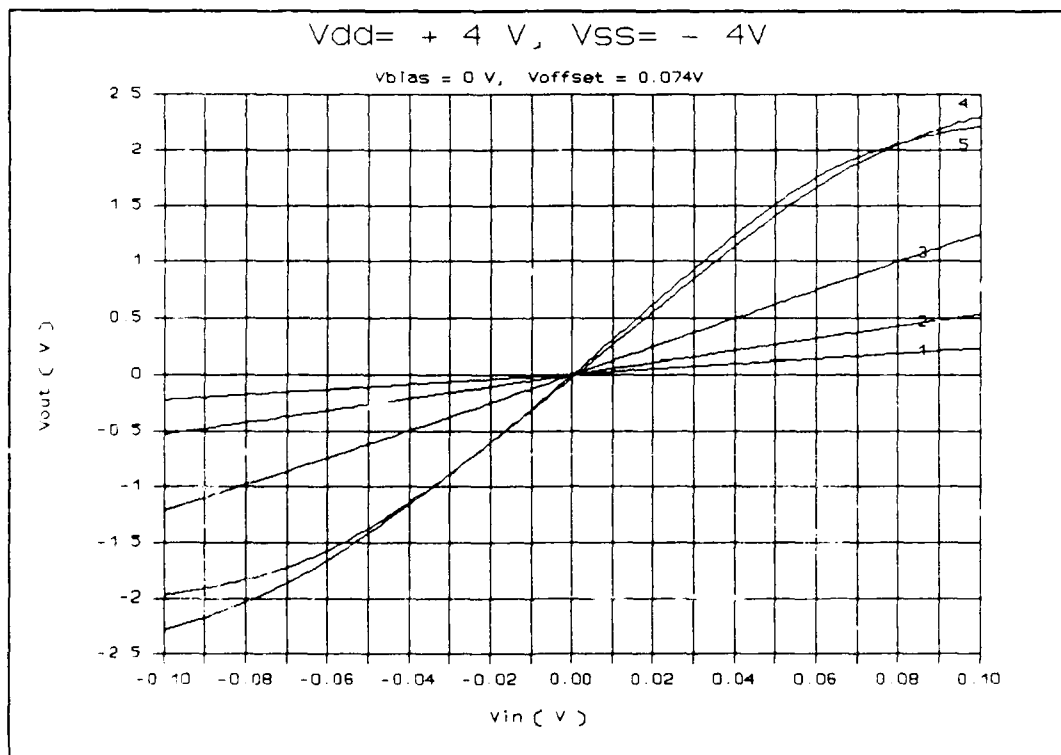
Figure III.8. DC Voltage Characteristics of the Five Amplifier Stages.
