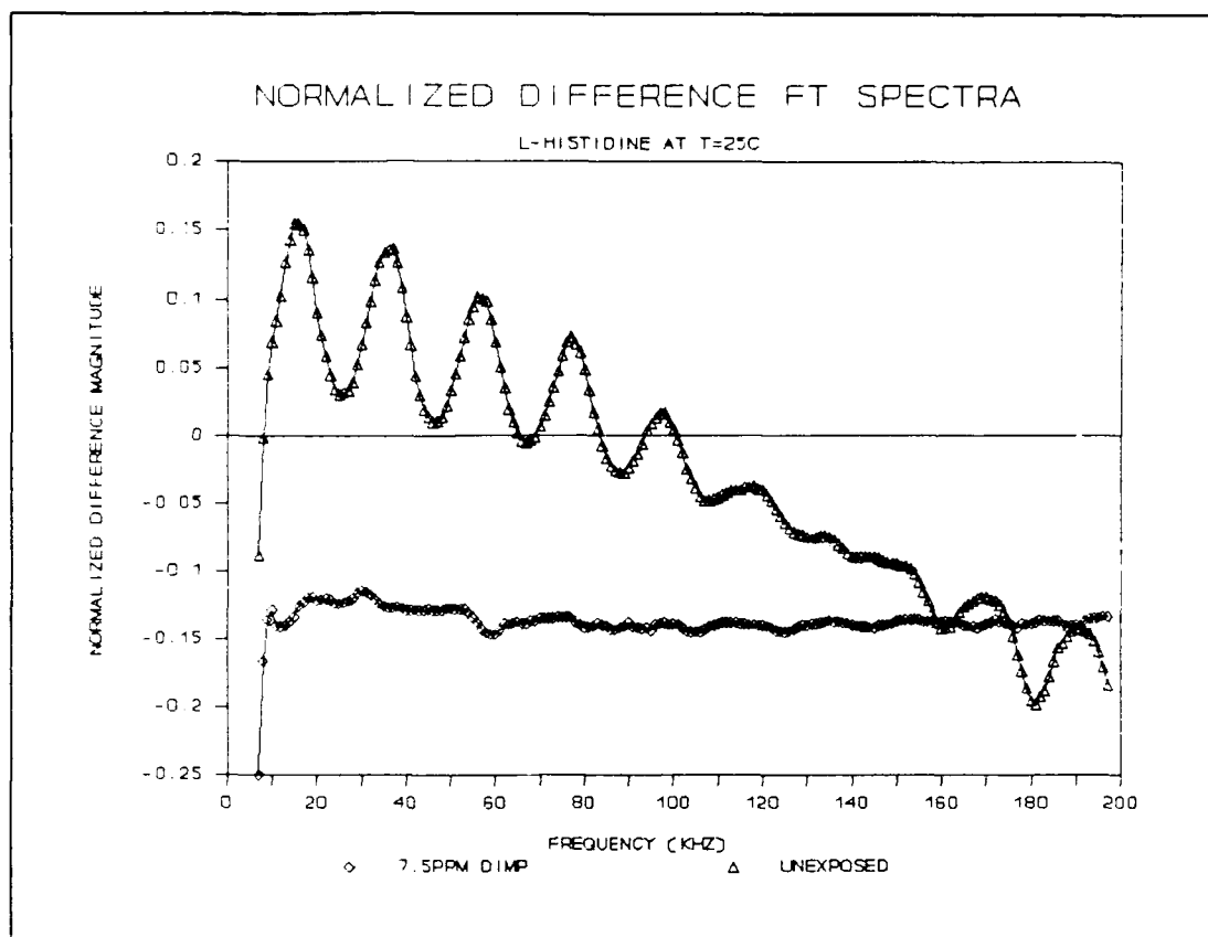
Figure V.38. Normalized Difference Fourier Transform Spectra of the CHEMFET Sensor Coated with the L-Histidine Dihydrochloride Film upon Exposure to the 7.5 ppm DIMP Challenge at 25 °C.
