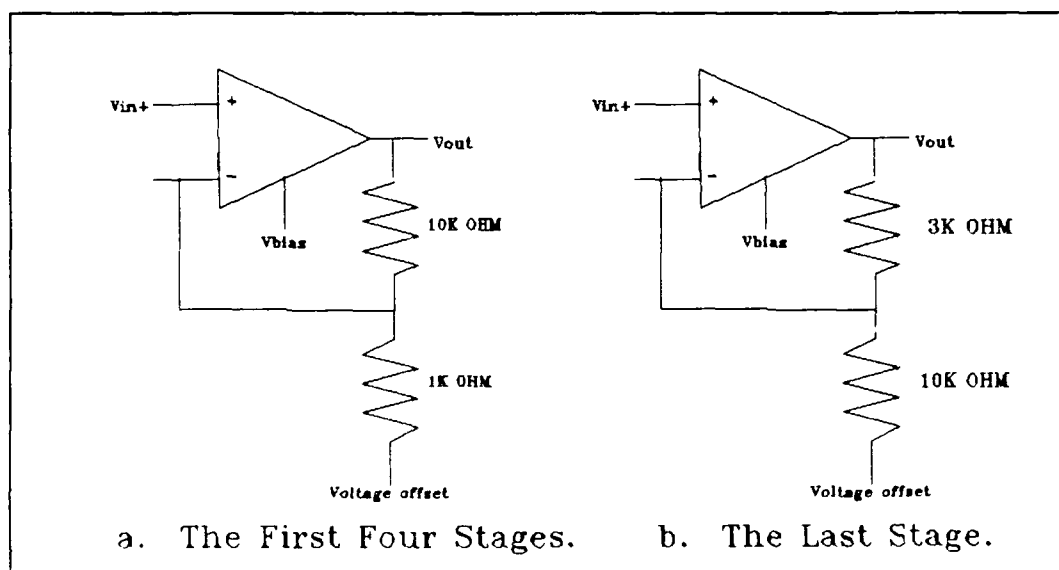
Figure III.4. Feedback Amplifier Stages.
