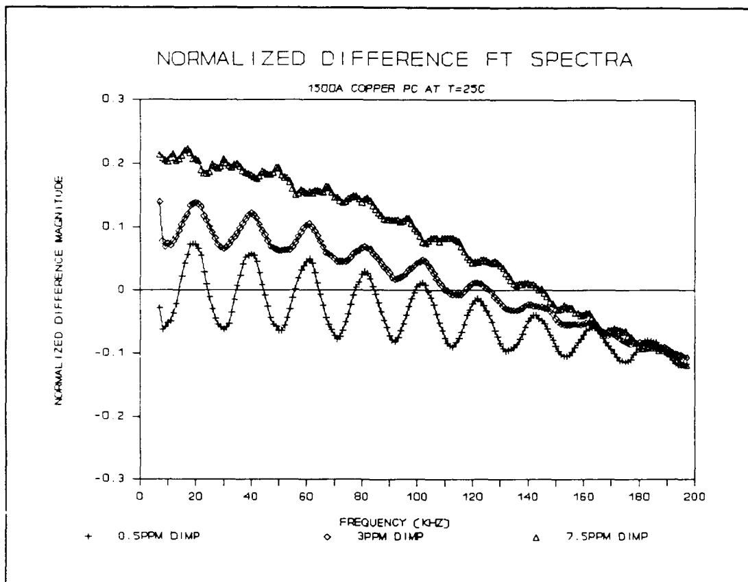
Figure V.25. Normalized Difference Fourier Transform Spectra of the CHEMFET Sensor Coated with the 1500Å Thick CuPc upon Exposure to the DIMP Challenge at 25 °C.
