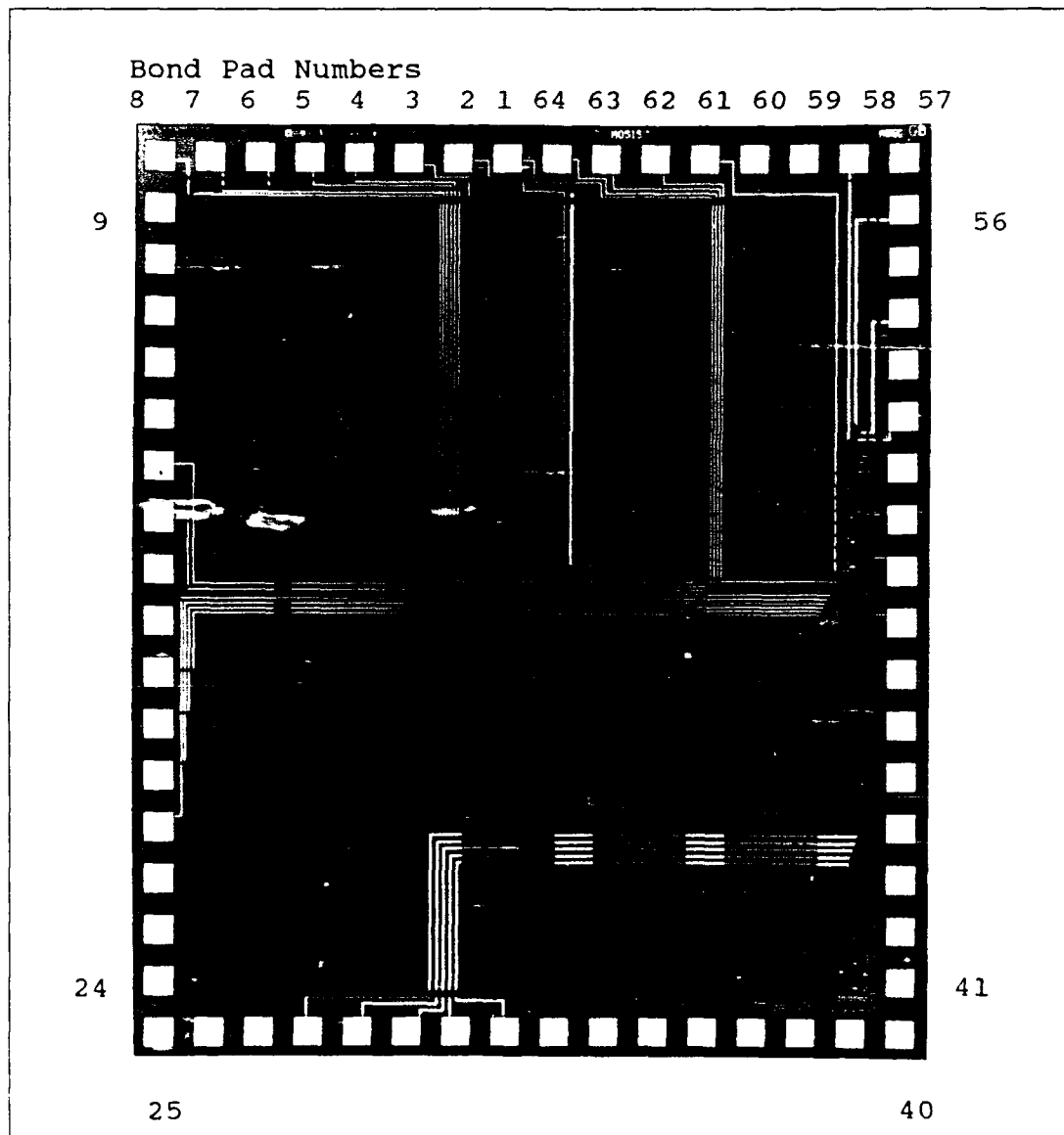
Figure III.6. Photomicrograph of the CHEMFET IC.
