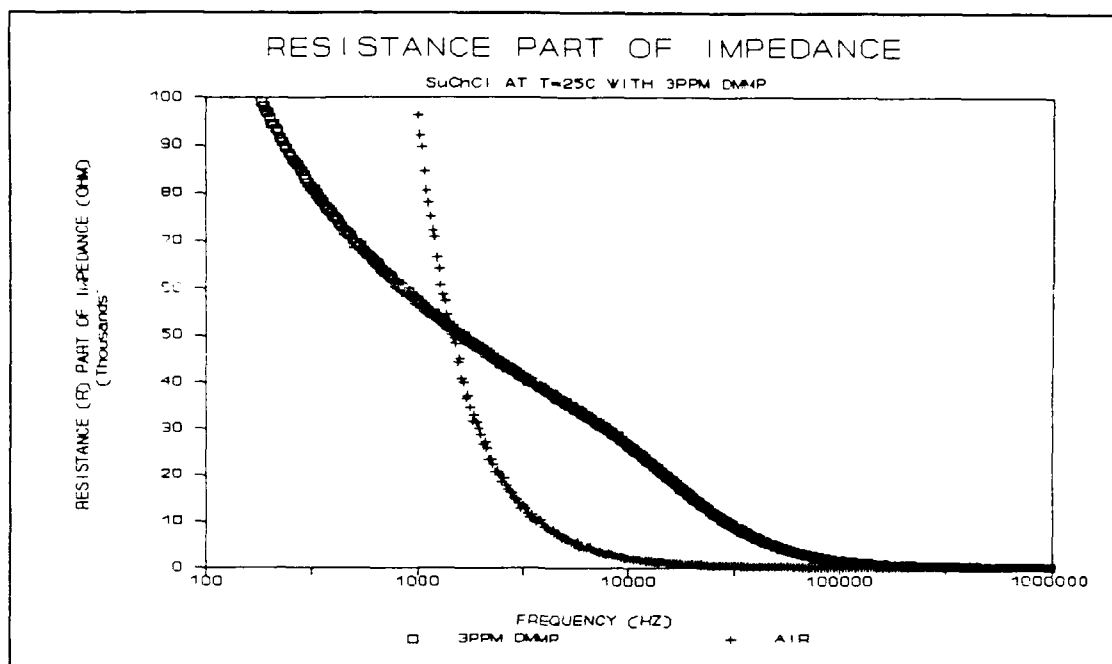
Figure F.15. Resistive Part of the Impedance for the Succinylcholine Chloride Film upon Exposure to the 3 ppm DMMP Challenge at 25 °C.
