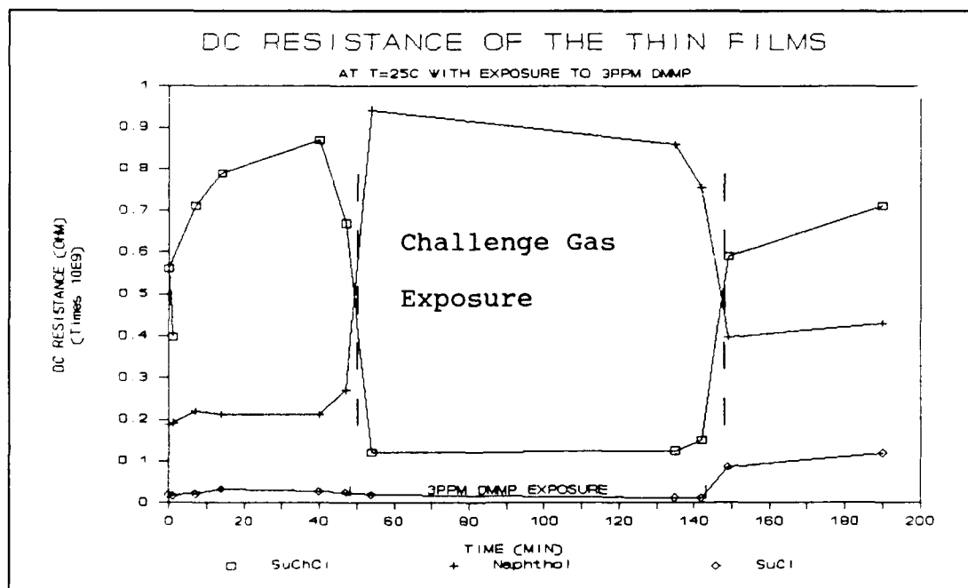
Figure V.34. DC Resistance of the Organic Thin Films, Succinylcholine Chloride, 2-Naphthol( \beta ), and Succinylchloride upon Exposure to the 3 ppm DMMP Challenge at 25°C.
