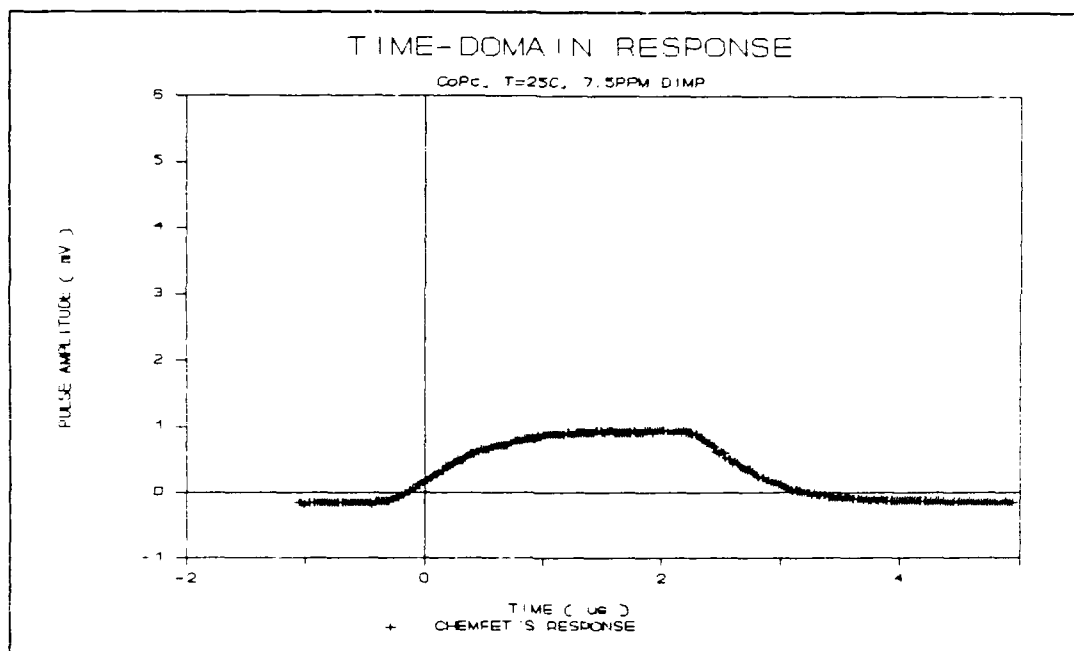
Figure V.4. Time-Domain Response of the CHEMFET Sensor Coated with a 1500Å Thick CoPc Film upon Exposure to a 7.5 ppm DIMP Challenge at 25 °C.
