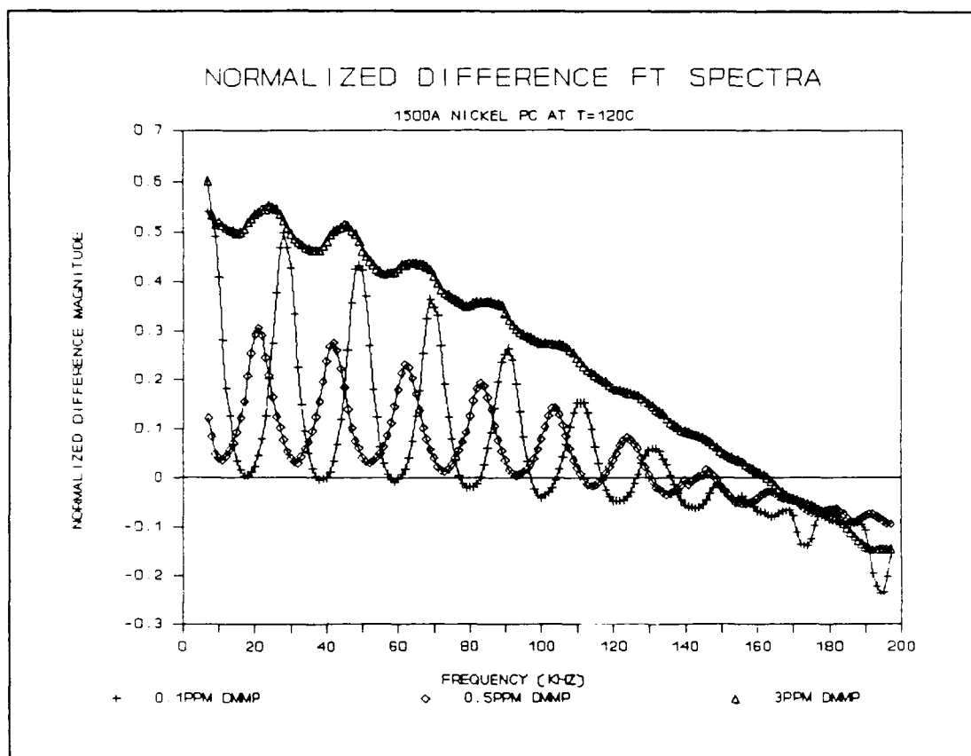
Figure V.17. Normalized Difference Fourier Transform Spectra of the CHEMFET Sensor Coated with the 1500Å Thick NiPc Film upon Exposure to the DMMP Challenge at 120 °C.
