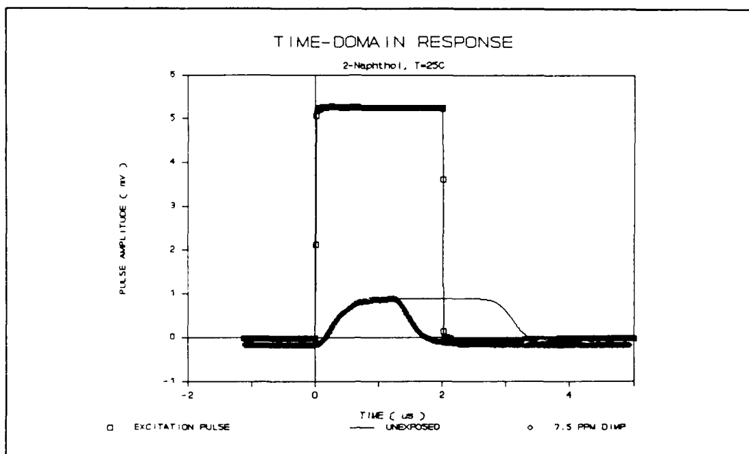
Figure V.32. Time-Domain Response of the CHEMFET Sensor Coated with the 2-Naphthol( \beta ) upon Exposure to the 7.5 ppm DIMP Challenge at 25 °C.
