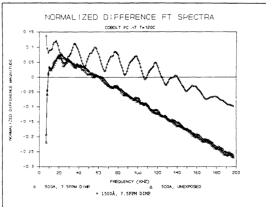
Figure V.9. Normalized Difference Fourier Transform Spectra of the CHEMFET Sensors Coated with the 500Å and 1500Å Thick CoPc Films upon Exposure to the 7.5 ppm DIMP Challenge at 120 °C.
