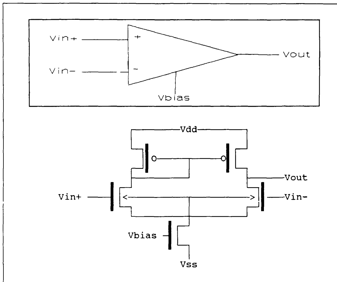
Figure III.3. Differential Input Comparator (20:330).
