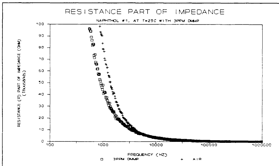
Figure F.3. Resistive Part of the Impedance for the 2-Naphthol( \beta ) Film upon Exposure to the 3 ppm DMMP Challenge at 25°C.
