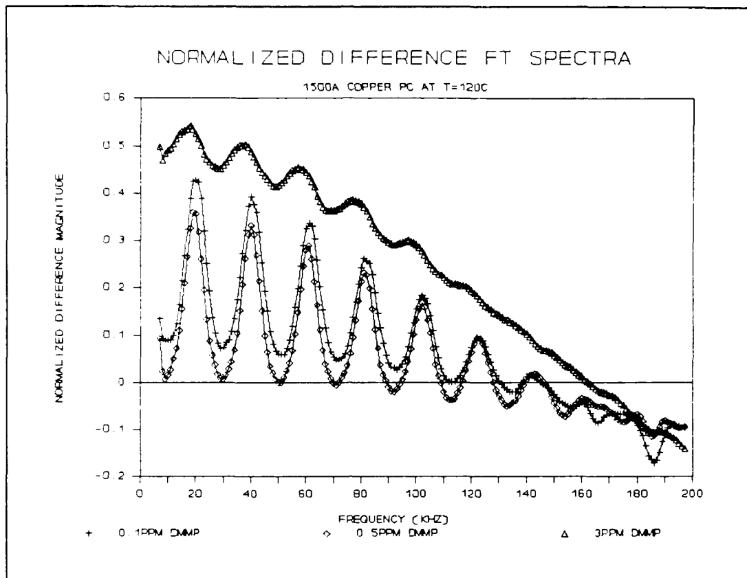
Figure V.29. Normalized Difference Fourier Transform Spectra of the CHEMFET Sensor Coated with the 1500Å Thick CuPc Film upon Exposure to DMMP Challenge at 120 °C.
