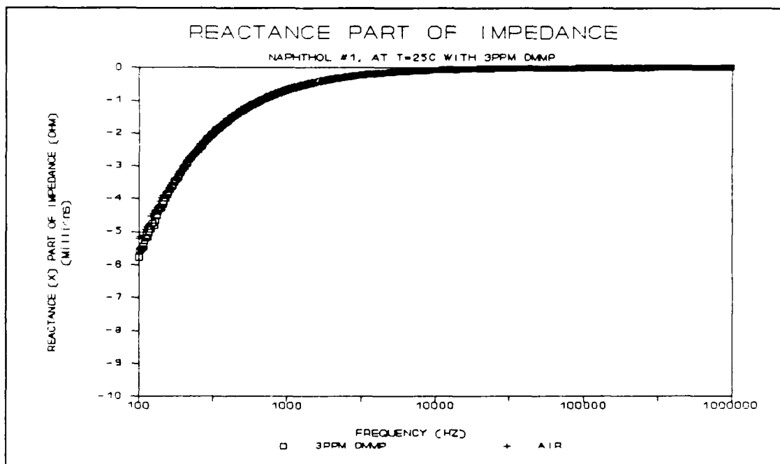
Figure F.4. Reactive Part of the Impedance for the 2-Naphthol( \beta ) Film upon Exposure to the 3 ppm DMMP Challenge at 25°C.
