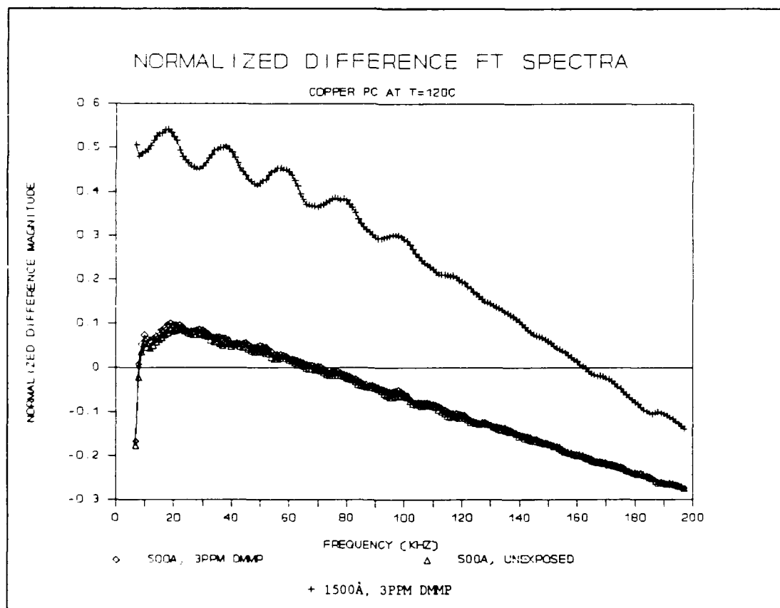
Figure V.30. Normalized Difference Fourier Transform Spectra of the CHEMFET Sensors Coated with the 500Å and 1500Å Thick CuPc Films upon Exposure to the 3 ppm DMMP Challenge at 120 °C.
