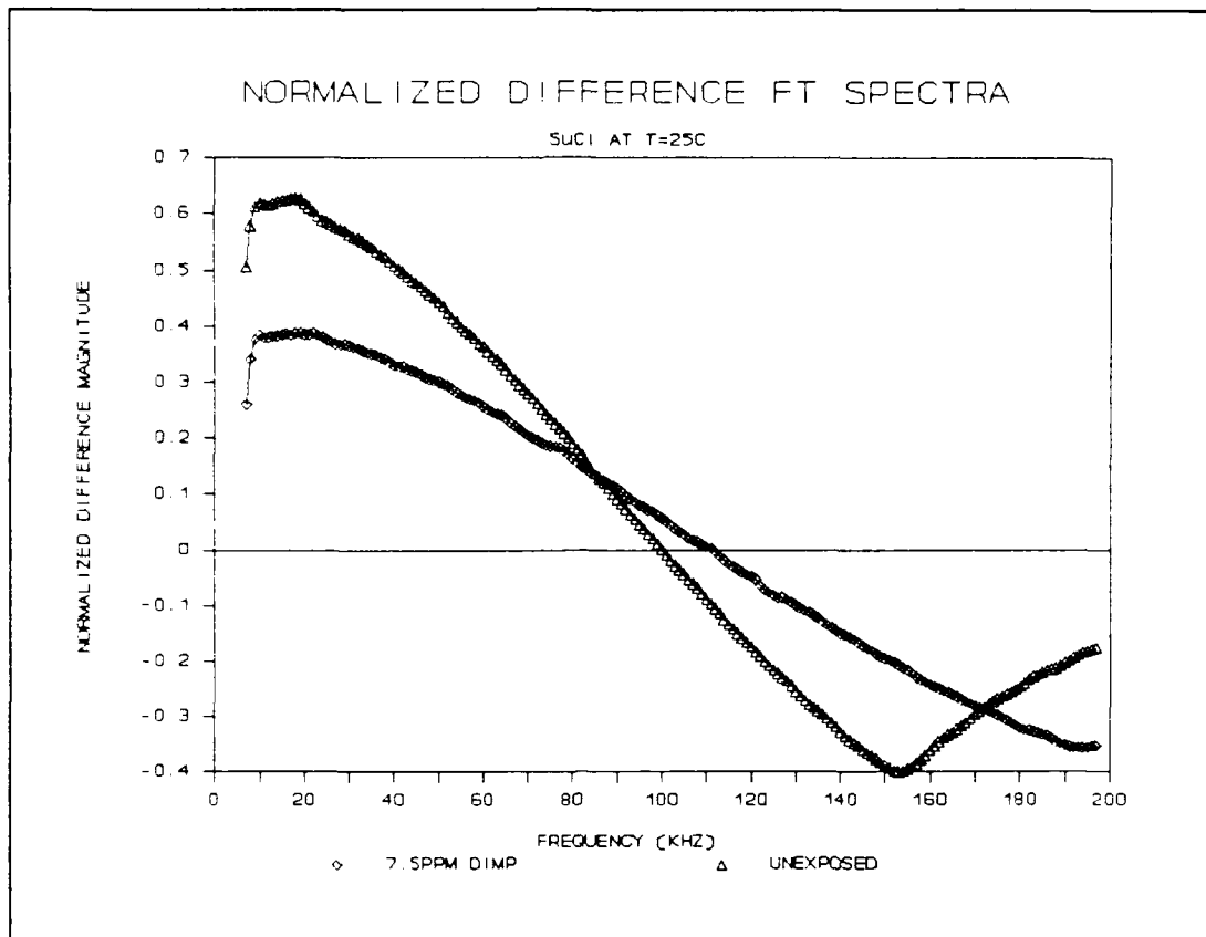
Figure V.35. Normalized Difference Fourier Transform Spectra of the CHEMFET Sensor Coated with the Succinylchloride Film upon Exposure to the 7.5 ppm DIMP Challenge at 25 °C.
