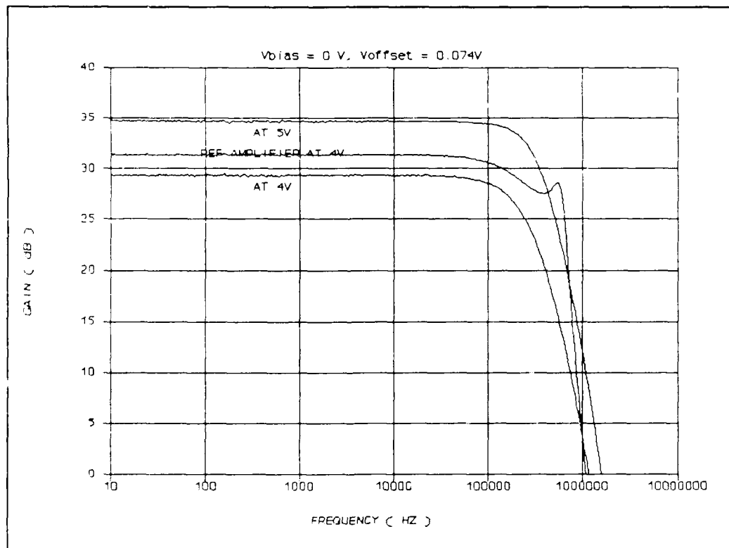
Figure III.9. Gain of the Interdigitated Gate Electrode CHEMFET's Amplifier versus Frequency.
