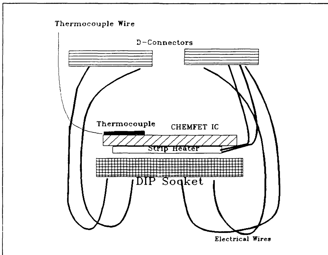
Figure D.8. Schematic Drawing of the DIP Socket.
