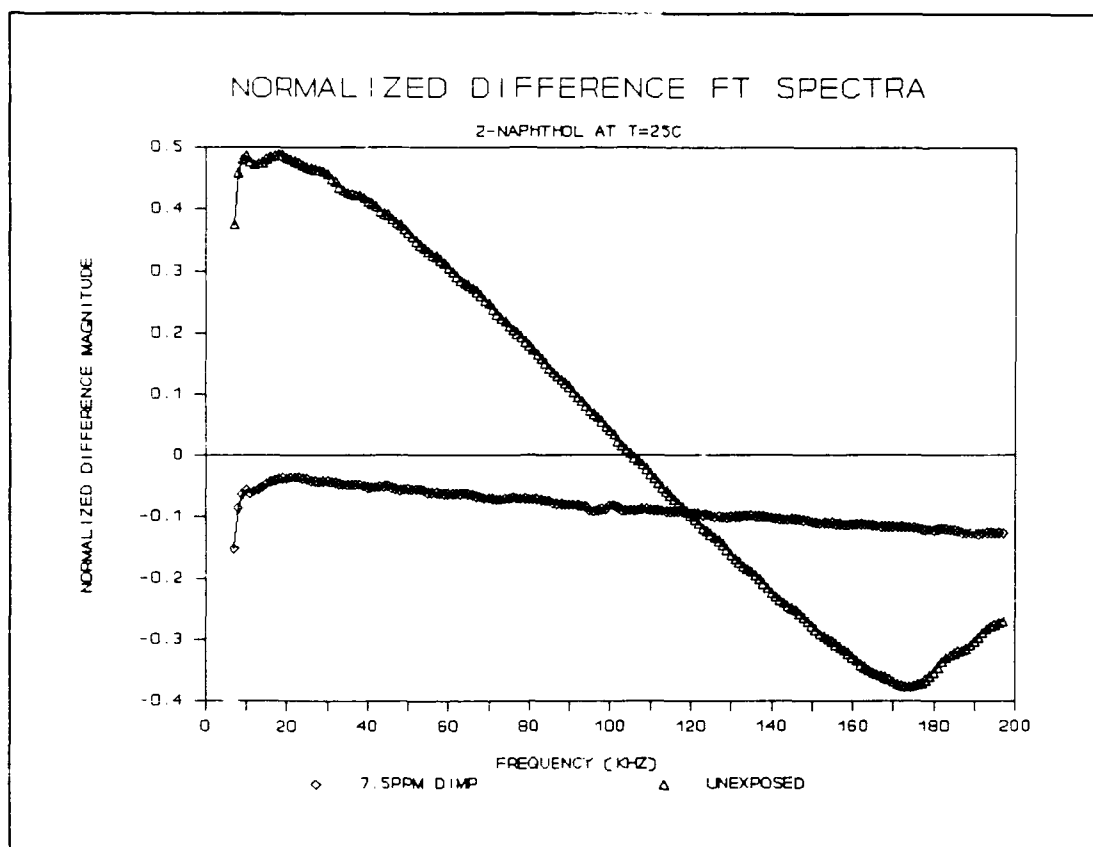
Figure V.31. Normalized Difference Fourier Transform Spectra of the CHEMFET Sensor Coated with the 2-Naphthol( \beta ) upon Exposure to the 7.5 ppm DIMP Challenge at 25 °C.
