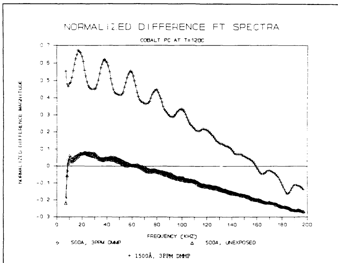
Figure V.12. Normalized Difference Fourier Transform Spectra of the CHEMFET Sensors Coated with the 500Å and 1500Å Thick CoPc Films upon Exposure to the 3 ppm DMMP Challenge at 120 °C.
