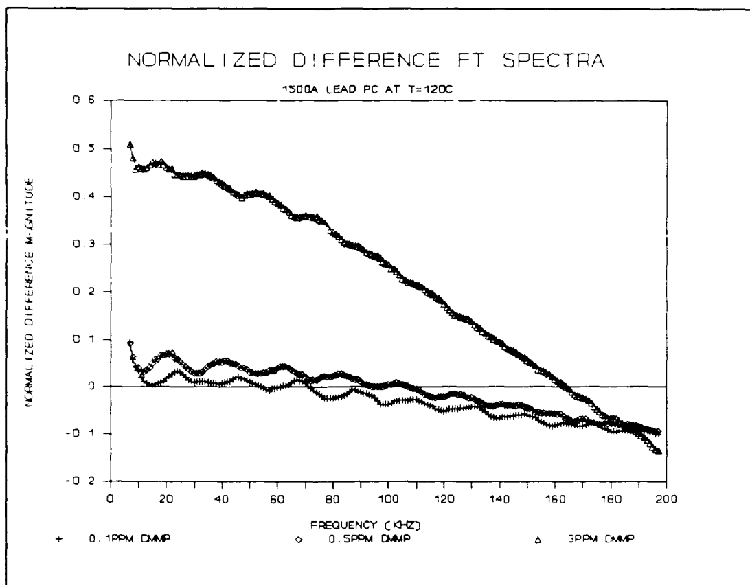
Figure V.23. Normalized Difference Fourier Transform Spectra of the CHEMFET Sensor Coated with the 1500Å Thick PbPc Film upon Exposure to the DMMP Challenge at 120 °C.
