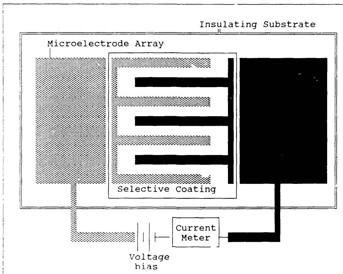
Figure II.2. Schematic of a Chemiresistor Structure (7:1170).
