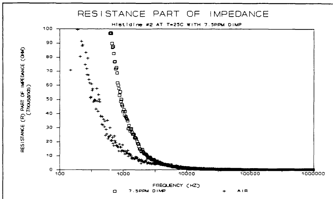
Figure F.9. Resistive Part of the Impedance for the L-Histidine Dihydrochloride Film upon Exposure to the 7.5 ppm DIMP Challenge at 25 °C.
