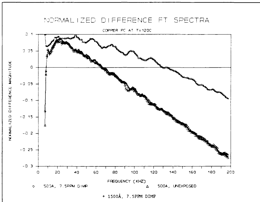
Figure V.27. Normalized Difference Fourier Transform Spectra of the CHEMFET Sensors Coated with the 500Å and 1500Å Thick CuPc Films upon Exposure to the 7.5 ppm DIMP Challenge at 120 °C.
