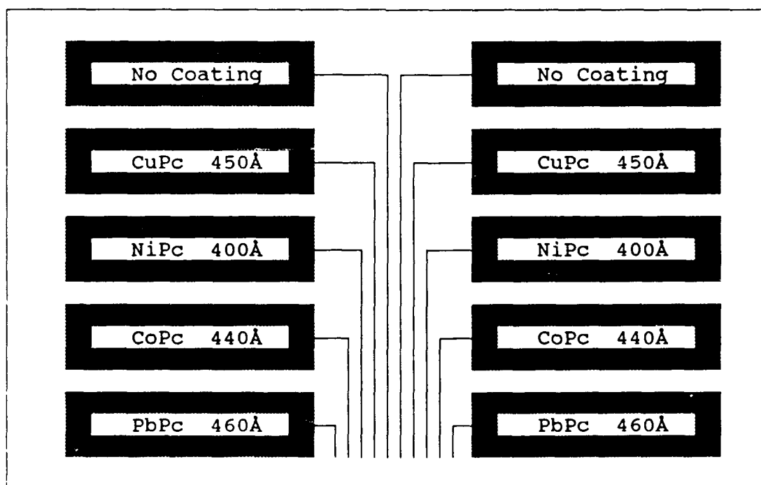
Figure IV.2. CHEMFET 2: 500Å Thick Phthalocyanine Films.
