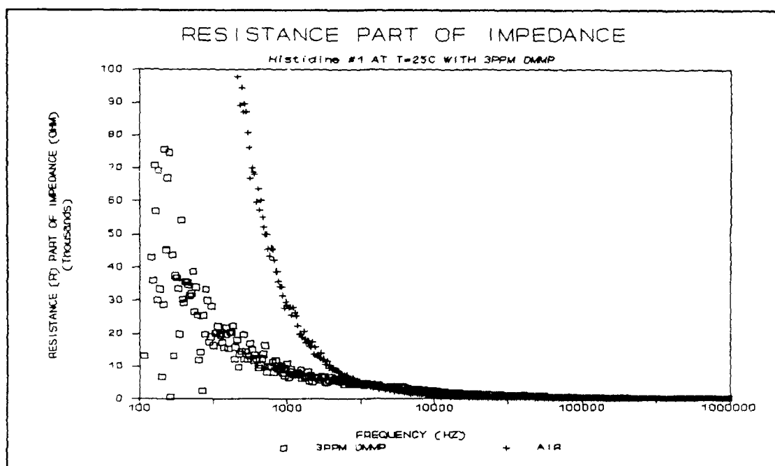
Figure F.11. Resistive Part of the Impedance for the L-Histidine Dihydrochloride Film upon Exposure to the 3 ppm DMMP Challenge at 25 °C.
