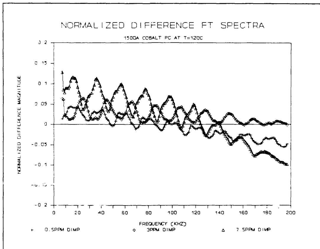
Figure V.8. Normalized Difference Fourier Transform Spectra of the CHEMFET Sensor Coated with the 1500Å Thick CoPc upon Exposure to DIMP at 120 °C.
