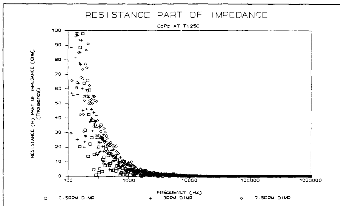
Figure V.5. Resistive Part of the Impedance of the 1500Å Thick CoPc Film upon Exposure to the DIMP at 25 °C.
