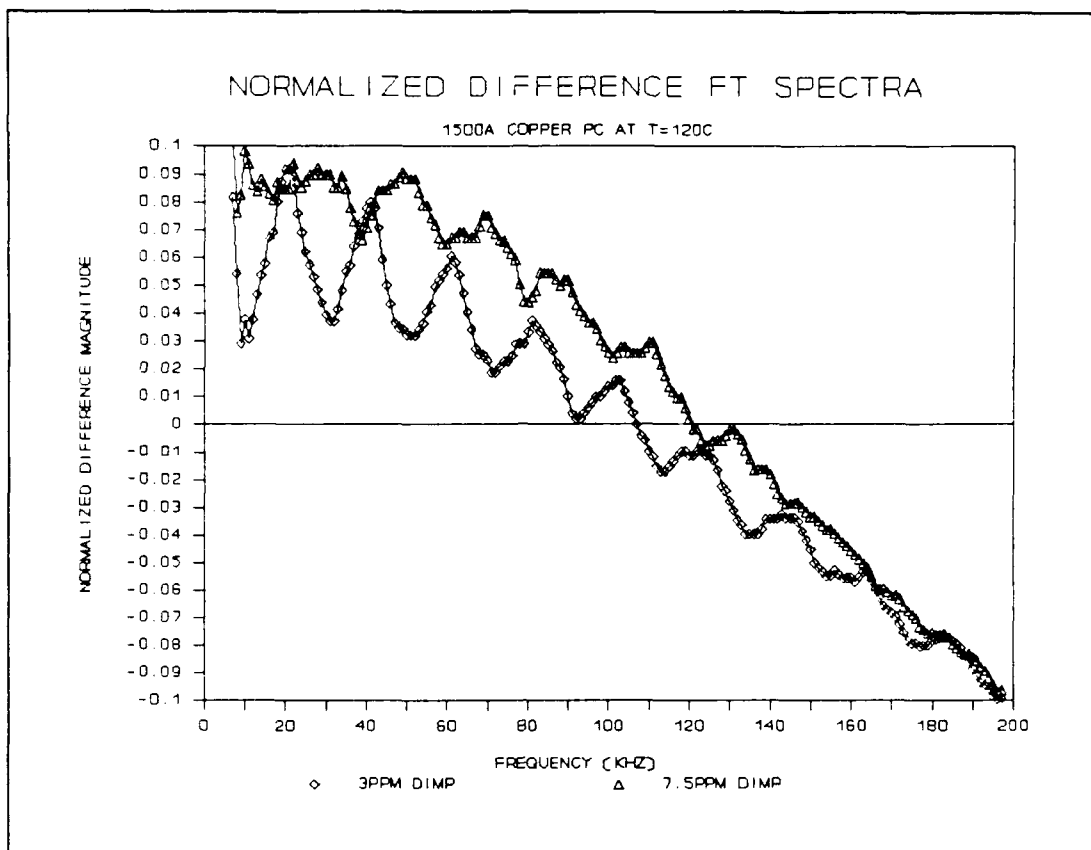
Figure V.26. Normalized Difference Fourier Transform Spectra of the CHEMFET Sensor Coated with the 1500Å Thick CuPc upon Exposure to the DIMP Challenge at 120 °C.
