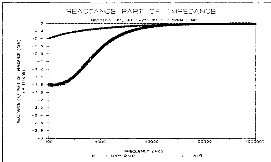
Figure F.2. Reactive Part of the Impedance for the 2-Naphthol( \beta ) Film upon Exposure to the 7.5 ppm DIMP Challenge at 25°C.
