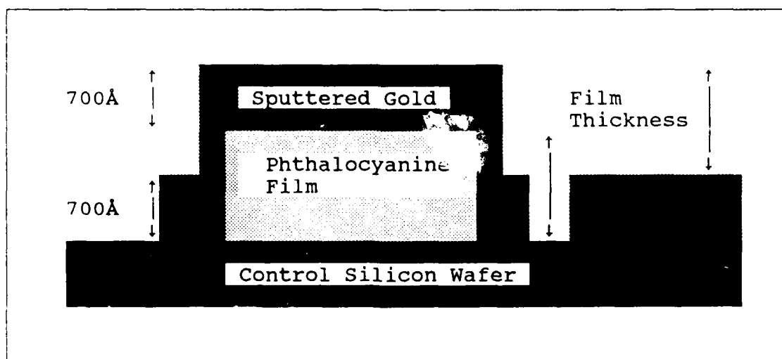
Figure C.4. Thin Gold Film Sputtered onto a Phthalocyanine Film.
