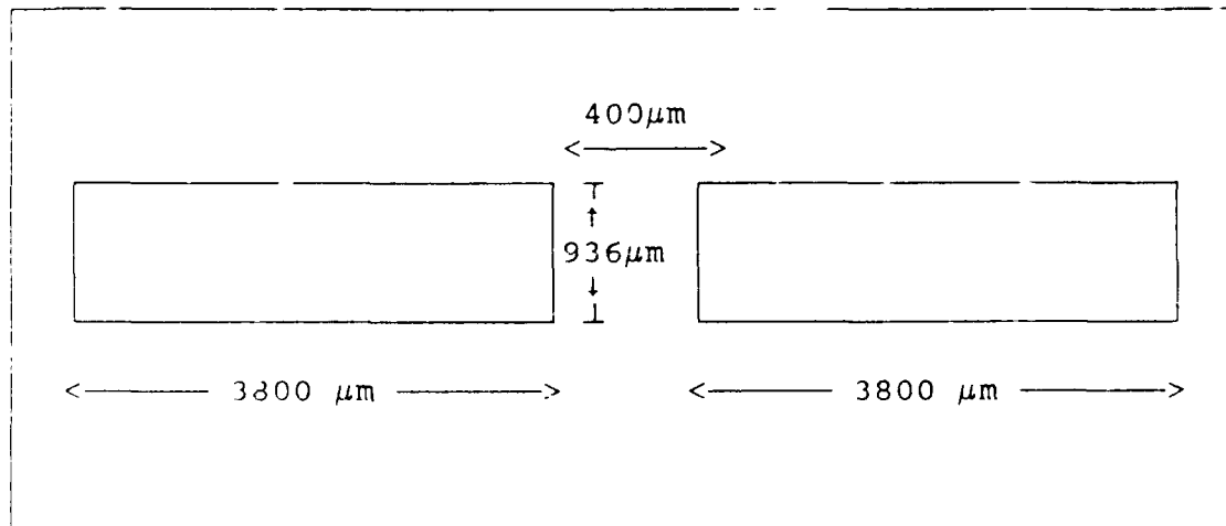
Figure C.1. Evaporation Mask Pattern.
