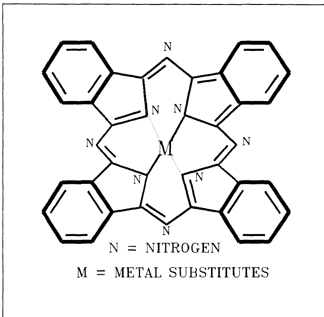
Figure II.3. Chemical Structure of a Metal-Doped Phthalocyanine (14:374).
