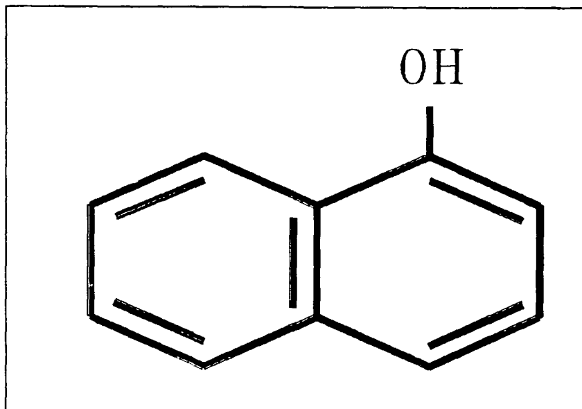
Figure II.4. Chemical Structure of 2-Naphthol( \beta ) (14:924).
