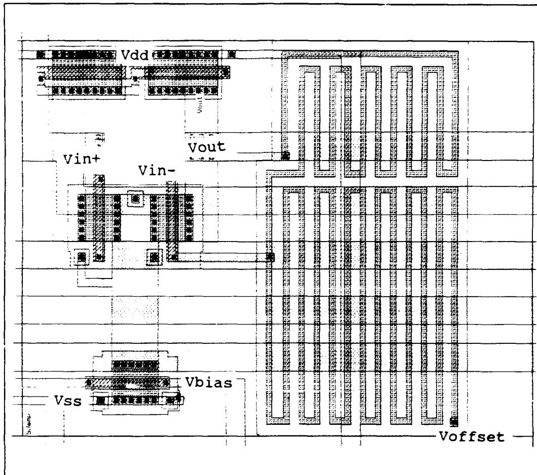
Figure III.5. CIF plot of the First Amplifier Stage.
