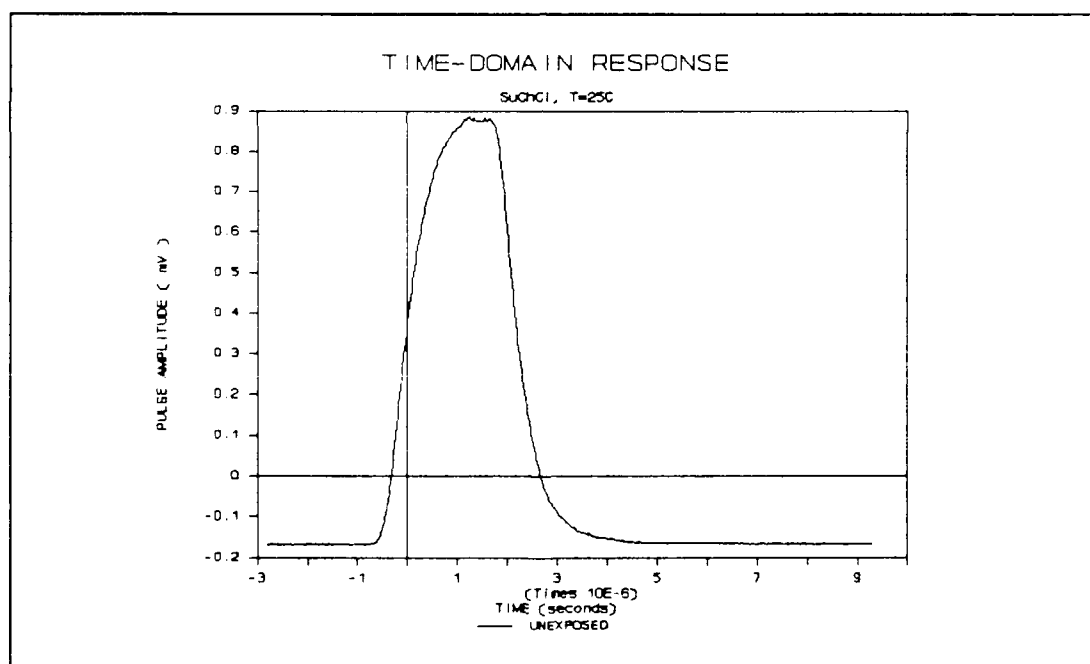
Figure V.44. Time-Domain Response of the CHEMFET Sensor Coated with the Succinylcholine Chloride Film upon Exposure to Air at 25 °C.
