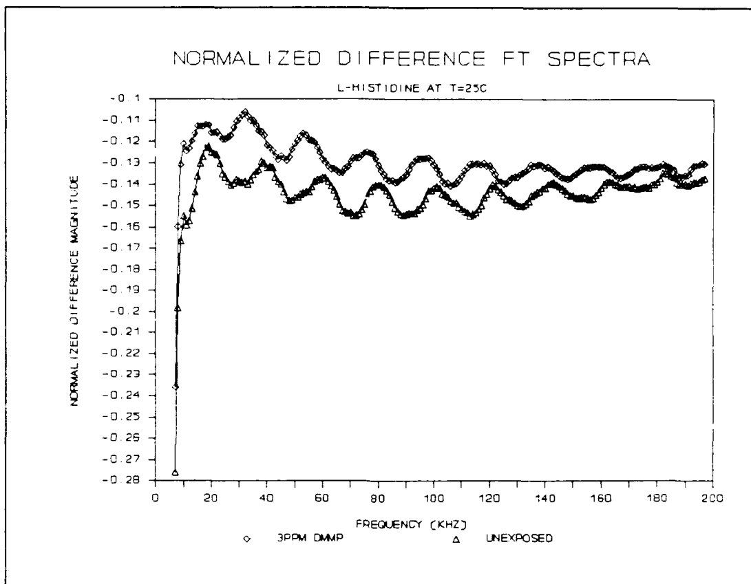
Figure V.40. Normalized Difference Fourier Transform Spectra of the CHEMFET Sensor Coated with the L-Histidine Dihydrochloride Film upon Exposure to the 3 ppm DMMP Challenge at 25 °C.
