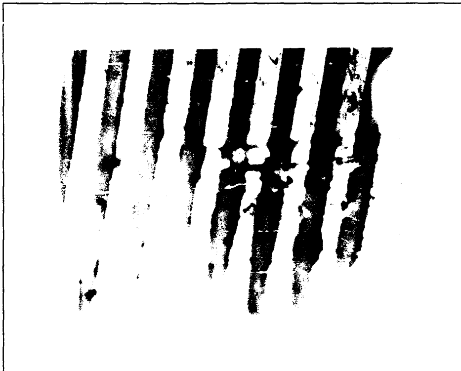
Figure III.7. Example of a Shorted Interdigitated Gate Electrode.
