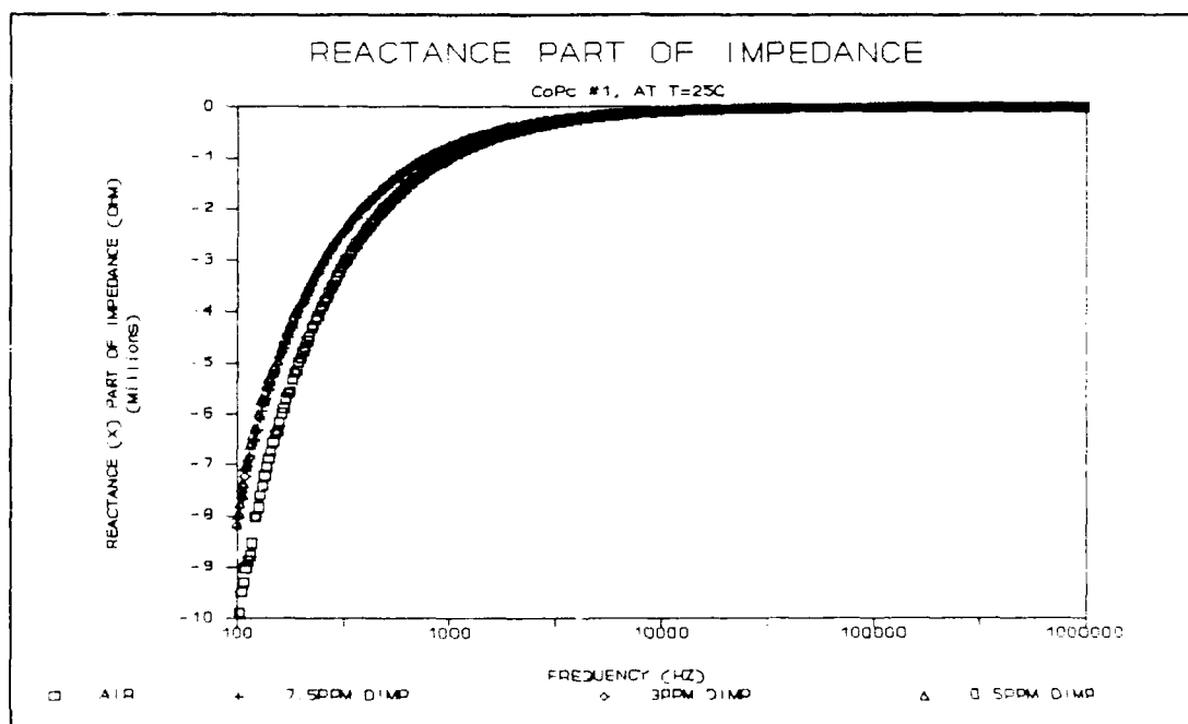
Figure V.6. Reactive Part of the Impedance of the 1500Å Thick CoPc Film upon Exposure to the DIMP at 25 °C.
