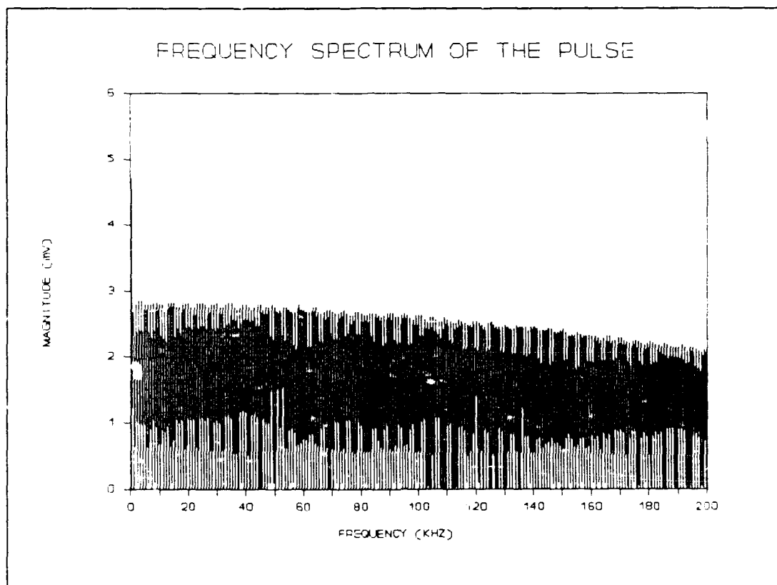
Figure IV.6. Frequency Spectrum of the Excitation Pulse.
