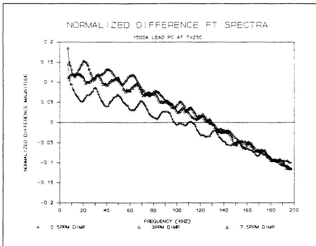
Figure V.19. Normalized Difference Fourier Transform Spectra of the CHEMFET Sensor Coated with the 1500Å Thick PbPc Film upon Exposure to the DIMP Challenge at 25 °C.
