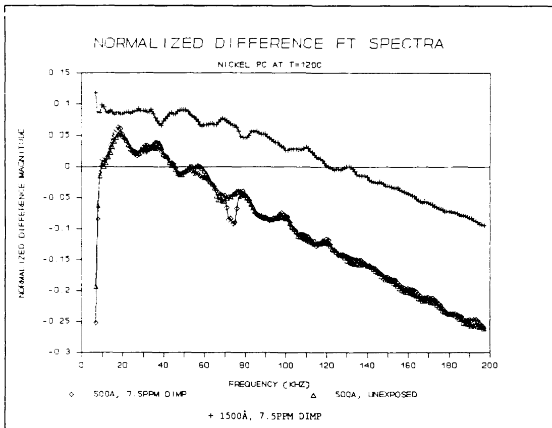
Figure V.15. Normalized Difference Fourier Transform Spectra of the CHEMFET Sensors Coated with the 500Å and 1500Å Thick NiPc Films upon Exposure to the 7.5 ppm DIMP Challenge at 120 °C.
