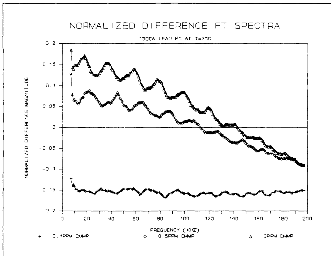
Figure V.22. Normalized Difference Fourier Transform Spectra of the CHEMFET Sensor Coated with the 1500Å Thick PbPc Film upon Exposure to the DMMP Challenge at 25 °C.
