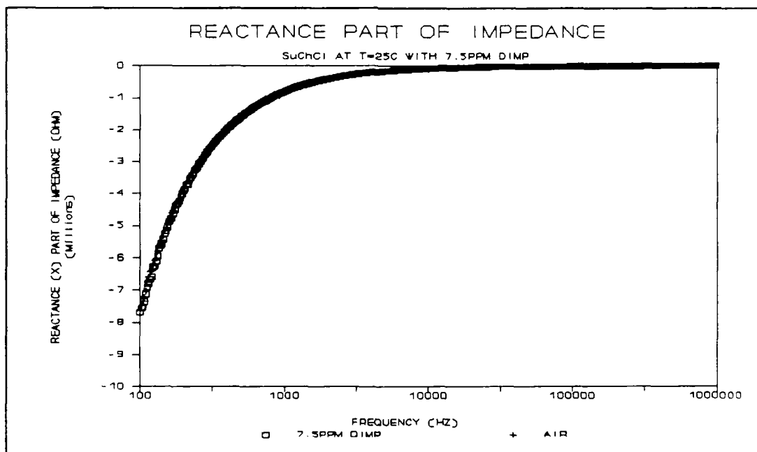
Figure F.14. Reactive Part of the Impedance for the Succinylcholine Chloride Film upon Exposure to the 7.5 ppm DIMP Challenge at 25 °C.
