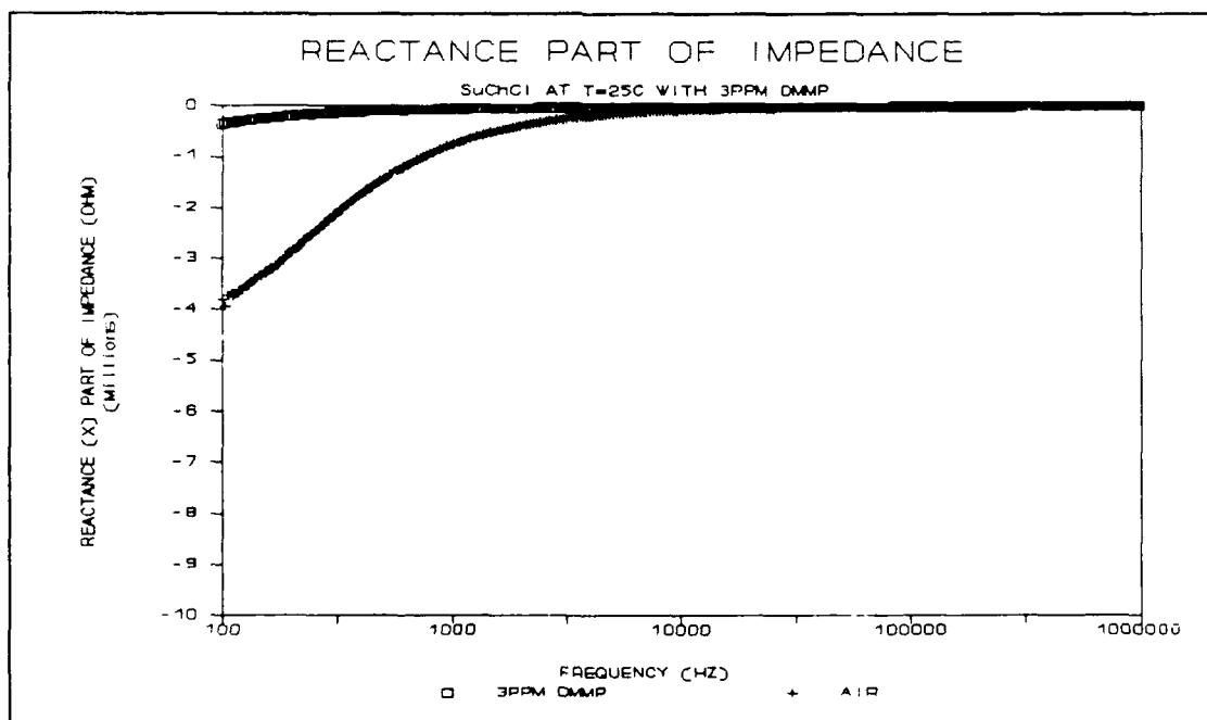
Figure F.16. Reactive Part of the Impedance for the Succinylcholine Chloride Film upon Exposure to the 3 ppm DMMP Challenge at 25 °C.
