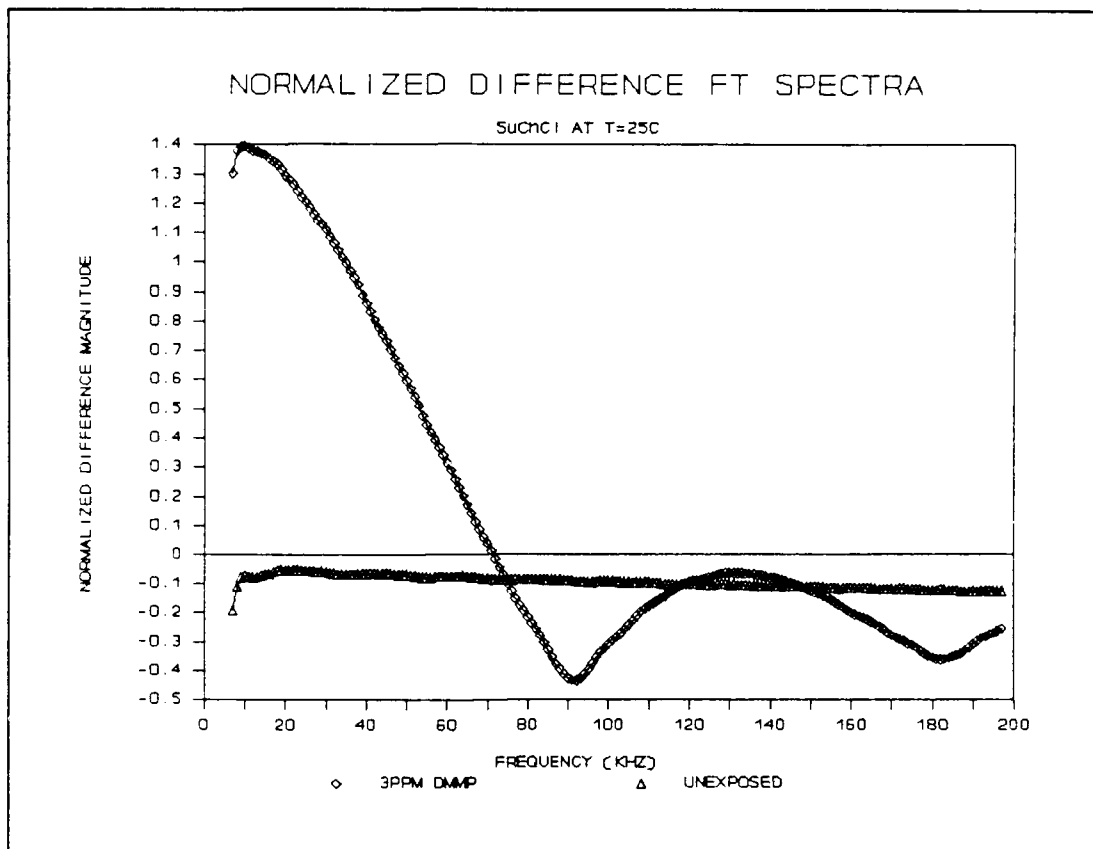
Figure V.43. Normalized Difference Fourier Transform Spectra of the CHEMFET Sensor Coated with the Succinylcholine Chloride Film upon Exposure to the 3 ppm DMMP Challenge at 25 °C.
