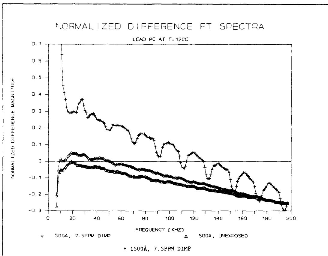
Figure V.21. Normalized Difference Fourier Transform Spectra of the CHEMFET Sensors Coated with the 500Å and 1500Å Thick PbPc Films upon Exposure to the 7.5 ppm DIMP Challenge at 120 °C.
