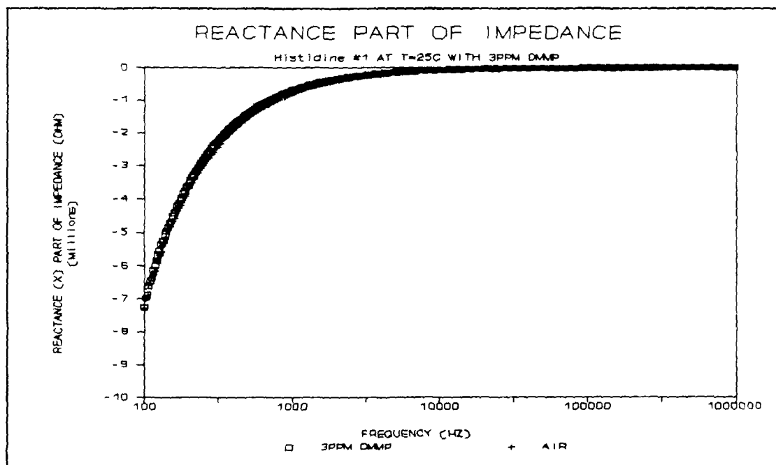
Figure F.12. Reactive Part of the Impedance for the L-Histidine Dihydrochloride Film upon Exposure to the 3 ppm DMMP Challenge at 25 °C.
