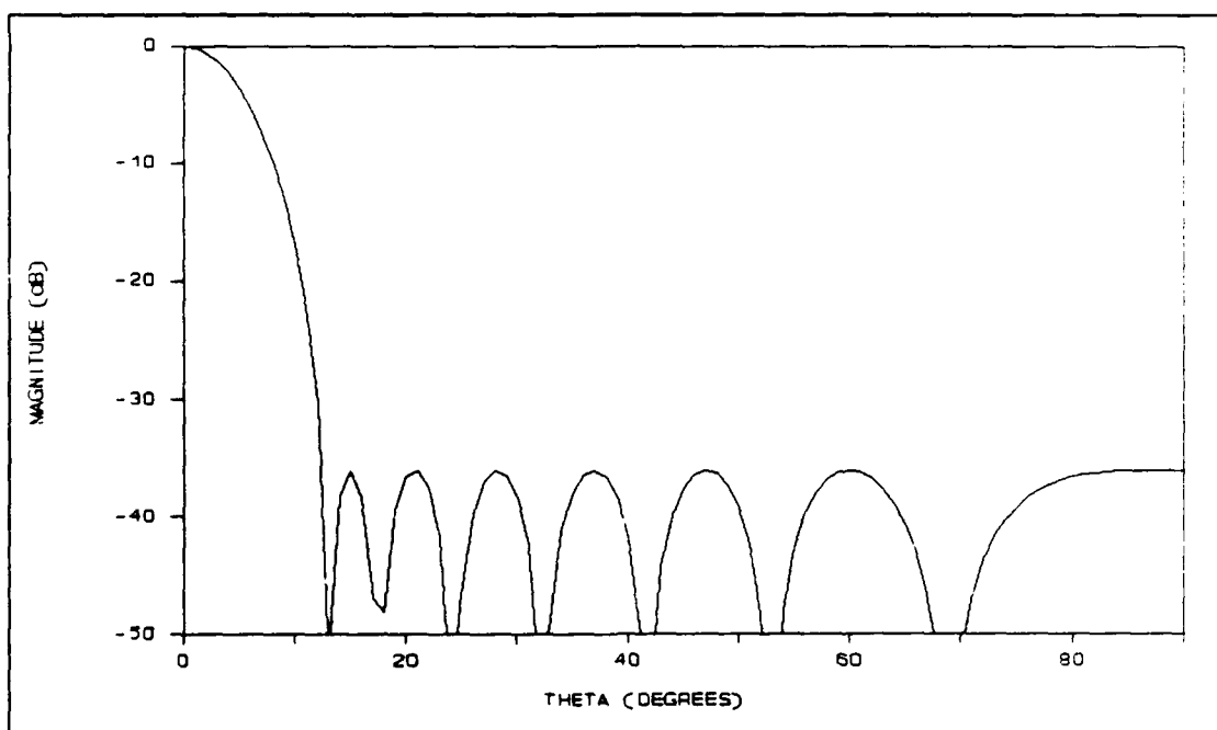
Figure 20. Radiation pattern for a 15 element, Dolph-Chebyshev synthesized array with \frac{1}{2} \lambda interelement spacing showing a -36 dB side lobe level
