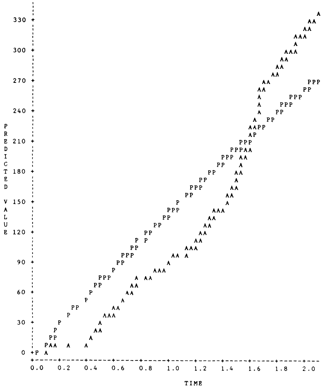
Figure 12: Model versus Actual for AFOTEC Model (Data Set #1)
