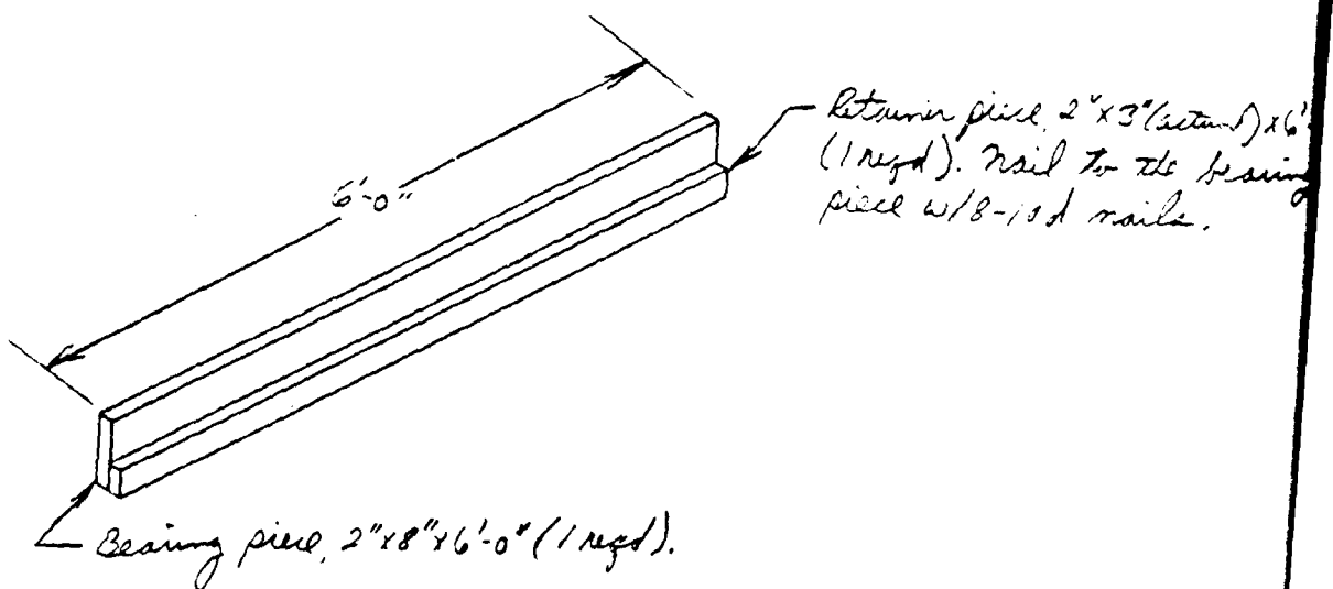
LOWER SIDE FILL ASSEMBLY
