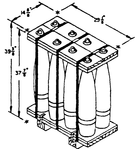
155MM, 8/PALLET (PALLET UNIT 2)
