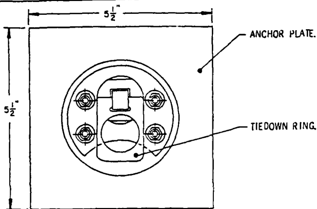
UNIVERSAL TIEDOWN ANCHOR (FRONT VIEW)
