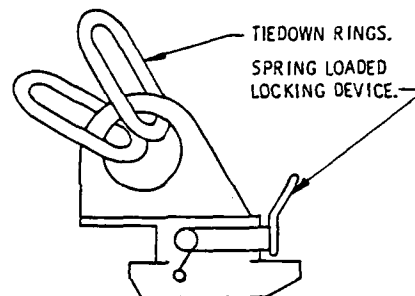
TYPE II. REMOVABLE TIEDOWN ANCHOR (SIDE VIEW)
