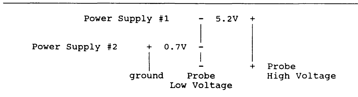
Figure 2.1: Probe Voltage Biasing Scheme.
