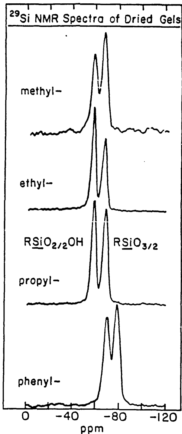
Figure 7. 29 Si NMR spectra of the dry gels prepared with methyl-, ethyl-, propyl- and phenyl-trimethoxysilane; in all cases, one line is due to \text{R SiO}_{3/2} and the other \text{R Si(O}_{2/2}\text{)OH} (where R = methyl, ethyl, propyl or phenyl).
