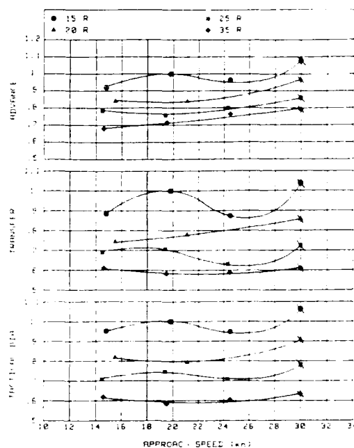
Fig. 21. Tactical Curves, USS NEW JERSEY (BB 62)
