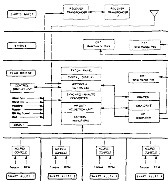
Fig. 14. Instrumentation block diagram, USS IOWA (BB 61).
