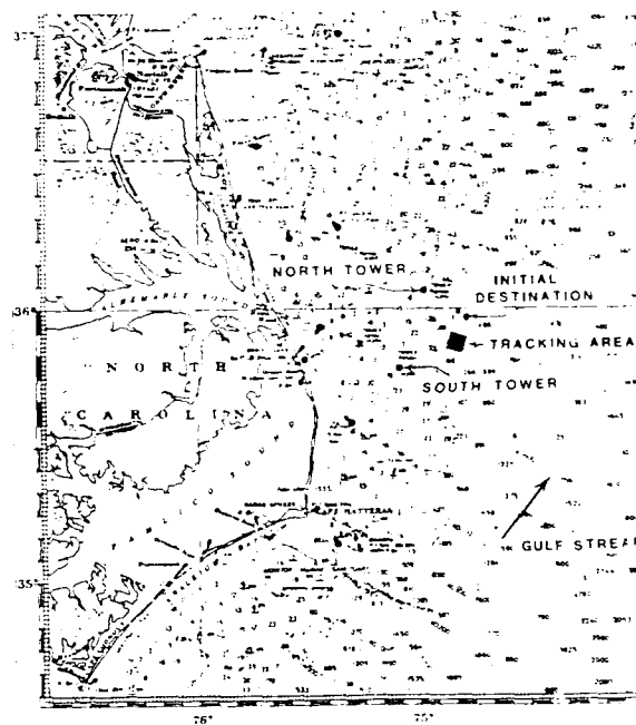
Fig. 7. Hatteras East Coast Offshore Range (HECTOR).
