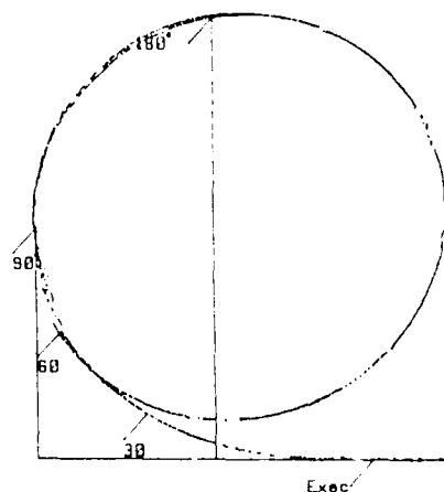
Fig. 24. Tactical plot, USS IOWA (BB 61).
