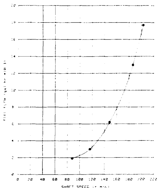
Fig. 22. Fuel Economy Curves, USS NEW JERSEY (BB 62).
