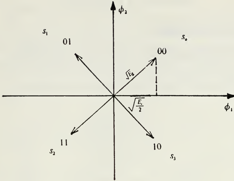
Figure 3. QPSK Signal Constellation Diagram
