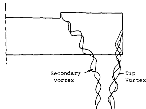
Figure 3. Vortex Interaction.
