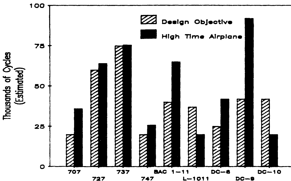
Figure 2. Landing cycles for selected active air carrier aircraft. (FAA, 1988; Boeing Commercial Airplanes, 1989)
