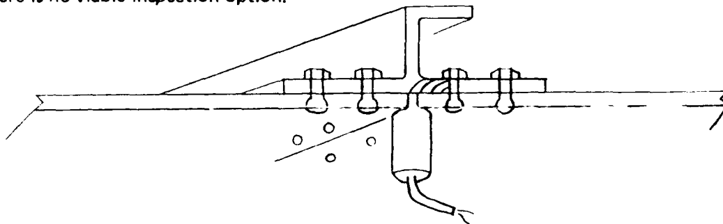
Figure 1. Example of low frequency eddy current inspection of lower wing surface span-wise splice stringer.
