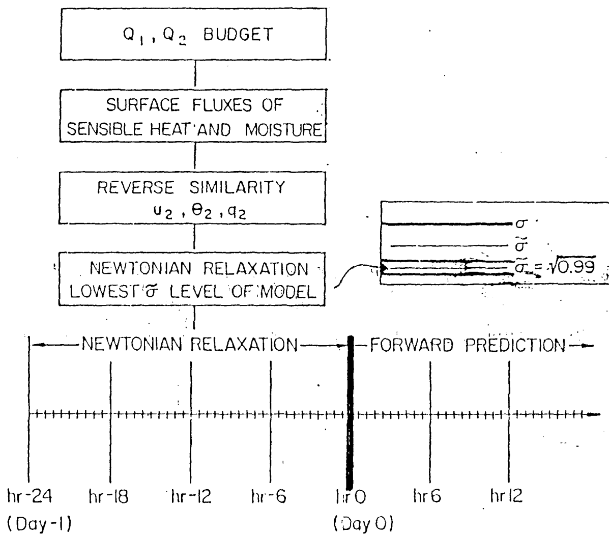
Figure 7c: Schematic outline of the implicit handling of surface fluxes of sensible heat and moisture. Here a reverse similarity algorithm is involved during each time-step of the Newtonian relaxation phase to give \tilde{V} , \theta , q at the lowest sigma level of the model. A Newtonian relaxation is then performed using these values.
