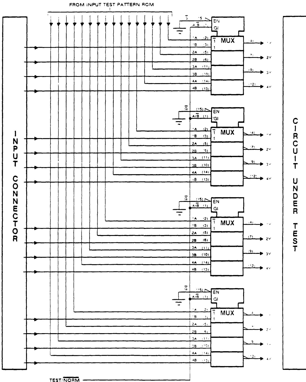
FIGURE 6 INPUT MULTIPLEXER
