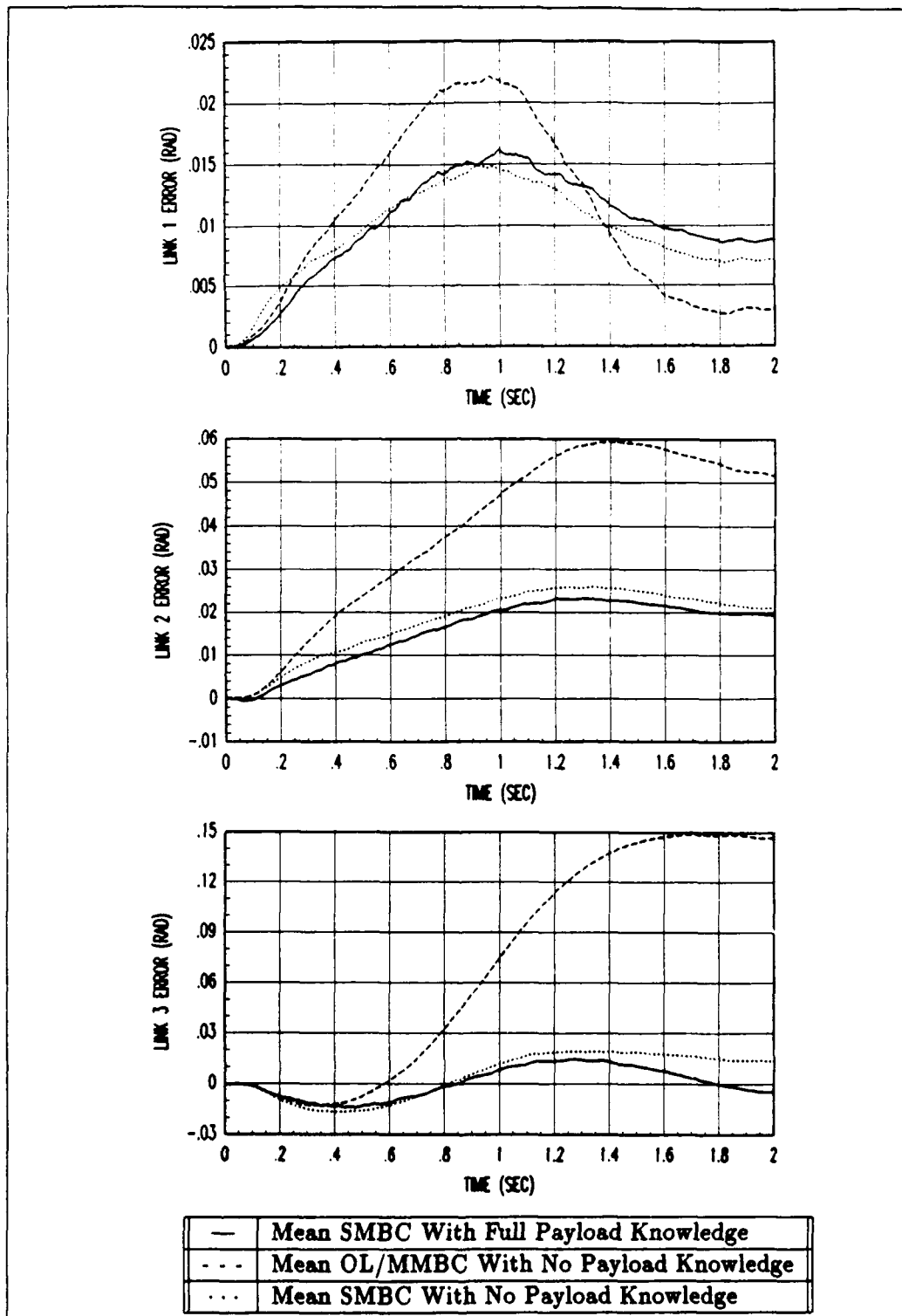
Figure D.2. Payload 3.0 Kg: Tracking Errors for Trajectory One Using Soft Gains
