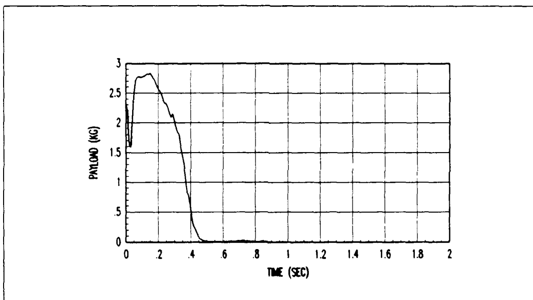
Figure D.12. Payload 0.0 Kg: Mean MMAE Payload Estimate Using Soft Gains
