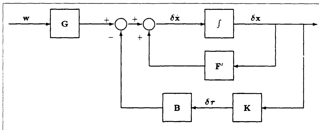
Figure 3.2. Rearranged Block Diagram of Linear Perturbation Model
