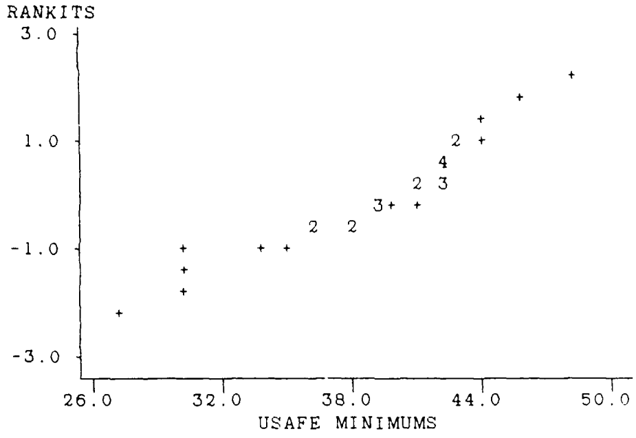
APPROX. WILK-SHAPIRO 0.9183 30 CASES PLOTTED
