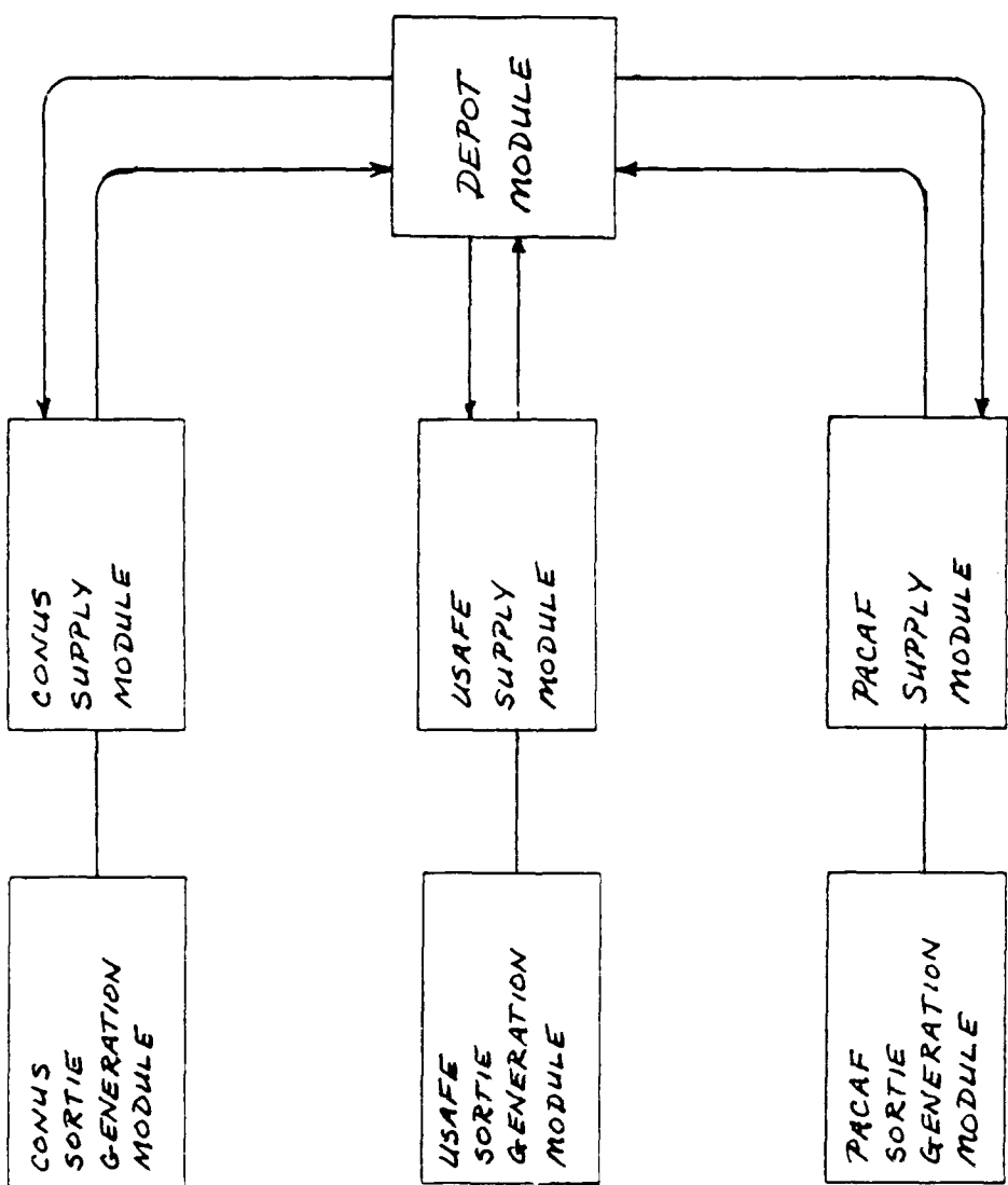
SLAM II Network Flow Diagram
