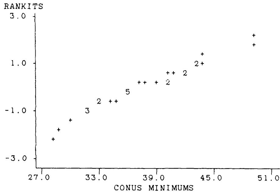
APPROX. WILK-SHAPIRO 0.9787 30 CASES PLOTTED
