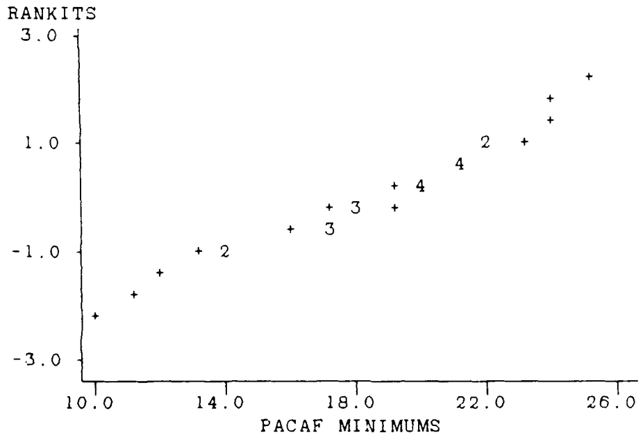
APPROX. WILK SHAPIRO 0.9685 30 CASES PLOTTED
