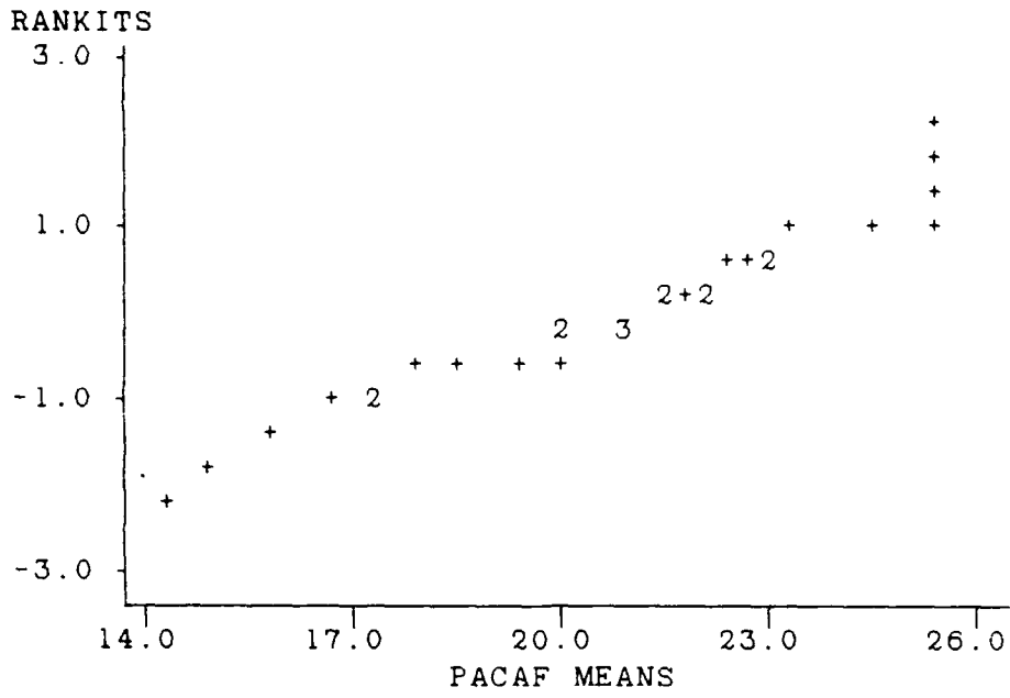
APPROX. WILK-SHAPIRO 0.9684 30 CASES PLOTTED
