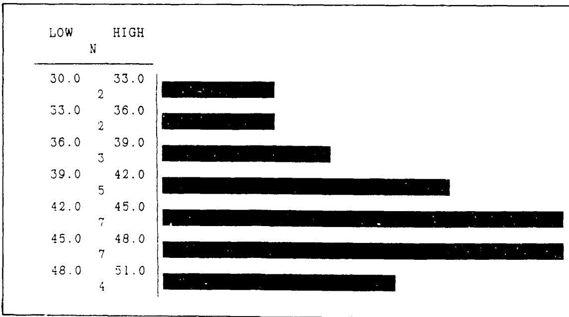
Figure 2. USAFE Average Monthly Spares Histogram
