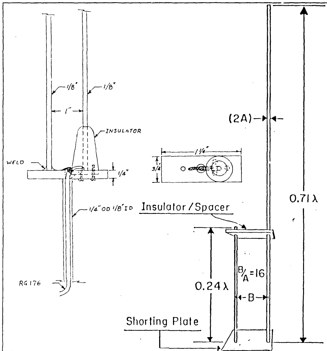
Figure 13. Construction Details for the Unbalanced Hybrid Dipole: The hybrid dipole design is from Shaw, (1973). It was designed to perform in marine and mobile applications without the requirement for a ground plane. For 143.675 MHz, \lambda = 2.08 meters. Constructed of stainless steel, with plastic insulators. Silicon sealant fills all voids to protect the exposed sections of the RG 176 coaxial cable.
