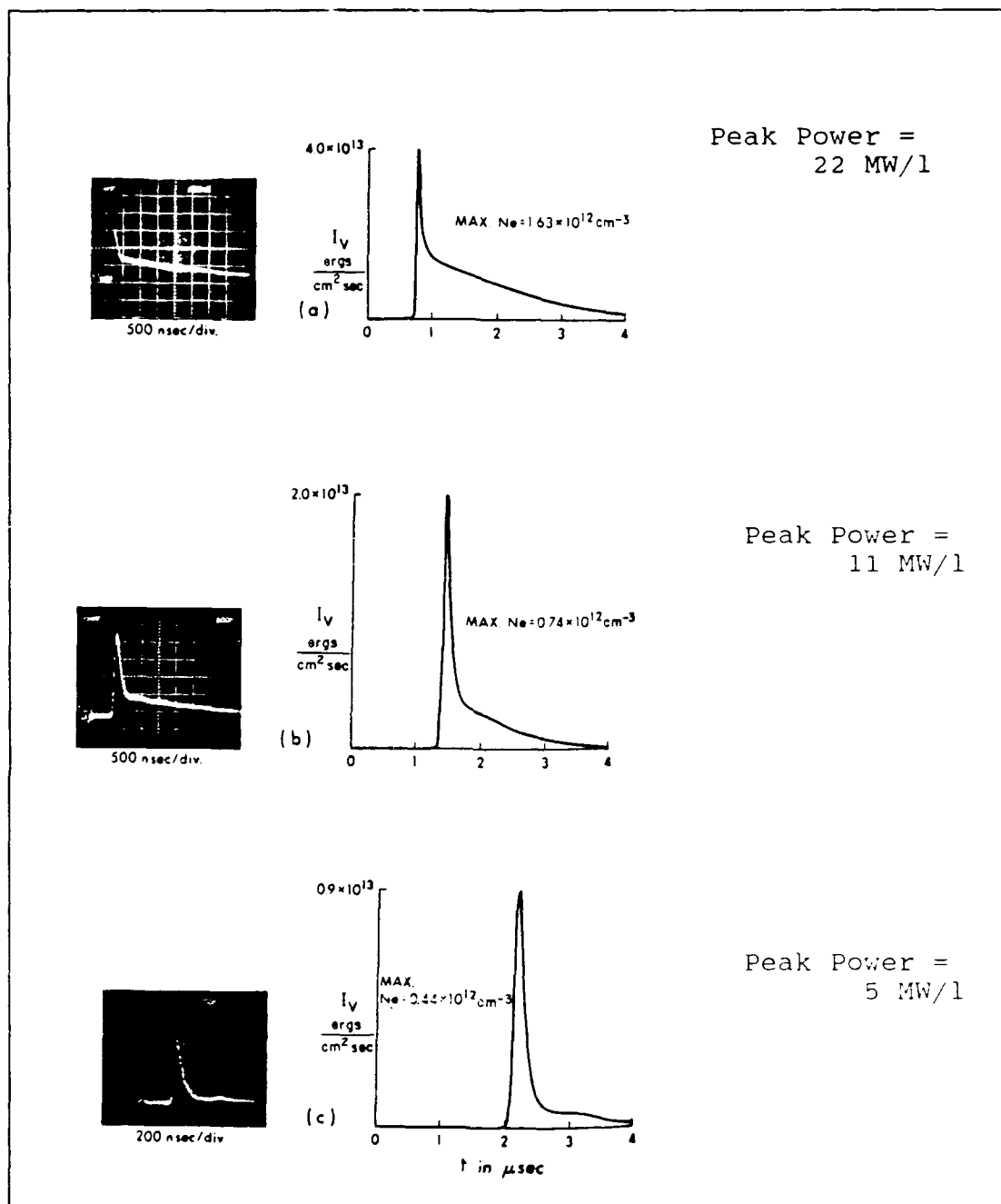
Figure 19. Pulse Shape vs Pump Energy from Manes' Study. Length = 2.5 m; Pressure = 1 atm; Temperature = 300°K; Mix = 10% CO 2 , 10% N 2 , 80% He; Refl = 70%; Pump Pulse = 1 \mu\text{sec} , sin shape; Losses = 0%. Reprinted from (14:5074)
