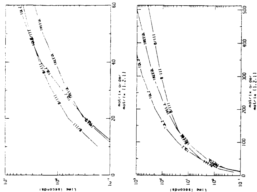
Figure 6.1: Times for TQL2, TREEQL, and B/III versus matrix order for matrix [1,2,1].
