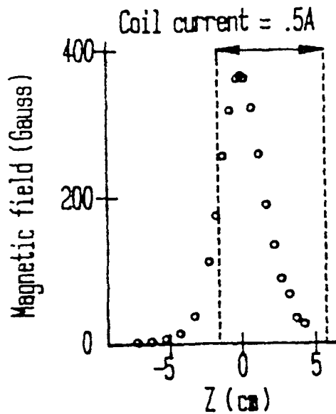
(a) Axial magnetic field on the Z axis.
