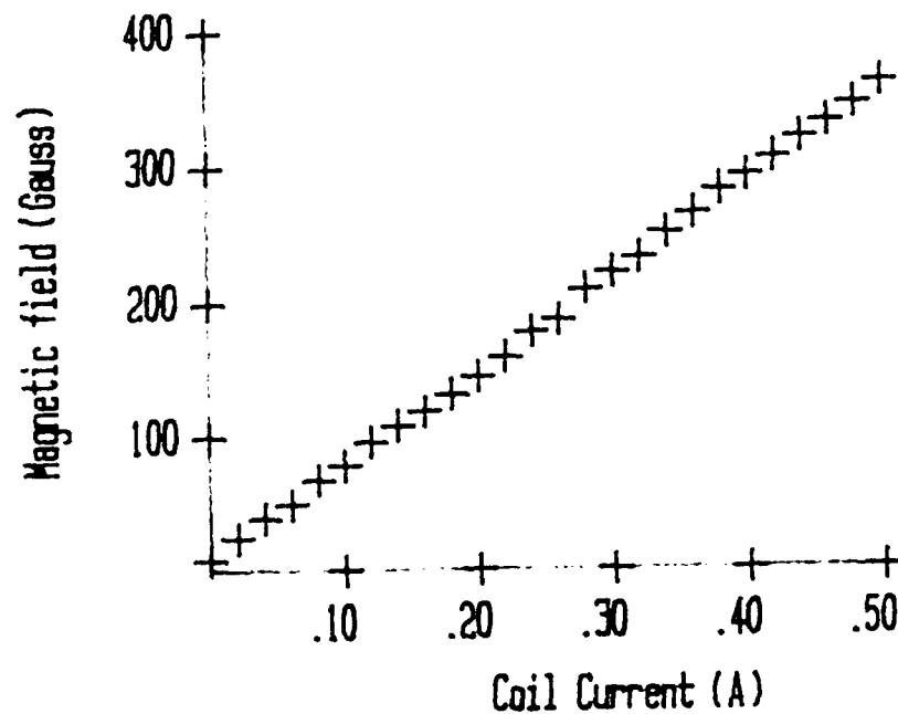
(c) Field vs. coil current.
