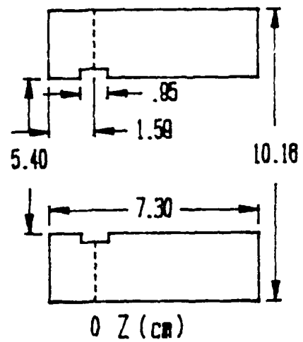
(b) Solenoid dimensions (cm).
