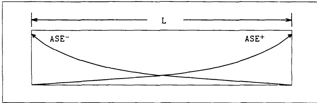
Figure 2.6. Relative intensity for ASE traveling in both directions
