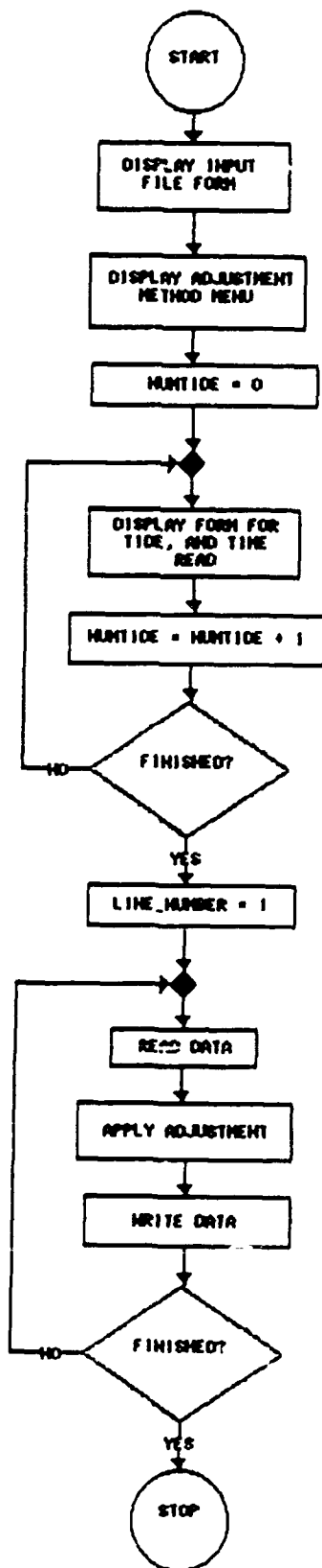
Figure C9. Flowchart, ADJUST DEPTHS FOR TIDE
