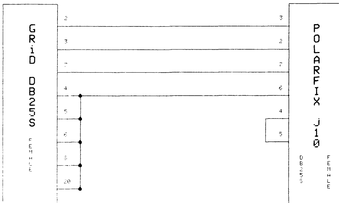
Figure B2. Polarfix cable (Polarfix is a registered trademark of Krupp Atlas)
