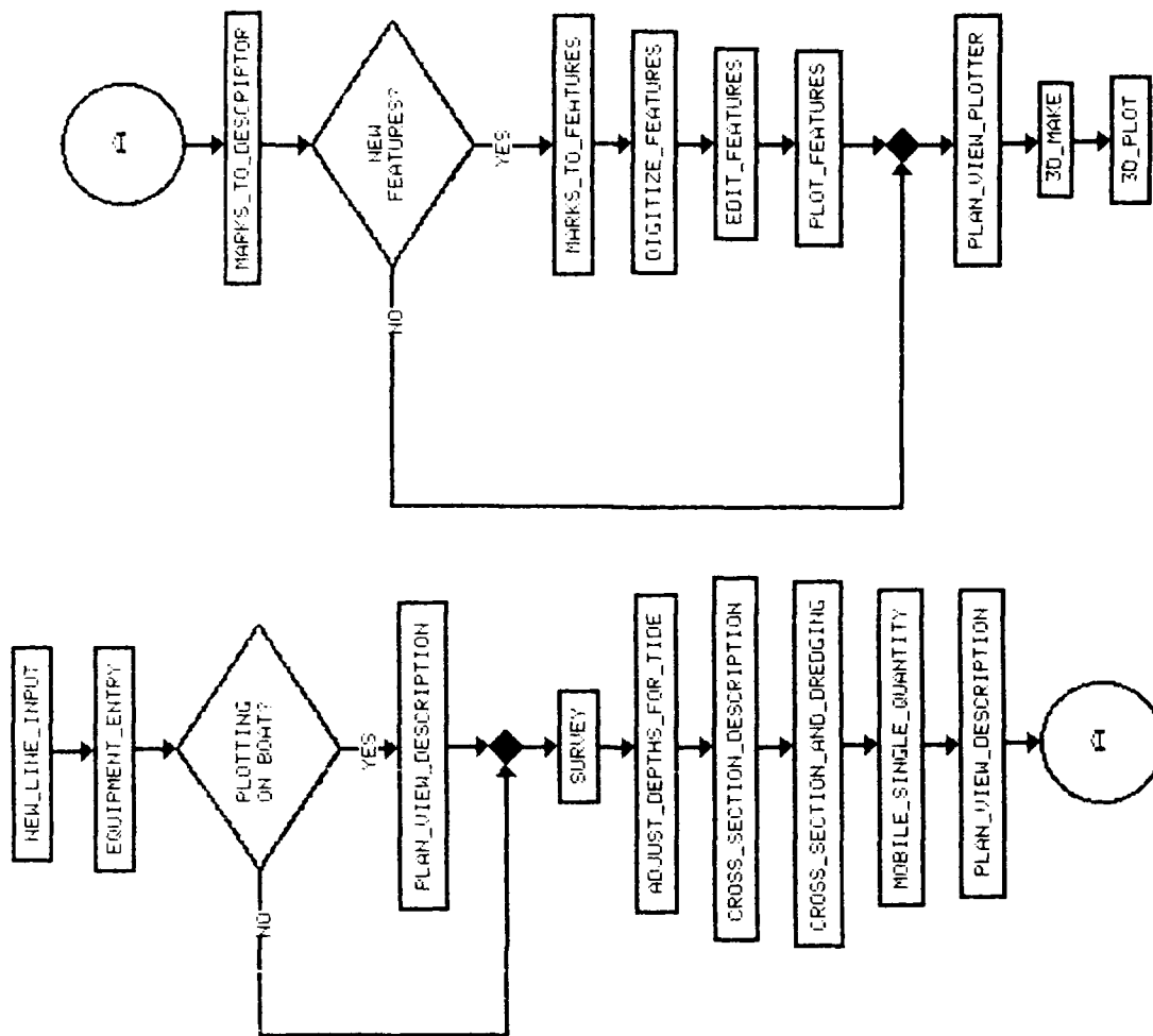
Figure 27. Random or section line survey typical program flow
