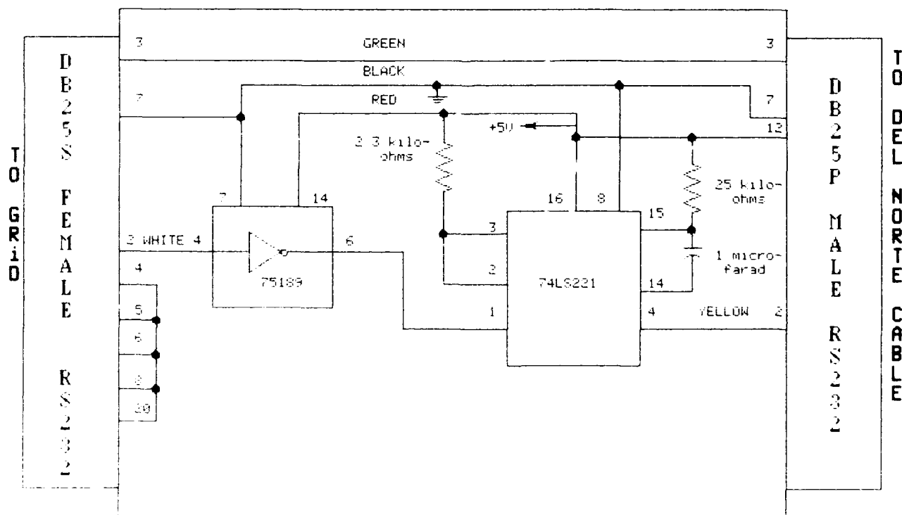
Figure B4. Del Norte RS232 to TTL Box
