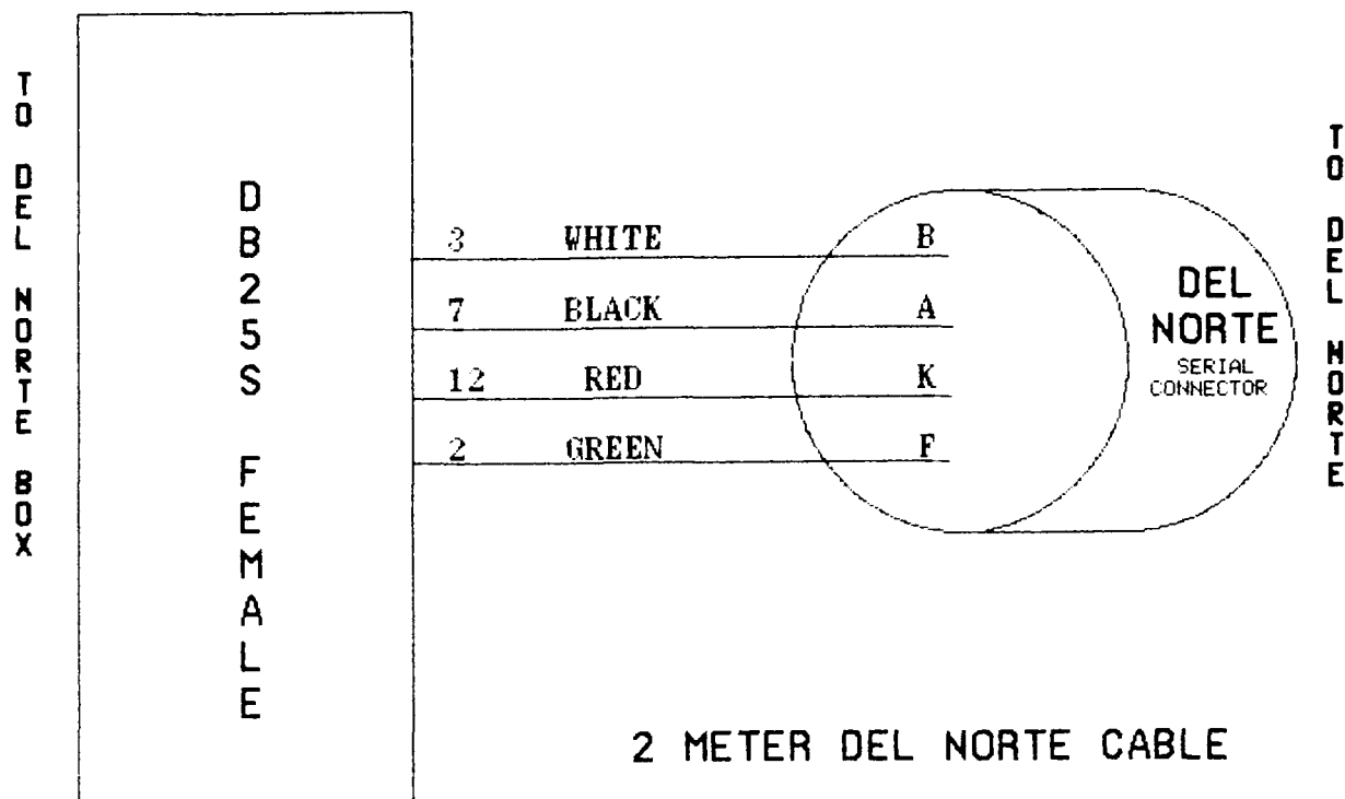
Figure B3. Internal to Del Norte jumper J22-39 to J1-K (serial). (Note: Pin J is used instead of K on older boxes.) (Del Norte is a registered trademark of Del Norte Technology)
