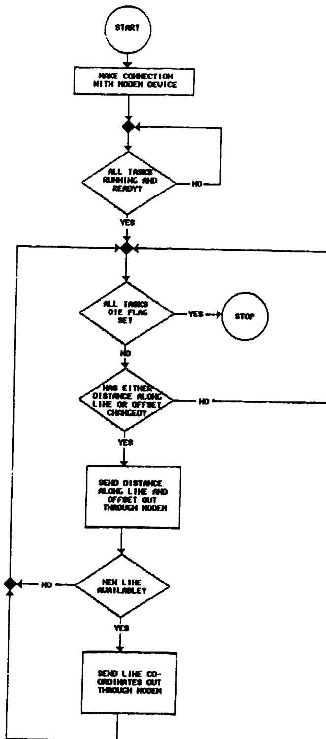
Figure C52. Flowchart, PILOT
