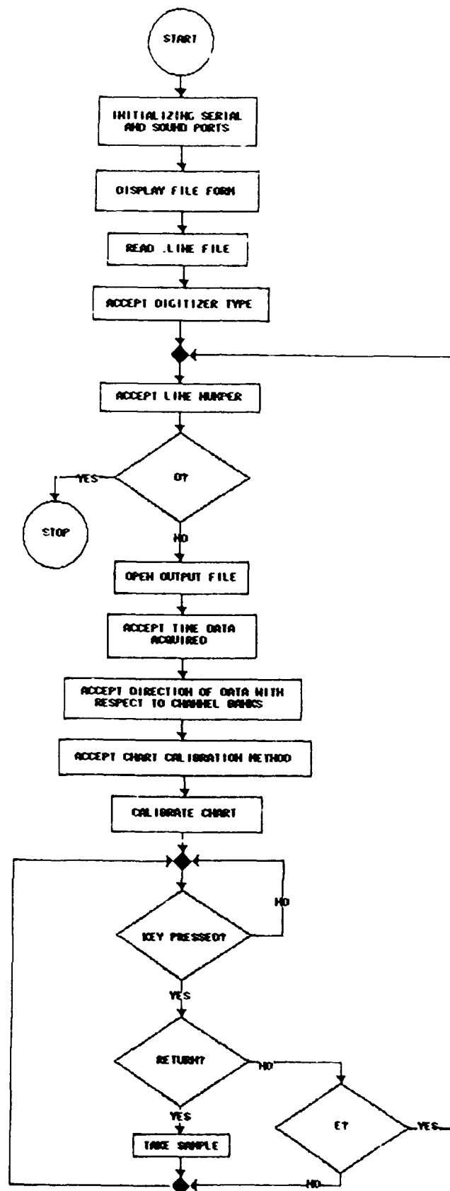
Figure C21. Flowchart, DIGITIZE_DEPTH_CHART
