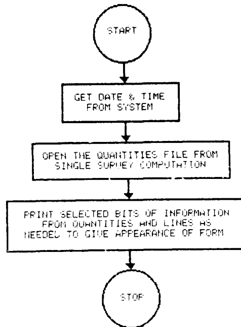
Figure C46. Flowchart, MOBILE_SINGLE_QUANTITY
