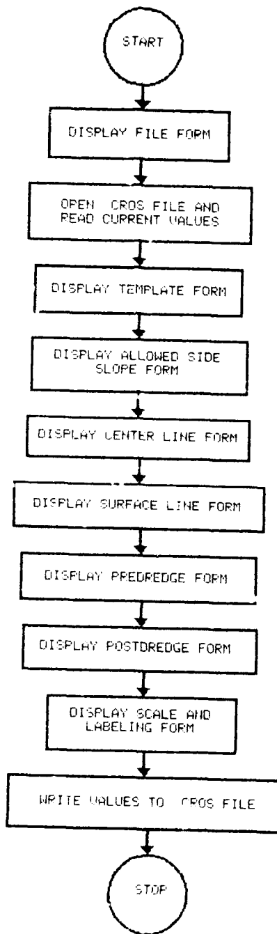
Figure C17. Flowchart, CROSS_SECTION_DESCRIPTION
