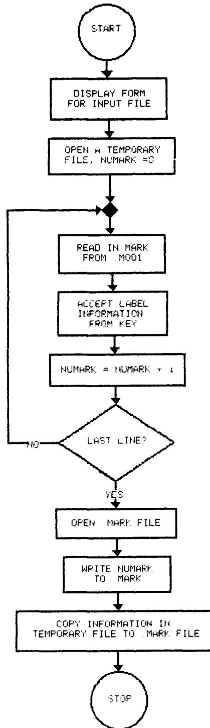
Figure C40. Flowchart, MARKS_TO_DESCRIPTOR
