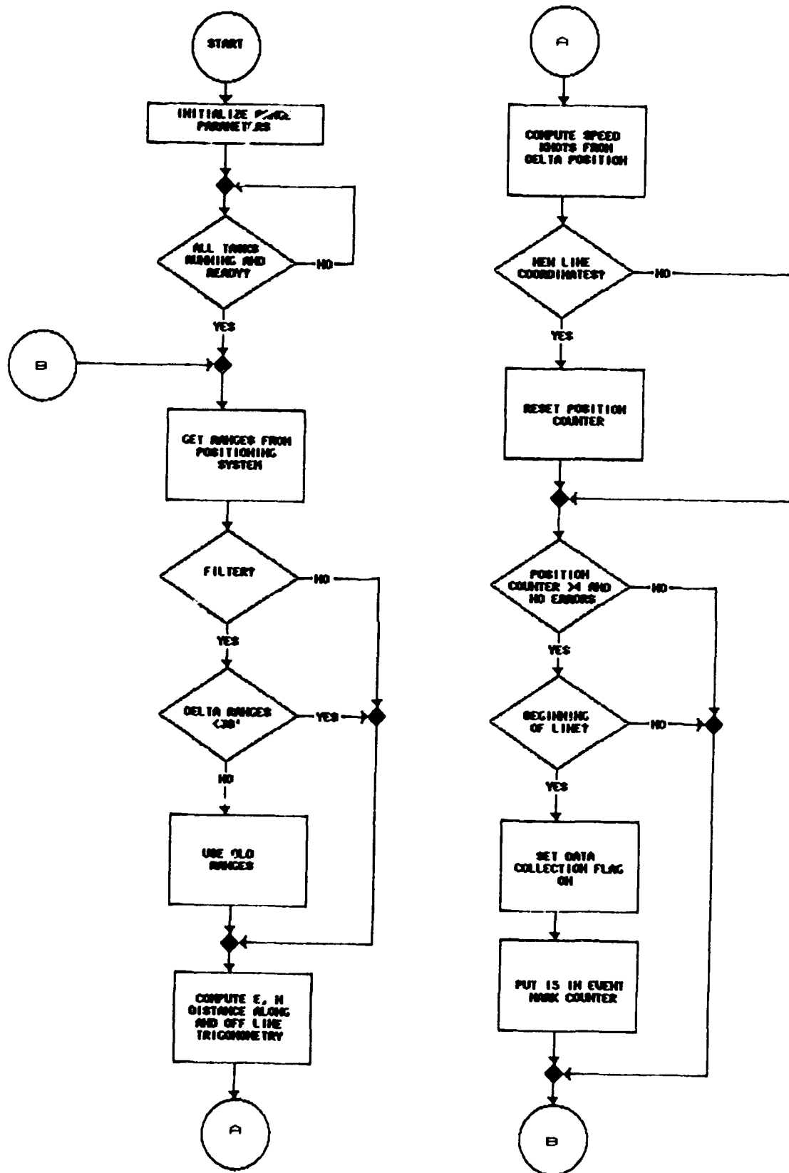
Figure C73. Flowchart, RANGE_DEVICE
