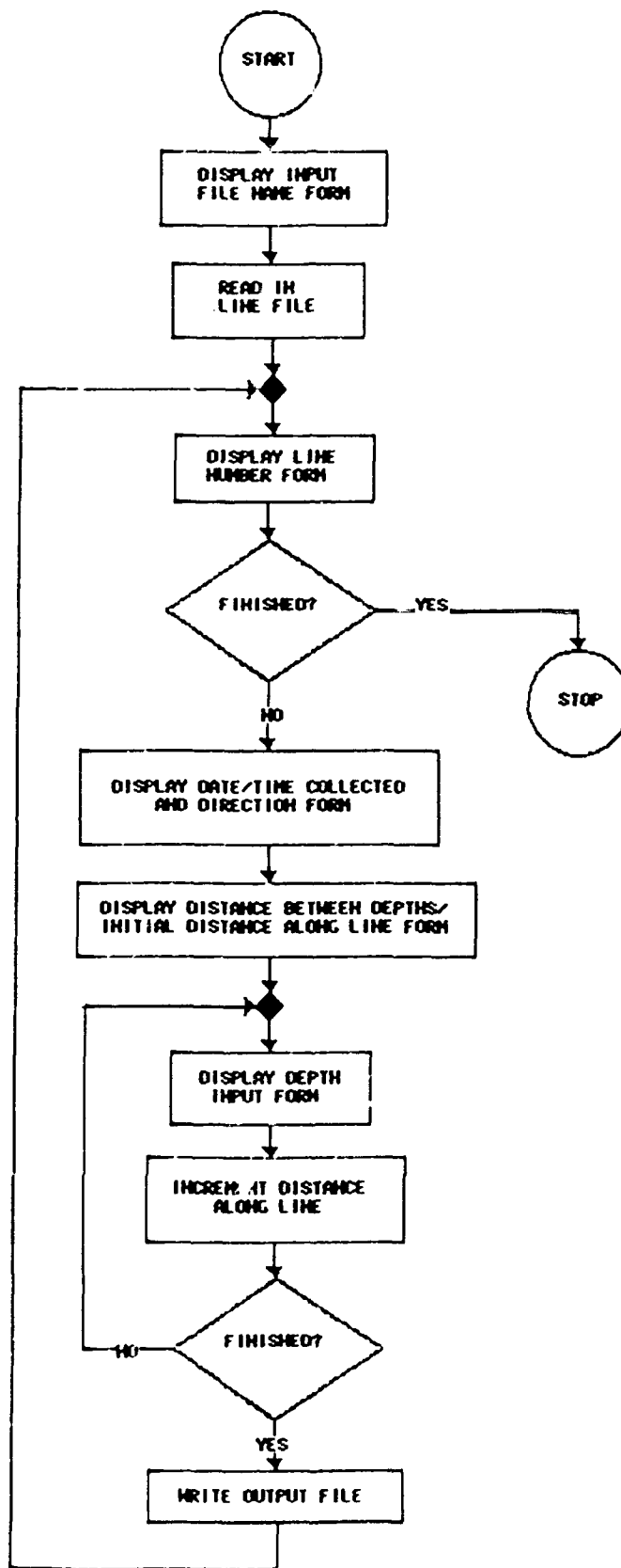
Figure C37. Flowchart, MANUAL_SURVEY_ENTRY
