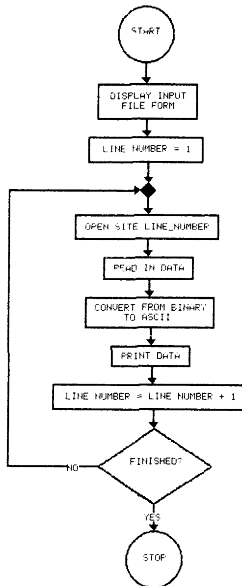
Figure C67. Flowchart, PRINT_DATA
