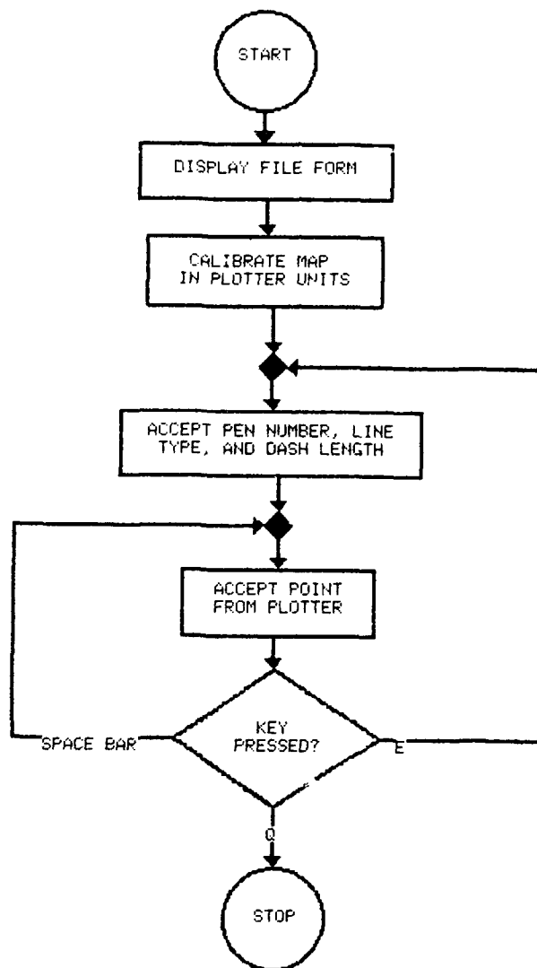
Figure C25. Flowchart, DIGITIZE_PLOTTER
