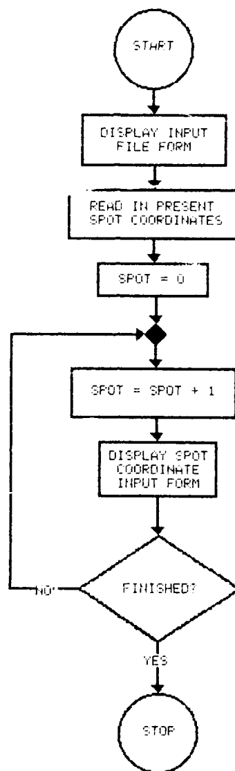
Figure C50. Flowchart, NEW_SPOT_INPUT
