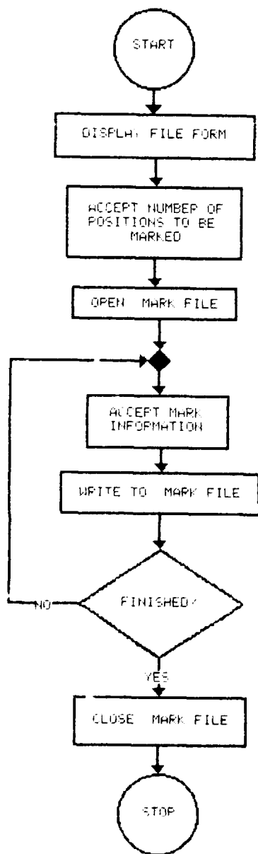
Figure C42. Flowchart, MARK_DESCRIPTION
