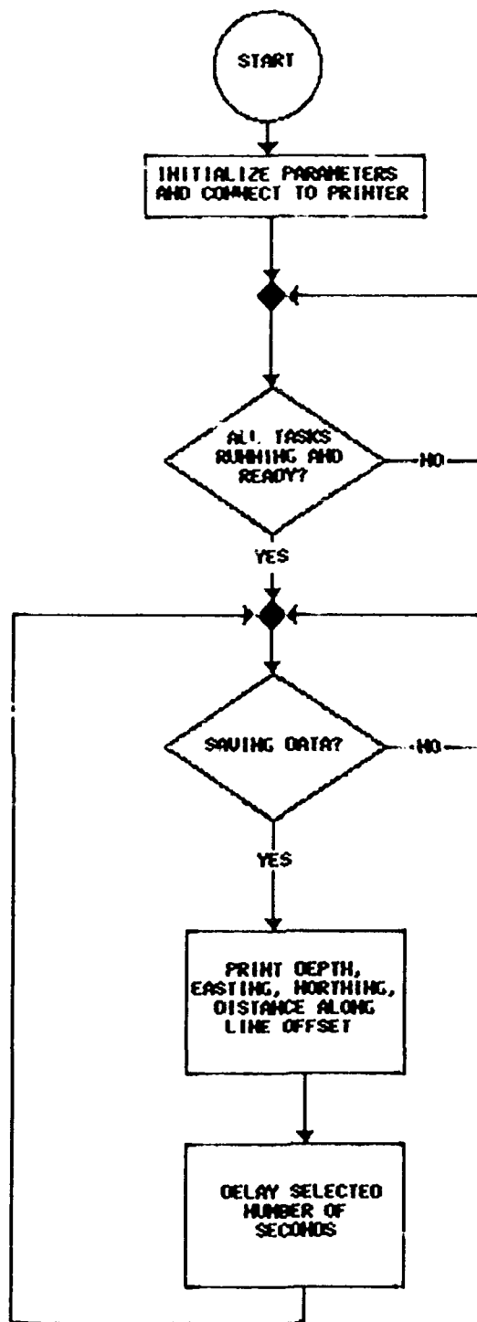
Figure C66. Flowchart, PRINT
