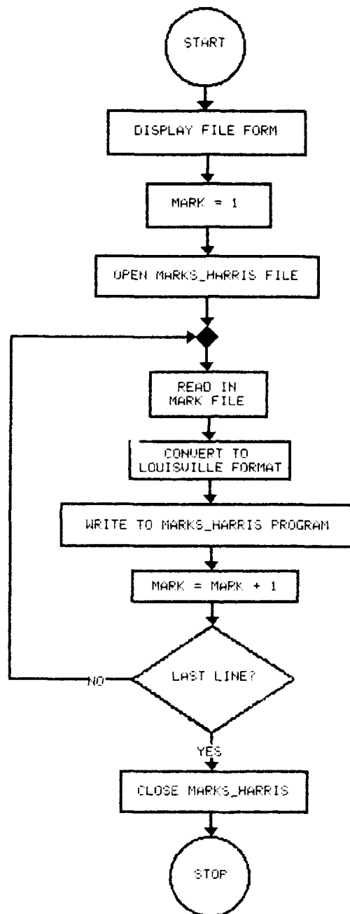
Figure C39. Flowchart, MARKS_HARRIS
