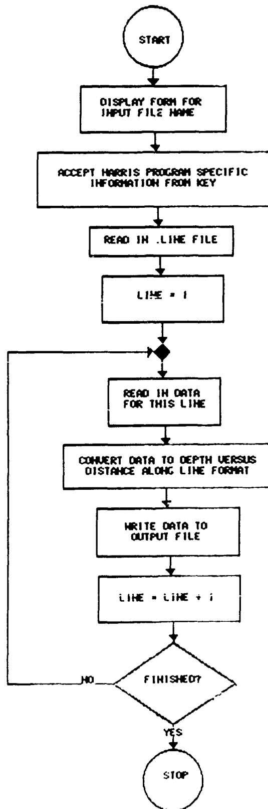
Figure C13. Flowchart, CONVERT_DATA
