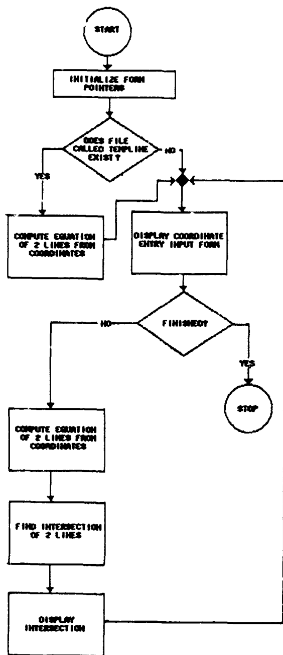
Figure C35. Flowchart, INTERSECTION_OF_2_LINES
