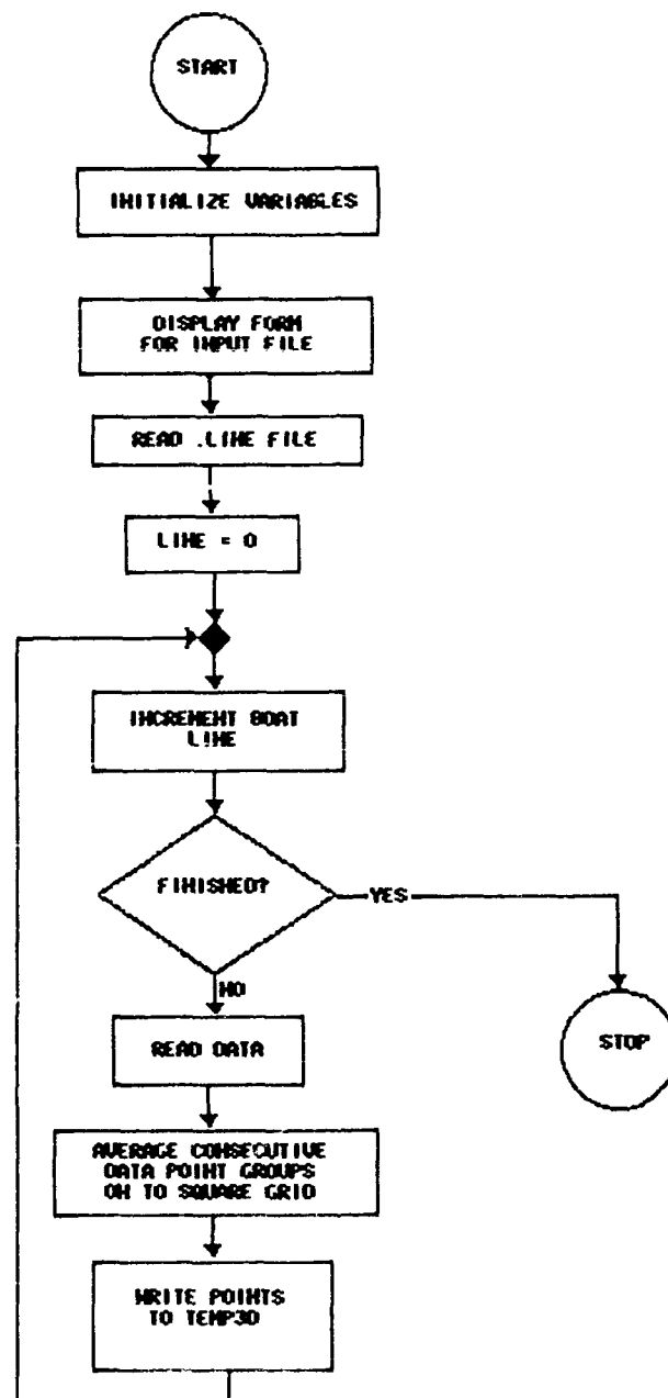
Figure C15. Flowchart, CROSS_SECTION_AND_DREDGING
