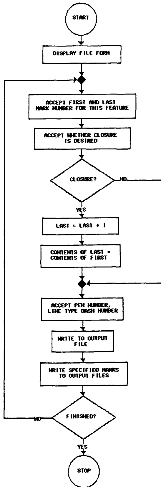
Figure C41. Flowchart, MARKS_TO_FEATURES
