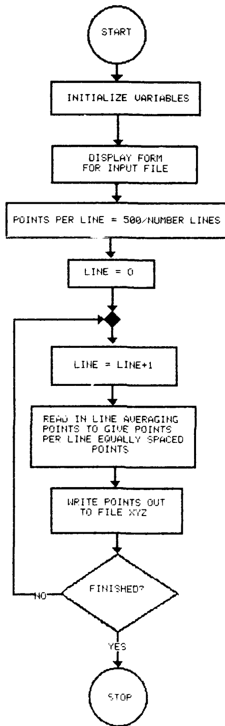
Figure C7. Flowchart, ACAD_XYZ
