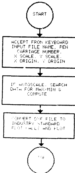
Figure C5. Flowcharts, ACAD_PLOT
