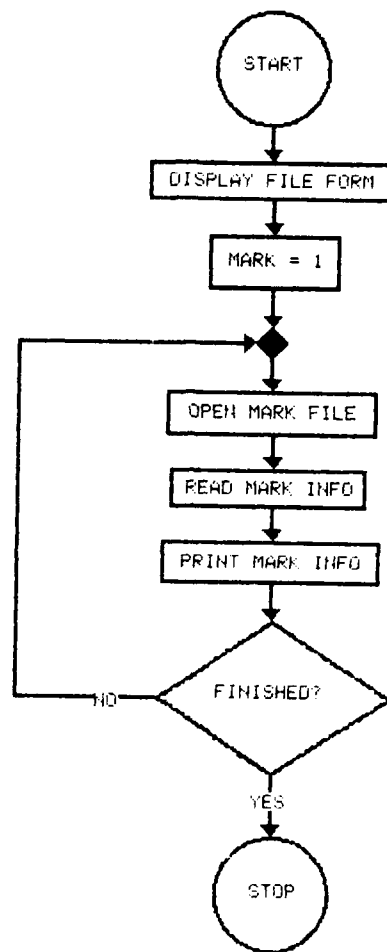
Figure C69. Flowchart, PRINT_MARKS
