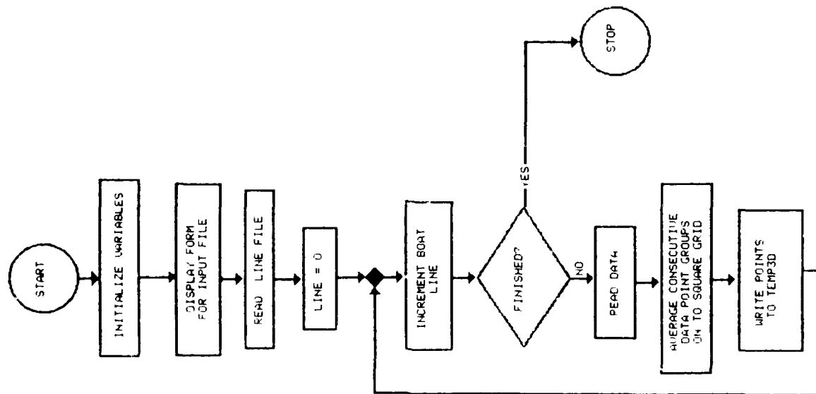
Figure C1. Flowchart, 3D_MAKE
