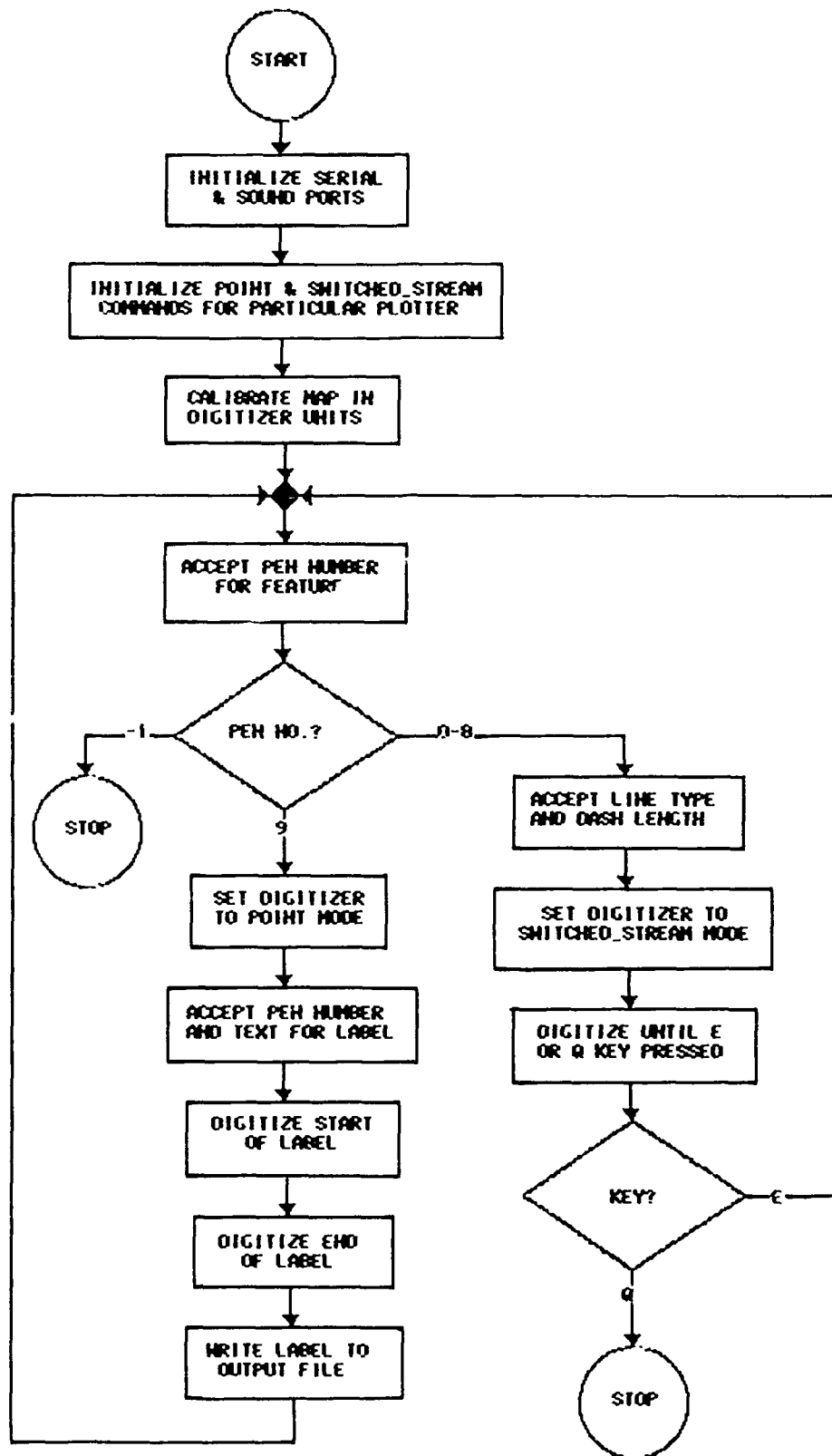
Figure C23. Flowchart, DIGITIZE_FEATURES
