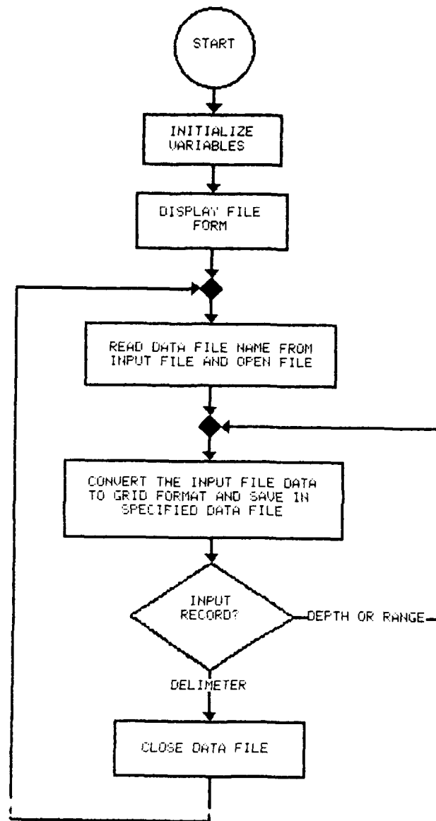
Figure C33. Flowchart, GENERIC_TO_GRID_FORMAT
