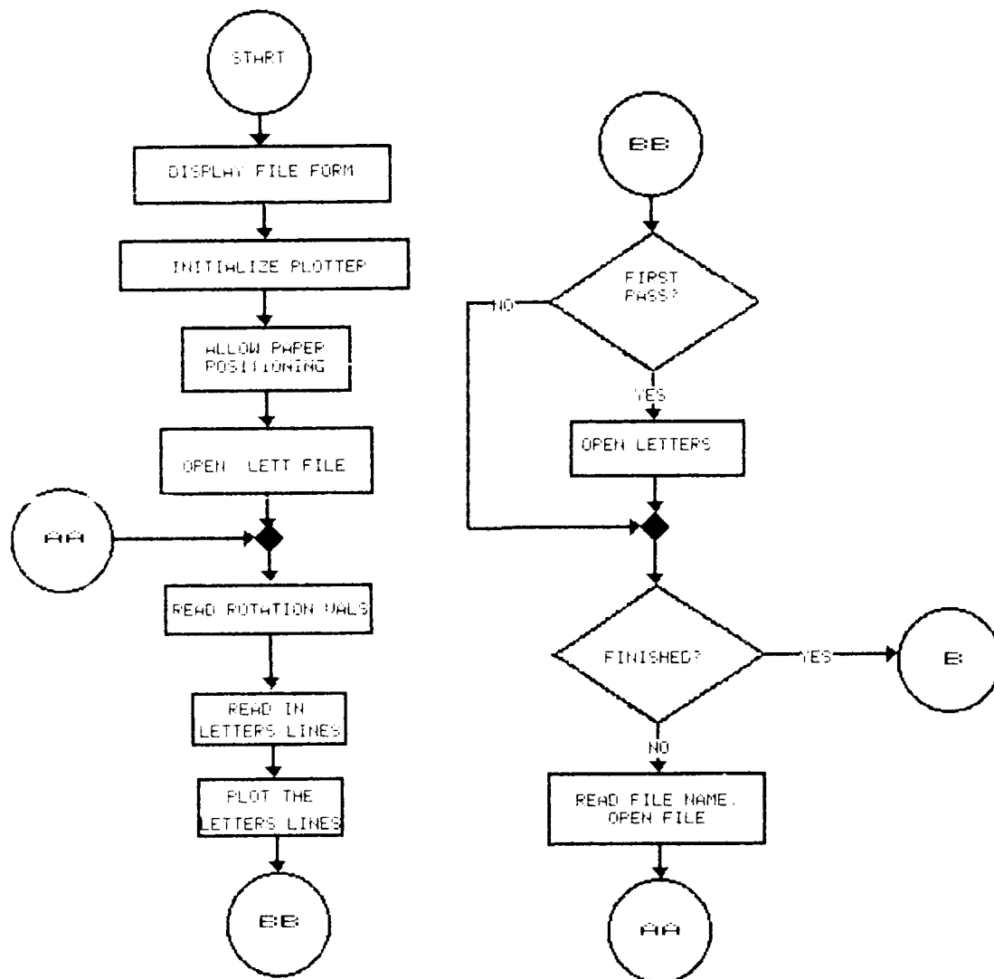
Figure C57. Flowchart, PLOT_LETTERS
