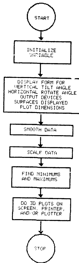
Figure C3. Flowchart, 3D_PLOT
