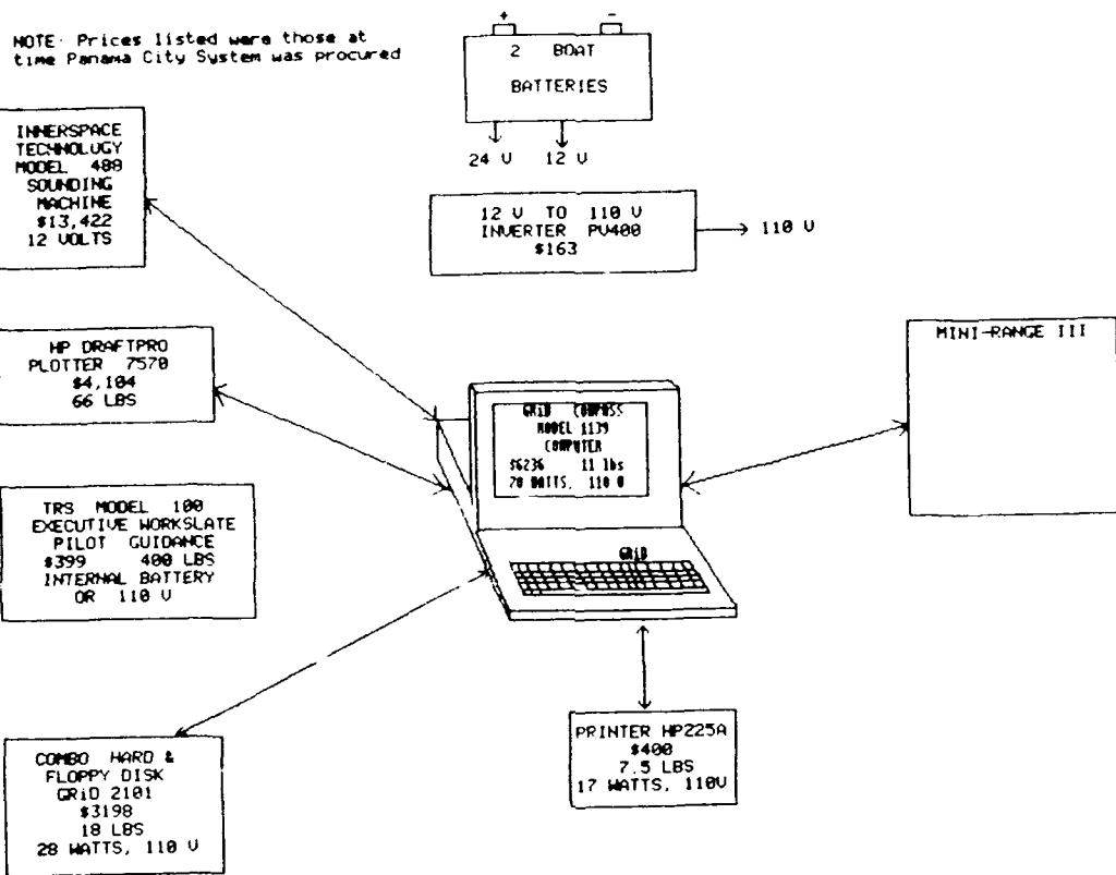
Figure 13. Panama City Mini-Ranger III
