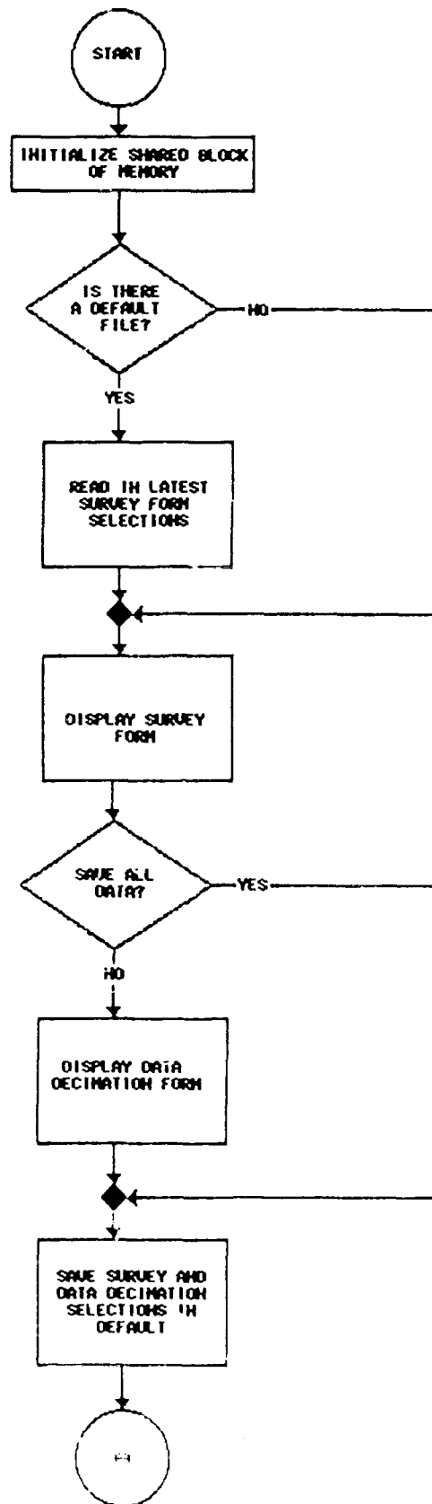
Figure C11. Flowchart, CONFIGURE (Continued)
