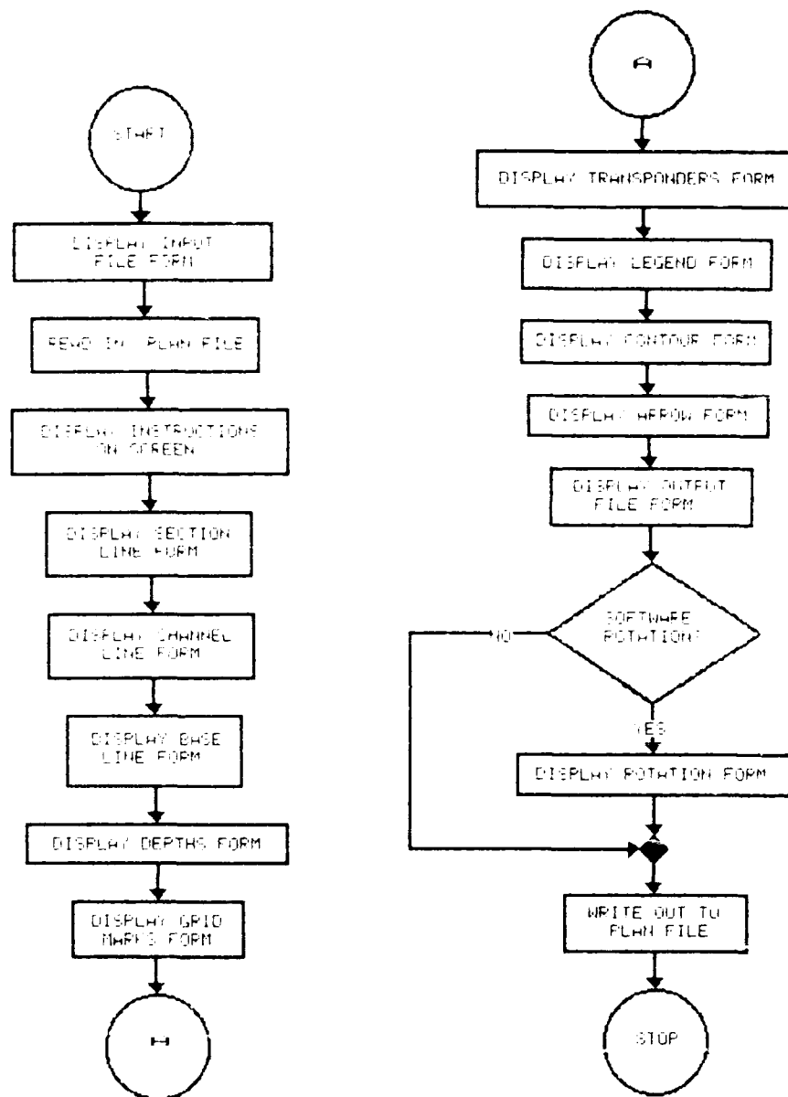
Figure C53. Flowchart PLAN_VIEW_DESCRIPTION
