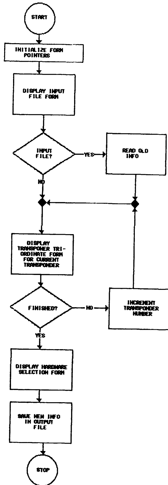
Figure C30. Flowchart, EQUIPMENT_ENTRY
