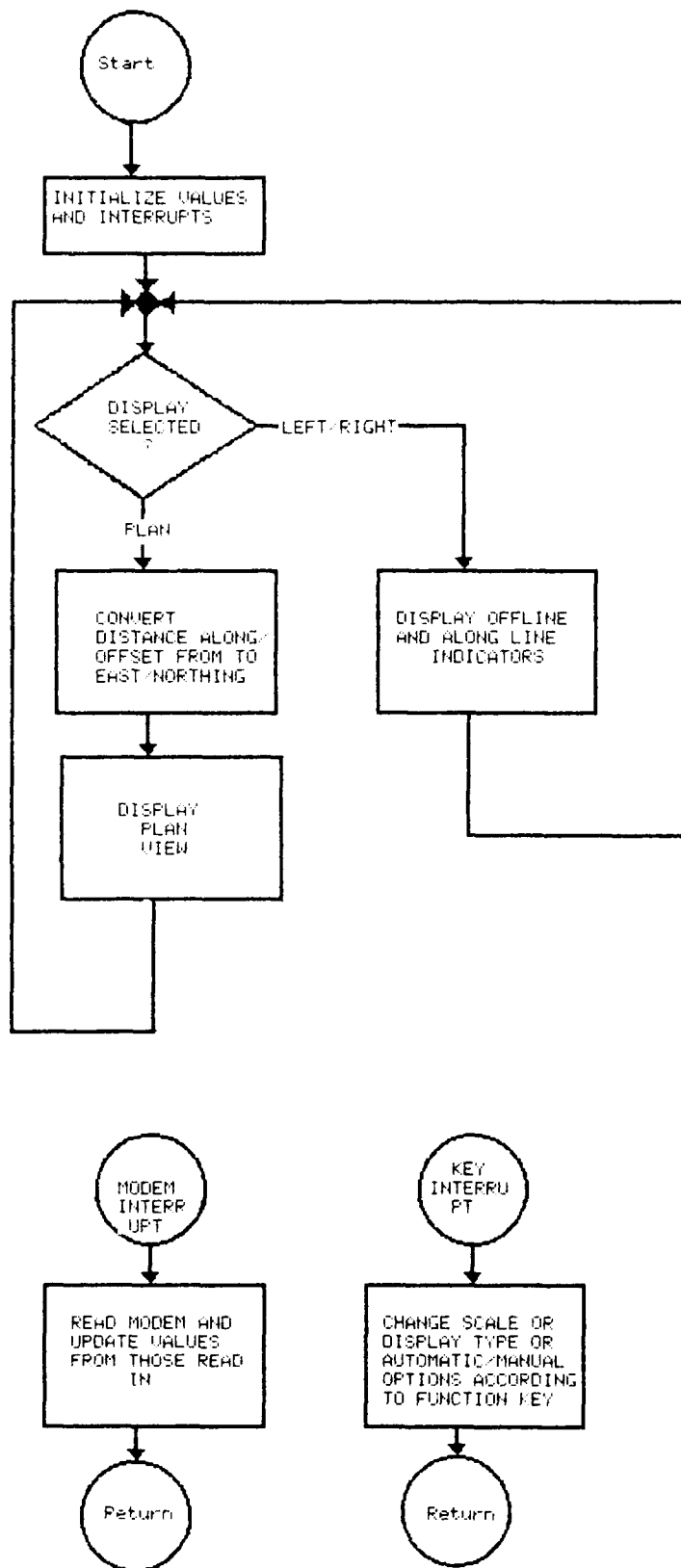
Figure C34. Flowchart, INDICATOR
