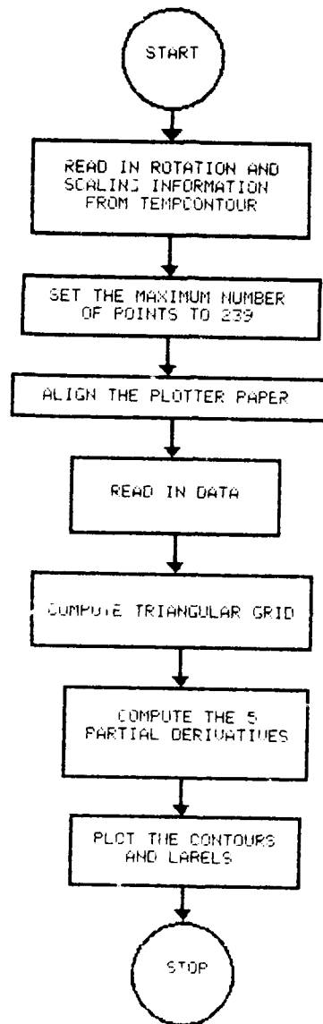
Figure C12. Flowchart, CONTOUR_PLOT
