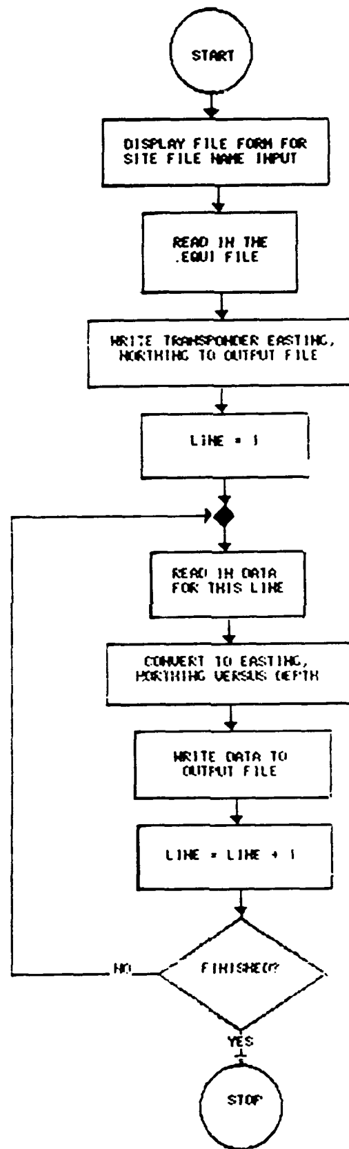
Figure C14. Flowchart, CONVERT_DATA_LOUISVILLE
