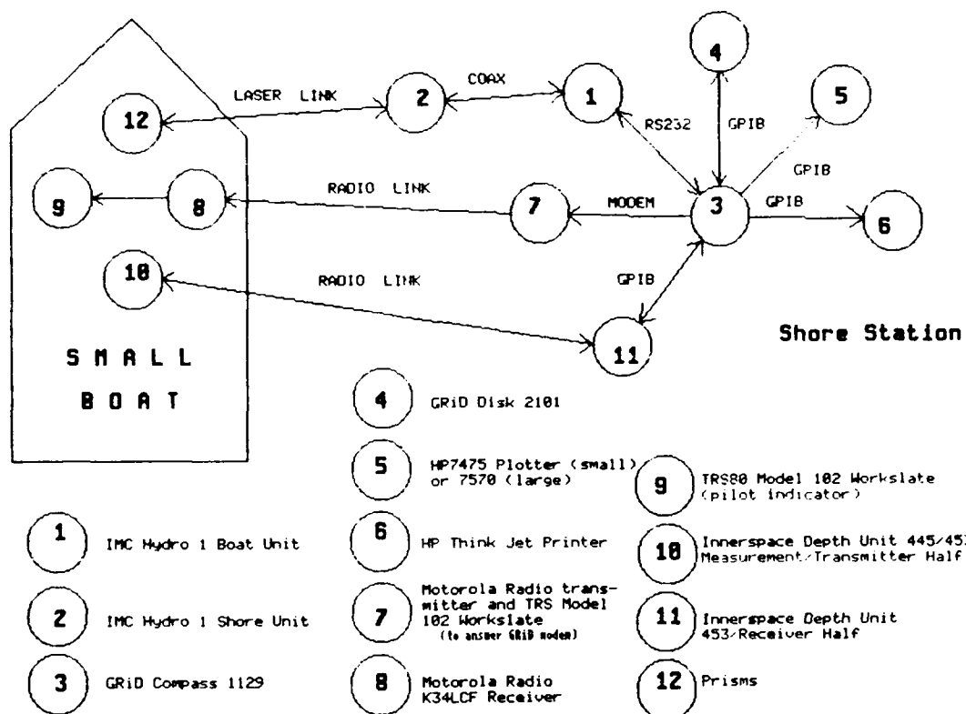
Figure 9. Configuration 1, computer on shore
