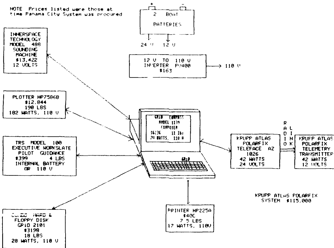
Figure 14. Panama City Krupp Atlas Polarfix
