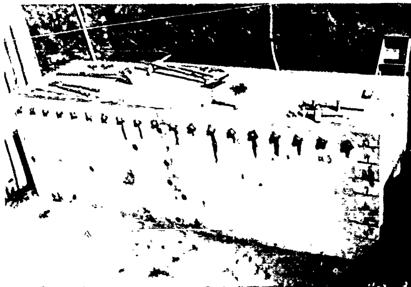
Figure 4.17. Reaction structure and test slab before Backfill Test 3.
