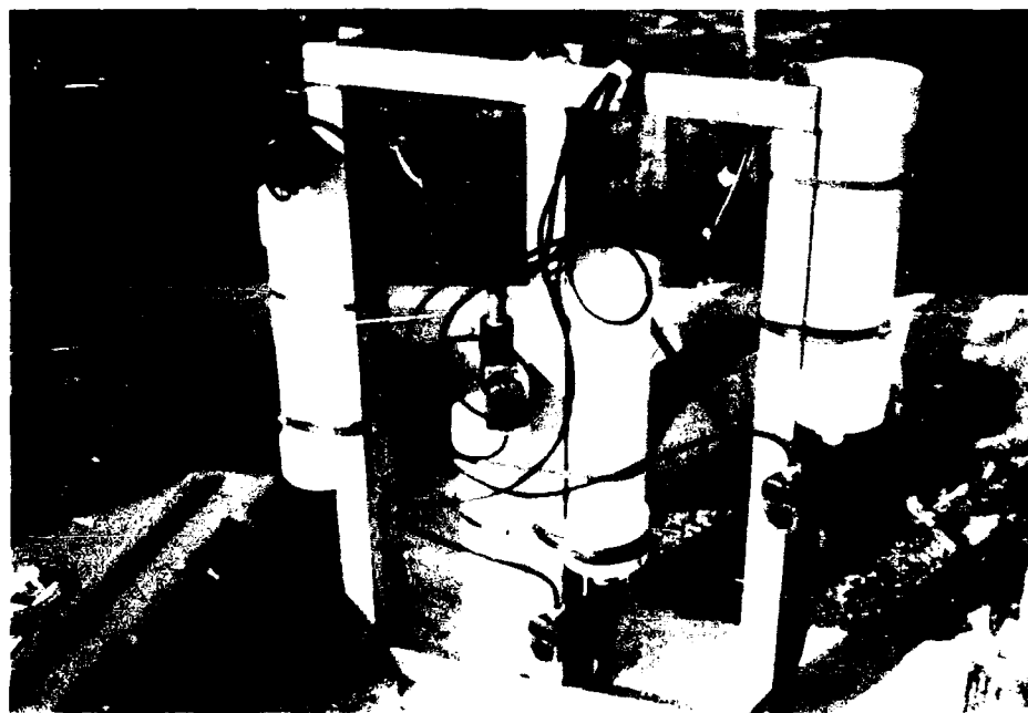
Figure 13. Vacuum sediment sampler
