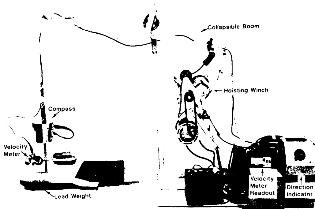
Figure 3. Components of the field instrument assembly
