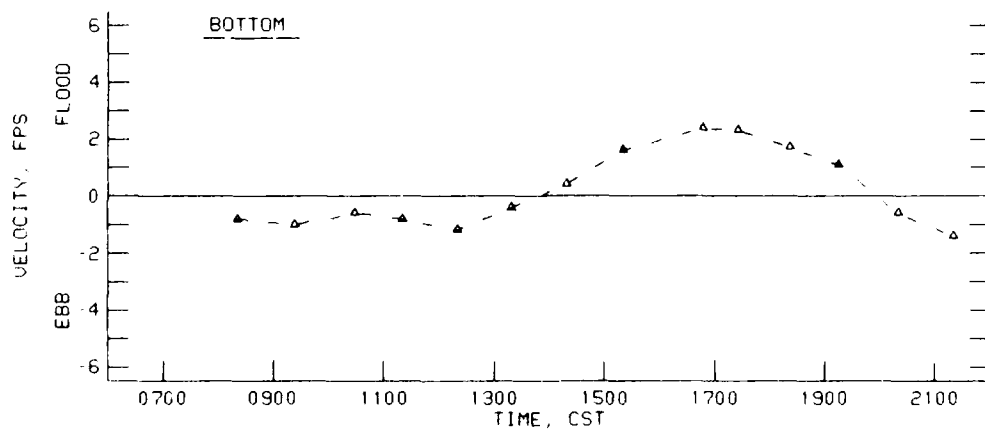
VELOCITIES AT STATION 1-C 19 JANUARY 1989
