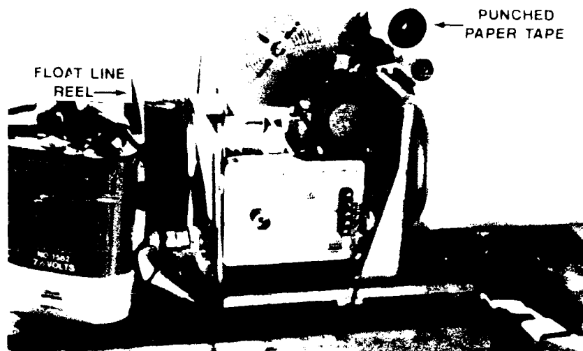
Figure 7. Punched paper mechanical water level recorders
