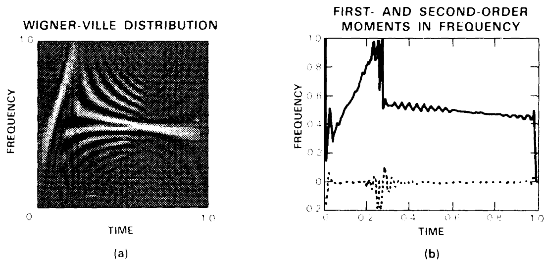
Figure 5. The WVD of a normalized down-chirp waveform. Normalized time-frequency axes are used. It is assumed that the down-chirp waveform is of the form f(t) = A \exp(j2\pi f_0 t - j\pi k t^2) , and with a time duration of 1. The bandwidth of the down-chirp waveform is half that of the up-chirp. The WVD of the up-chirp waveform is shown in (a). In (b), the first-order moment of the WVD component associated with the down-chirp waveform is shown as the solid line and the second-order moment is shown as the dashed line. The time-frequency axes are normalized to the time duration of the down-chirp waveform.
