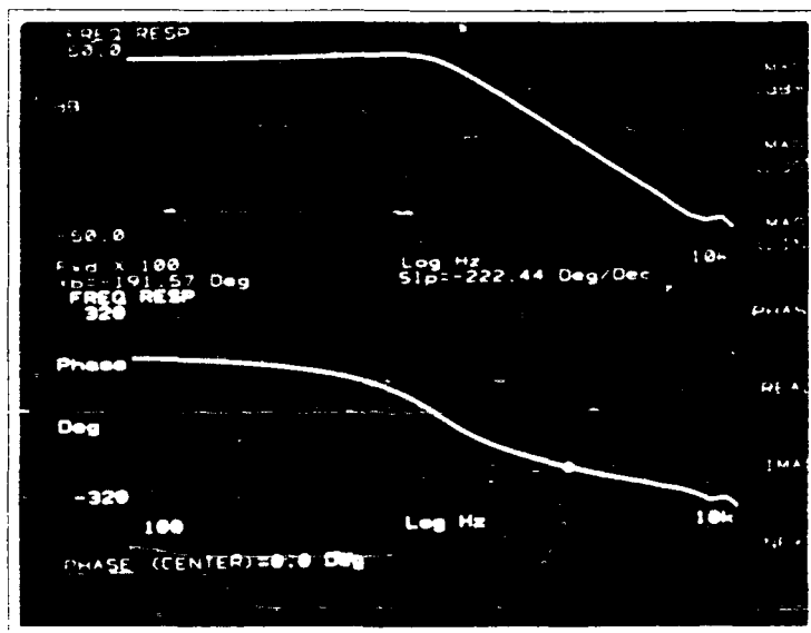
Figure 1. Frequency Response
