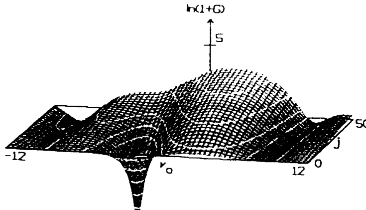
Figure 5. The gain spectrum G(\nu_0, j) dependence on j .
