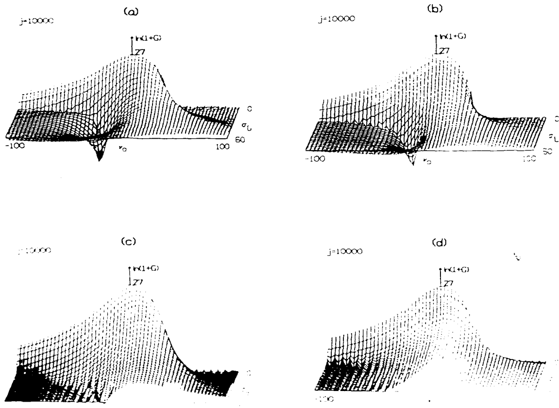
Fig. 2. The FEL gain surface \ln(1 + G) as a function of current j = 10^4 .
