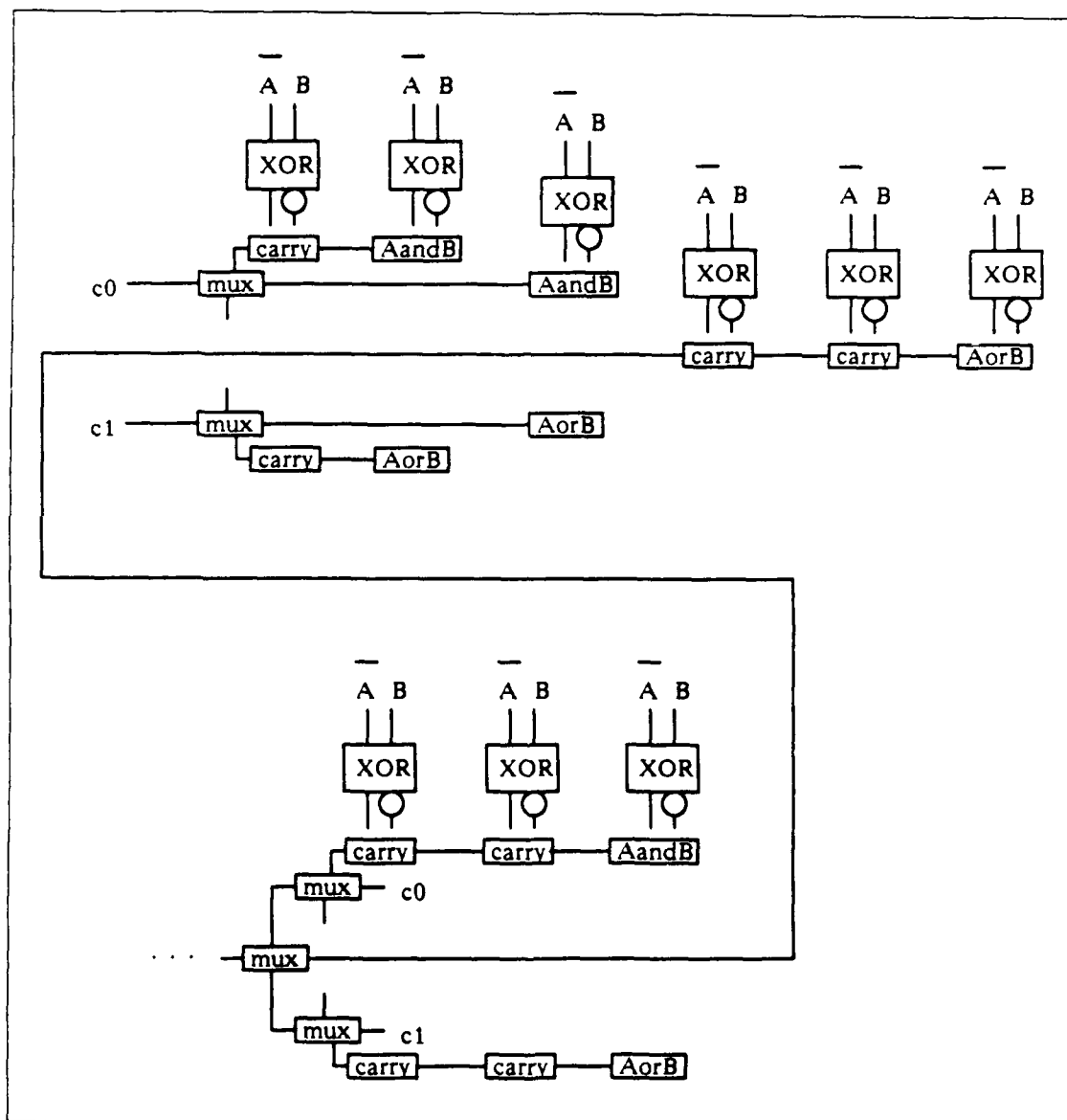
Figure 4.27. OCM Comparitor (321,3)
