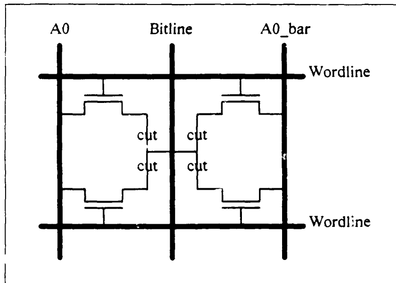
Figure 5.1. LEPROM Cell
