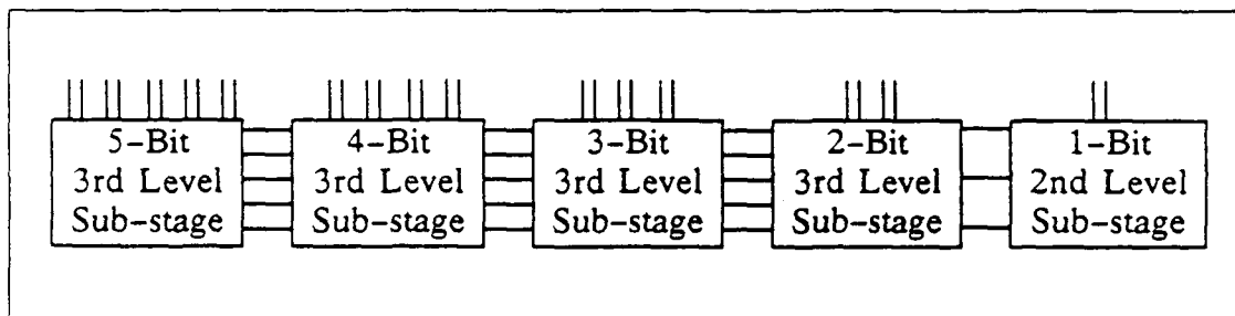
Figure 4.11. Fifteen-bit Stage
