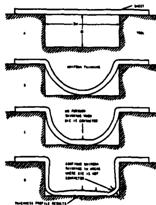
Fig. 26. Illustration of thinning characteristics in the blow forming of an unlubricated part of rectangular cross-section and semi-infinite length.
