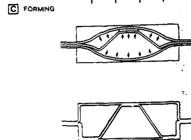
Three-sheet SPF/DB
