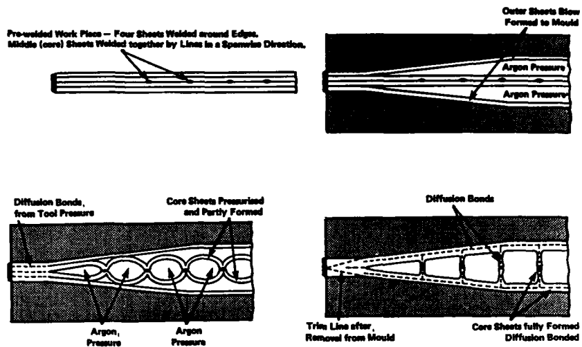
FIGURE 29 Advanced manufacturing, involving SPFD
