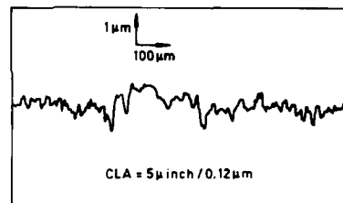
Fig 7 Talysurf Traces for Al Sheet
