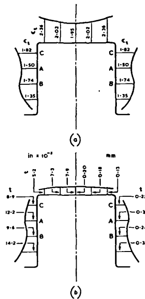
Fig. 34. Thickness profile for "hat" configuration formed with a concave die member as shown in Fig. 32. (20)
