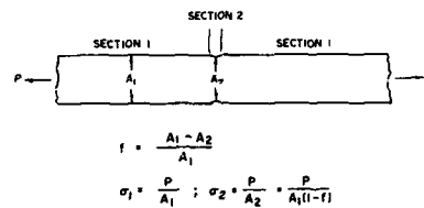
Fig. 17. Geometric inhomogeneity in a tensile specimen.
