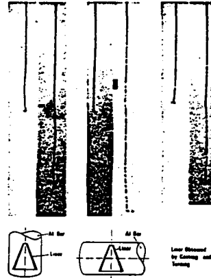
Fig. 27 Flash radiographs of an aluminum rod undergoing large strain plastic deformation at extremely high strain rates (125).
