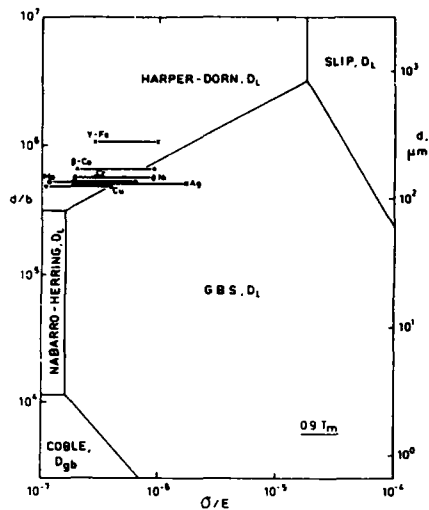
Fig. 26 Deformation map for metals and dilute alloys at a high homologous temperature ( 0.9T_m ). H-D creep dominates at low stresses and coarse grain sizes and has been used to explain the Newtonian-viscous creep behavior of the pure metals shown in the figure (123).
