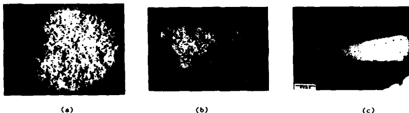
Figure 15. Longitudinal sections of \alpha/\beta brasses pulled to failure (a) 60/40 (b) 59/41 (c) 58/42.
