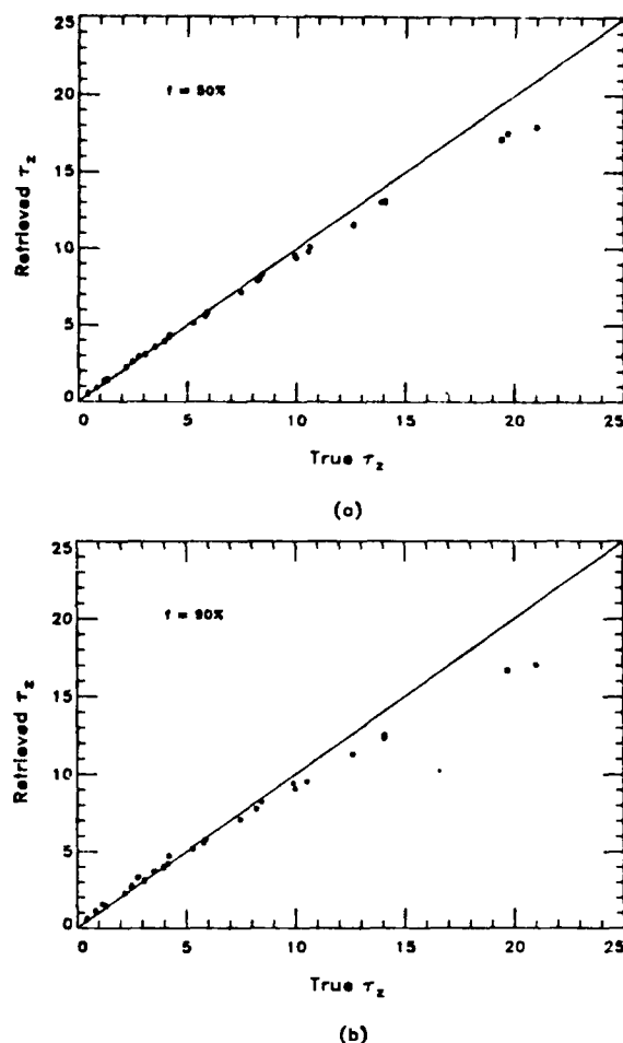
Fig. 15. Comparison between the source optical depth, \tau_z \equiv cz_0 , retrieved by inverting Eq. (36) for various pigment concentrations and source physical depths: (a) f = 50\% ; (b) f = 90\% .
