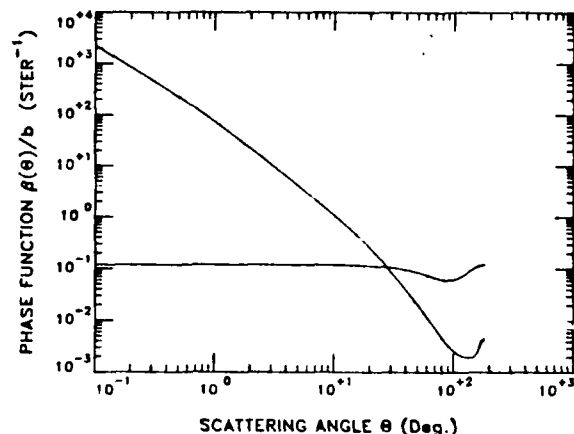
Fig. 1. Particle scattering phase function used in this study. The water phase function (lower curve at small scattering angles) is also shown for comparison.
