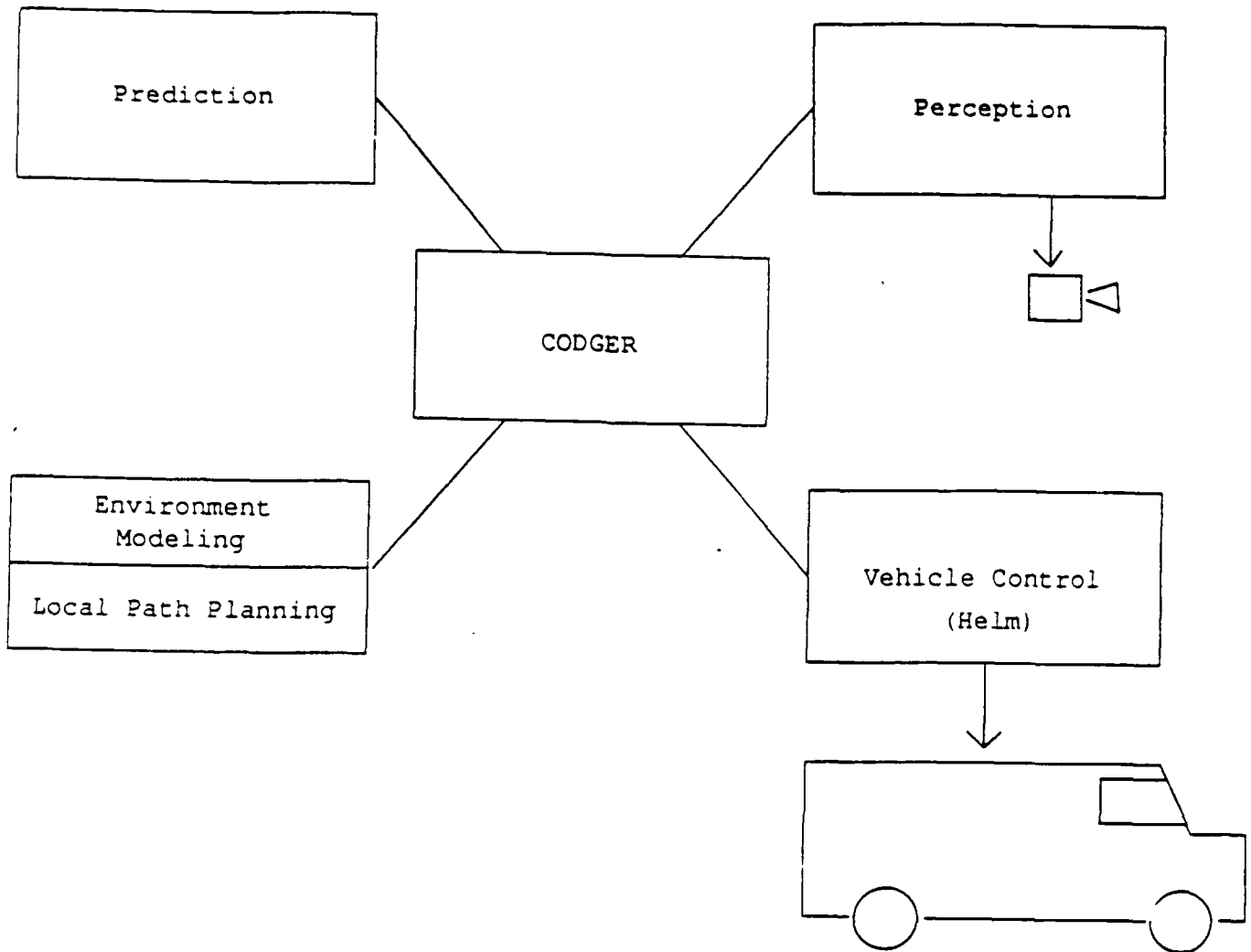
Figure 23: Module Structure
