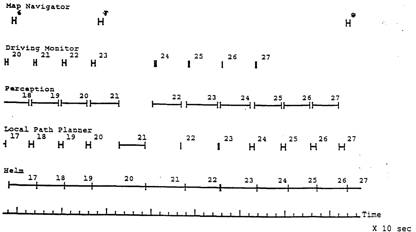
Figure 25: Timing Diagram of the Processing Steps
