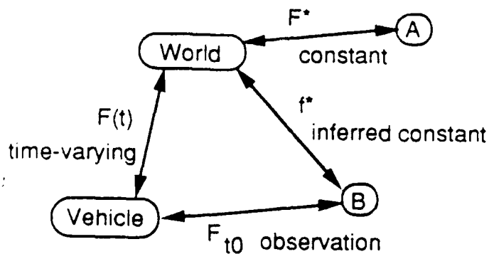
Figure 10: Several Types of Frame Generator
