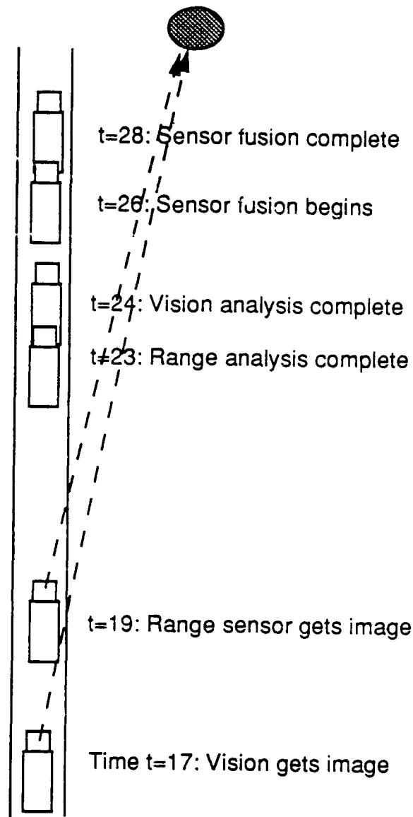
Figure 4: Fusion of Data in a Moving Robot
