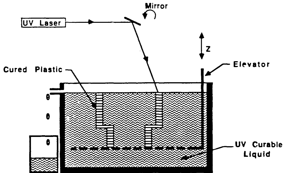
Figure 2-1: Stereolithography Apparatus
