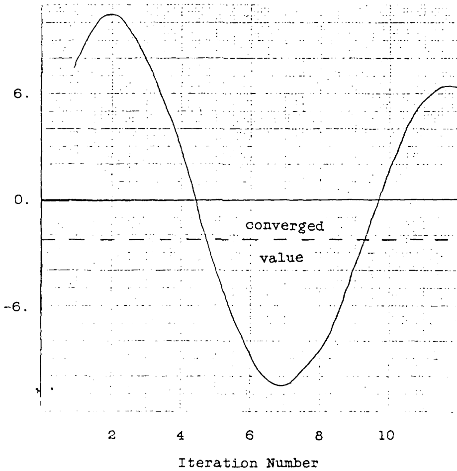
Figure 5: Sun Gear Displacement and Velocity Boundary Conditions vs. Number of Iterations
