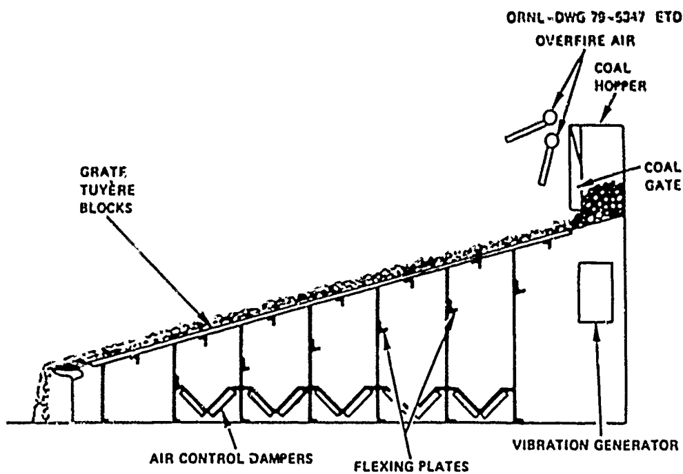
Fig. 6. Vibrating-grate stoker.
