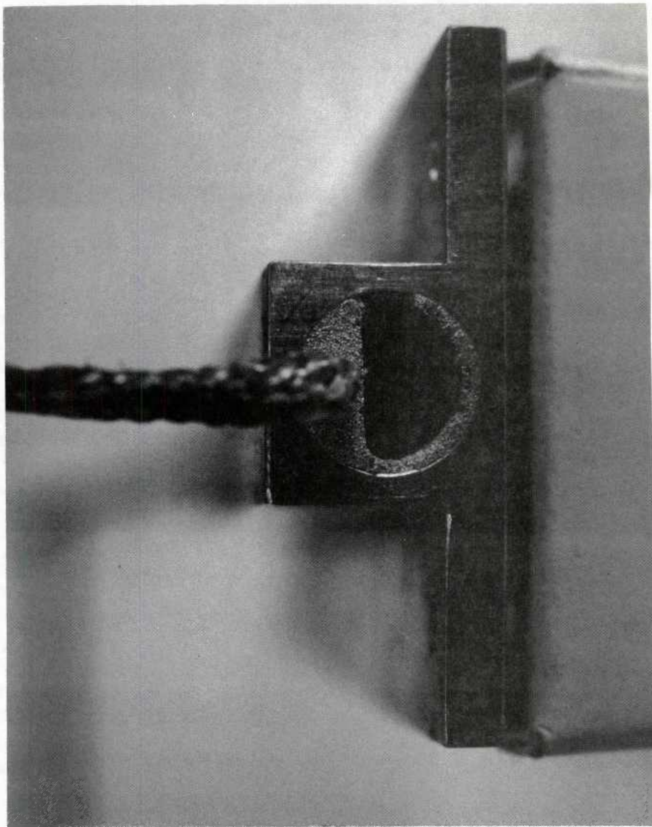
Figure 15. Photograph of condenser wick structure and artery cable
