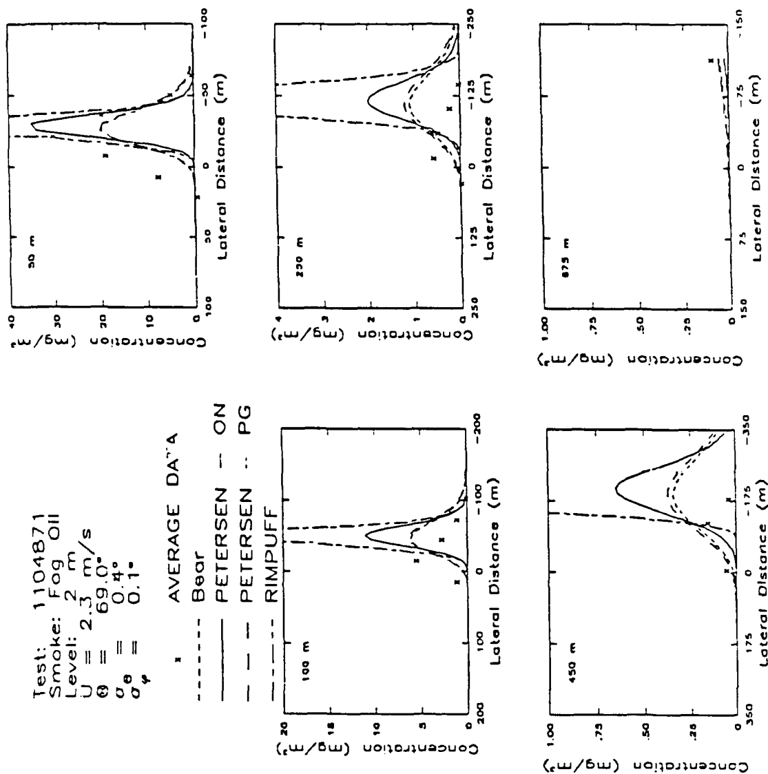
Figure 6.2. Comparison of RIMPUFF, BEAR, INPUFF-Onsite and INPUFF-PG mathematical models with average concentrations from test 1104871 at Camp Altermury.
