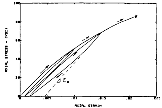
Fig. 1 Stress-strain behavior of Hercules AS4/3502 angle-ply laminate [\pm 30]_3 showing inelastic behavior.
