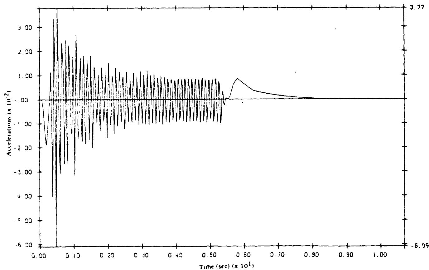
Figure A-3. Vertical displacements and accelerations at top of column (Monterey "O" sand)
