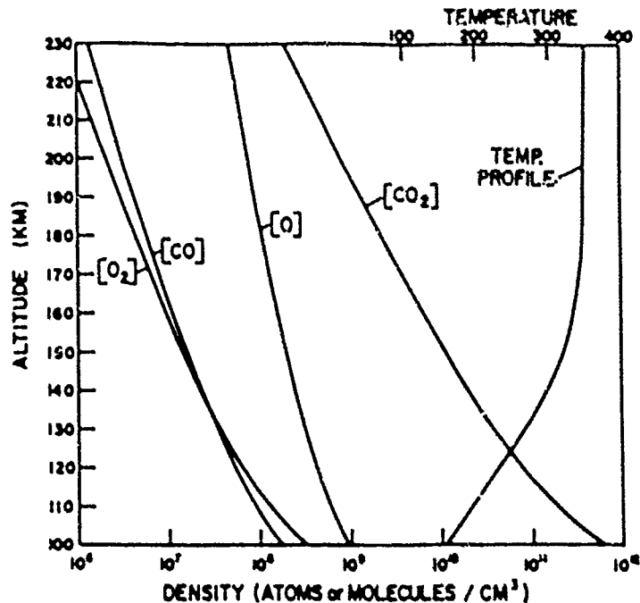
Figure 1.2: Ionosphere Density as a Function of Altitude
