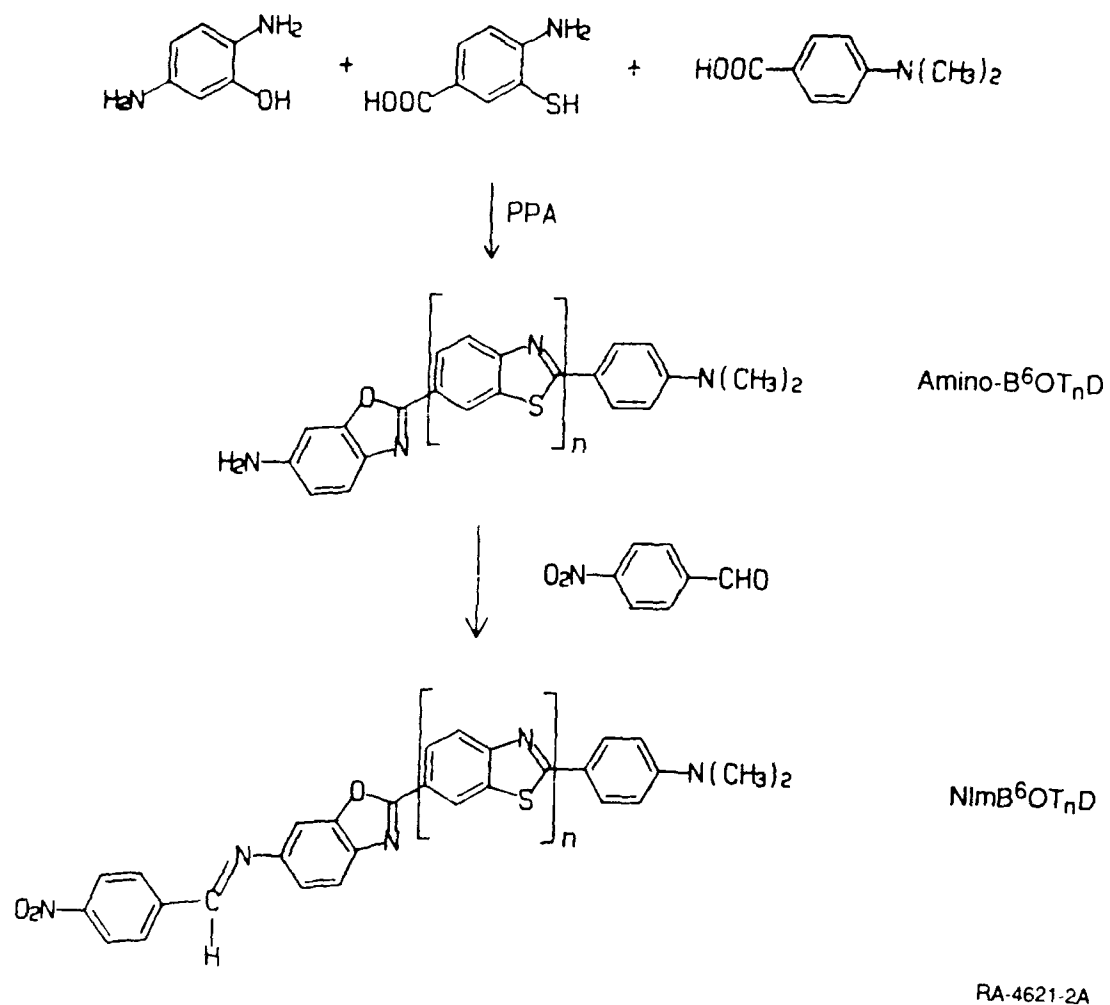
Figure 2. Synthesis of NIm-HD compounds.
