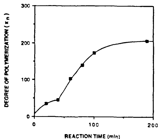
Figure 2 Degree of polymerization as a function of reaction time for polycondensation of 15 wt% PBT in PPA.
