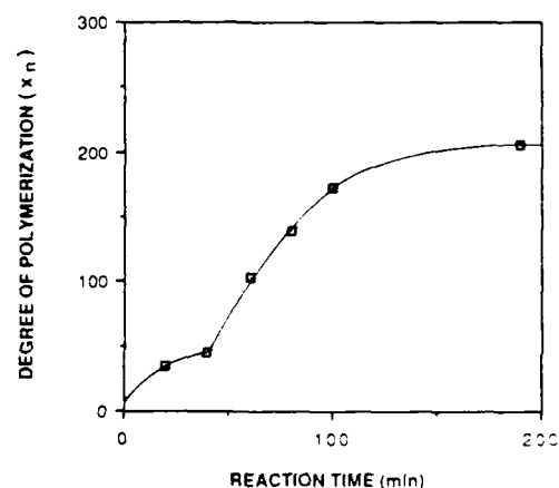
Figure 3. Degree of polymerization as a function of reaction time for polycondensation of 15 wt% PBT in PPA.
