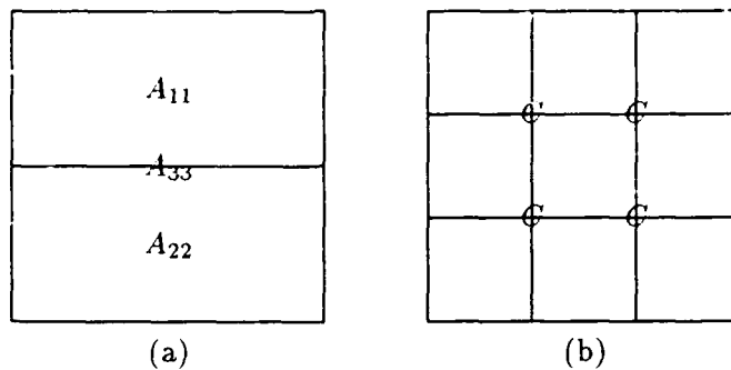
Figure 1: Two forms of decompositions. A two domain strip decomposition is shown in (a); a many domain box decomposition with cross points (labeled "C") is shown in (b).
