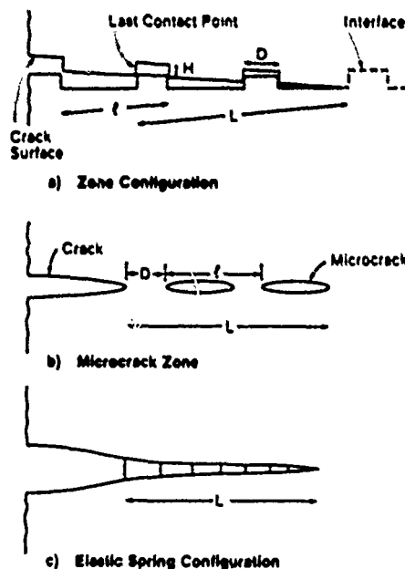
Fig. 9. A schematic illustrating the zone model used to determine trends in G_i with phase angle of loading.
