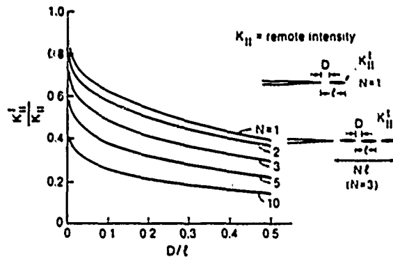
Fig. 10. Stress intensity at tip of lead microcrack in an array of equally spaced microcracks ahead of a macrocrack.
