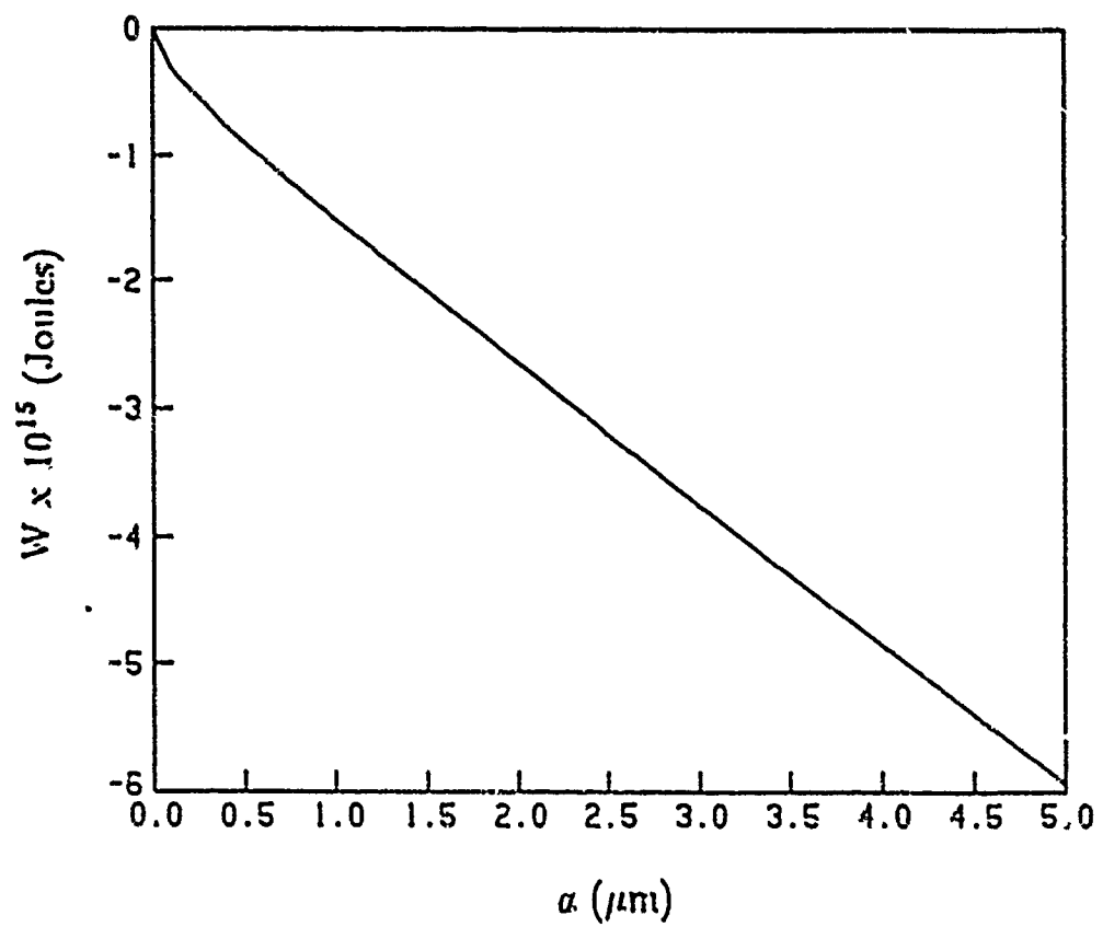
Fig.9 Total energy ( W ) versus dislocation spreading length ( a ) for c_s = 0.01 and h = 70 nm.
