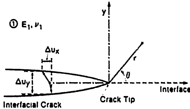
Fig. 6. The near tip crack surface displacements used in CSD method. In this figure, \Delta u_x = i\Delta u_y = \Delta u_x + i\Delta u_y , used in (14) and (19).
