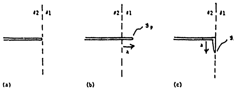
Fig. 9 Competition between crack penetration and deflection at an interface: (a) main crack at interface, (b) penetration of interface, and (c) deflection by interface.
