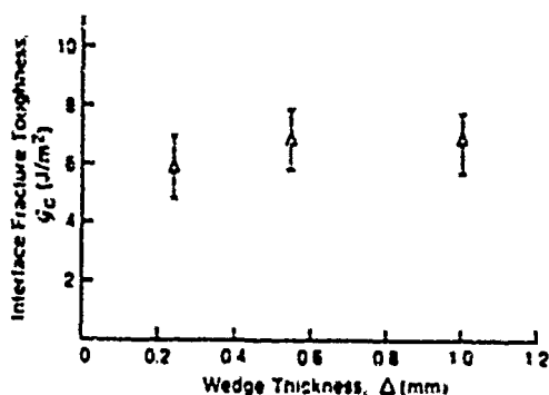
Fig. 9. Interface fracture resistances obtaining using asymmetric cantilever specimens ( \psi = 36^\circ ) for three wedge thicknesses.
