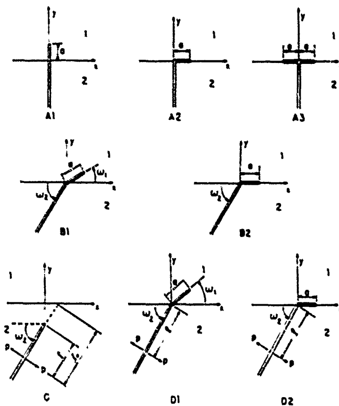
Fig. 1. Crack geometries.
