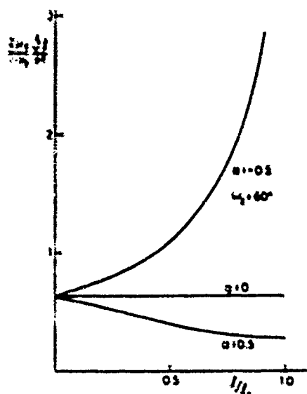
Fig. 9. Normalized energy release rate for straight crack approaching an interface at \omega_2 = 60^\circ , \beta = 0 .
