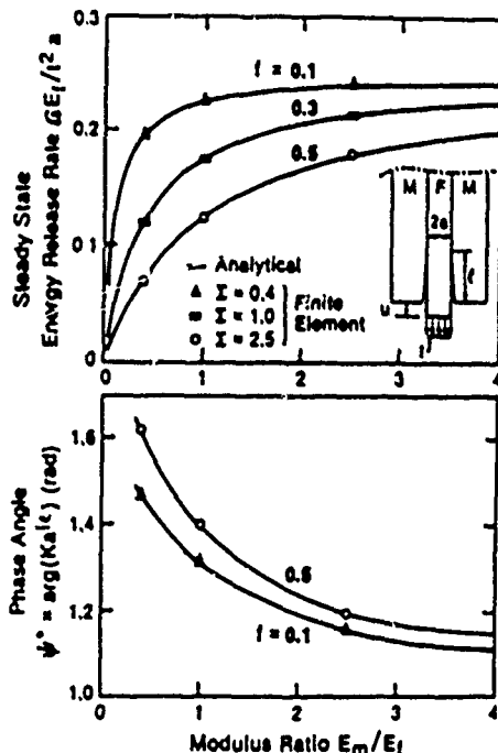
Fig. 6. Nondimensional strain energy release rate and phase angle: trends with modulus ratio and volume fraction for \nu_f = \nu_m = 0.25 .
