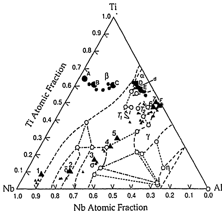
Figure 5 --The composition profiles between the \gamma -TiAl and the Nb (triangles) and TiNb (circles) particles plotted on the 1200°C Ti-Al-Nb isotherm (9). The numbers or letters on the larger symbols reference positions shown in Figure 6. The smaller symbols are for spectra taken at other nearby positions.
