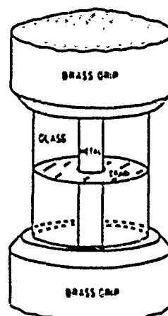
Fig. 3 A diagram of the sample immediately before testing. The crack is introduced by scoring the glass with a diamond and applying a small, intense, heat source
