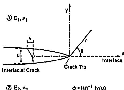
Fig. B1. Displacement field associated with a crack at a bimaterial interface.
