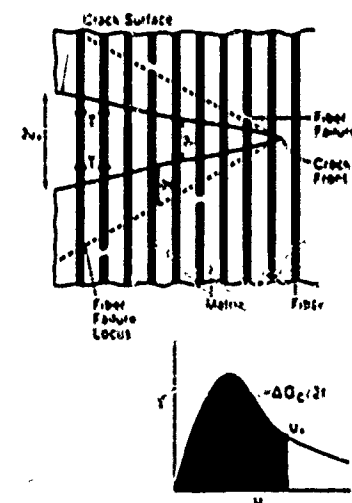
Fig. 1. Schematic illustration of fiber failure occurring away from the matrix crack plane.
