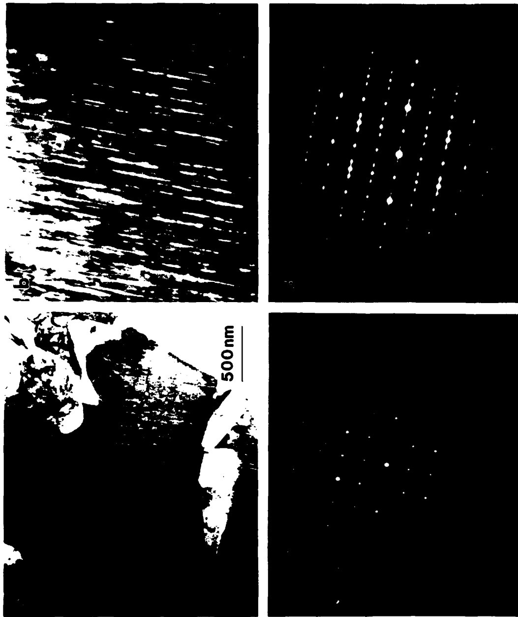
Figure 8. TEM microstructures of Ti-48Al XSR fine powder ( <25\mu\text{m} ): (a) \alpha_2 dendrite partially transformed to (\alpha_2 + \gamma_1) , surrounded by the \gamma -segregate; (b) very fine (\alpha_2 + \gamma_1) lath within the dendrite. The zone axis patterns are: (c) [1210]\alpha_2 and (d) [1210]\alpha_2/[110]\gamma_1 for the untransformed and transformed regions, respectively.
