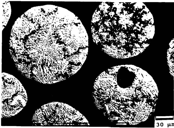
Figure 85 Microstructure, alloy G (Ti50-Al48-Nb2), CM features in AM matrix, 88-150 microns.
