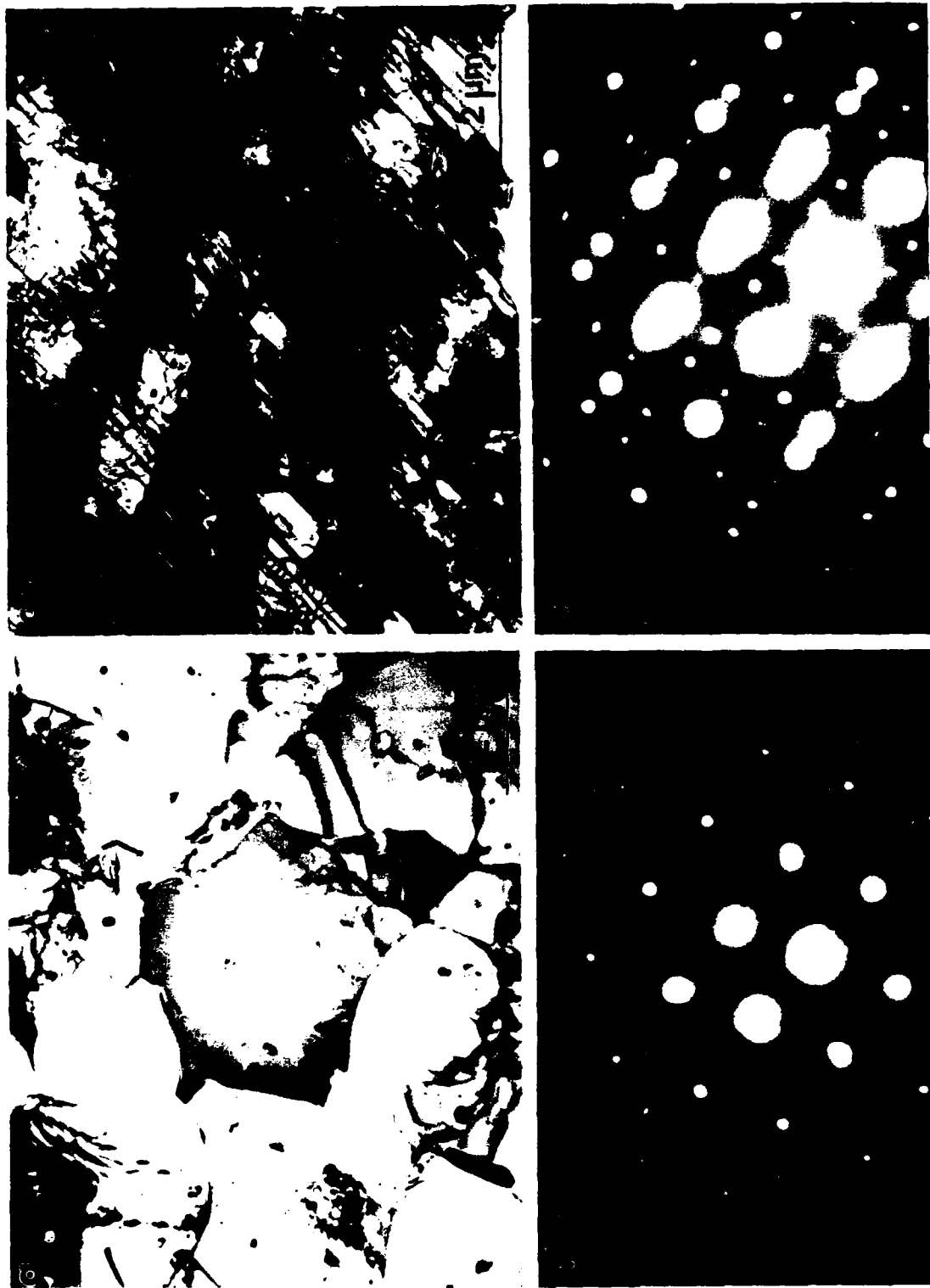
Figure 5. TEM micrographs of vacuum hot forged billet prior to high temperature X-ray; (a) fine grained \gamma , (b) [101]_\gamma zone axis, (c) area containing \gamma twins and \alpha_2 laths, (d) zone axis showing a single [1210]_\alpha zone and two twin related [110]_\gamma zones.
