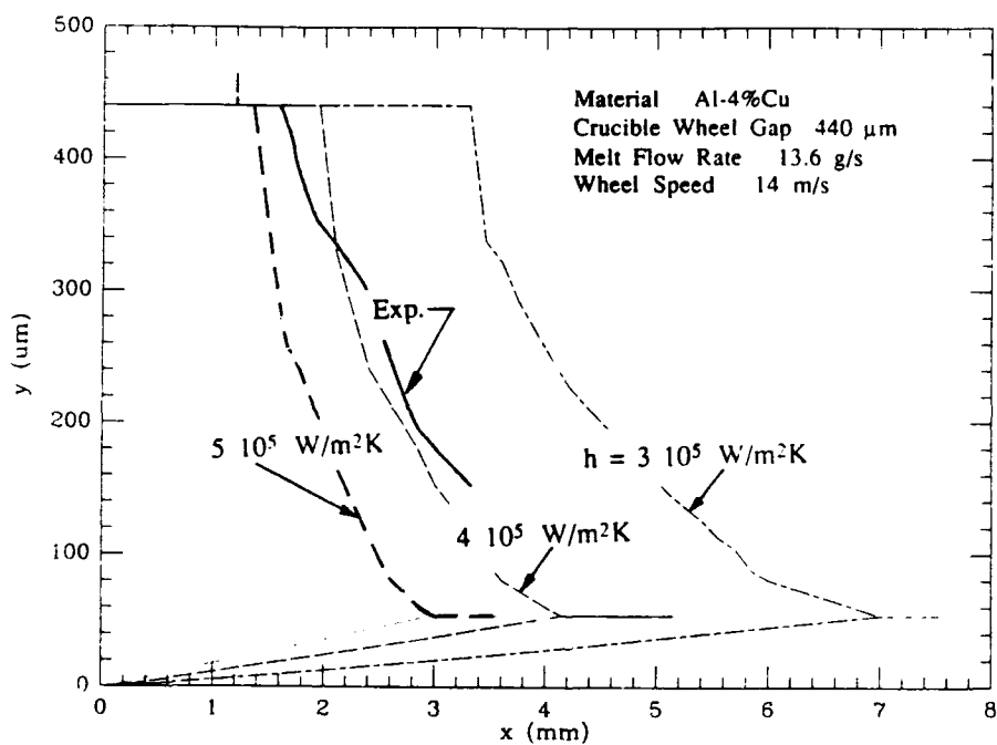
Figure 10 : Comparison of measured detachment point and downstream meniscus shape with predicted values corresponding to different heat transfer coefficients at the wheel. The best match is for 4 \cdot 10^5 \text{ W/m}^2\text{-K} . [Al-4%Cu; gap: 440 microns; flow rate: 13.6 g/s; wheel speed: 14 m/s.]
