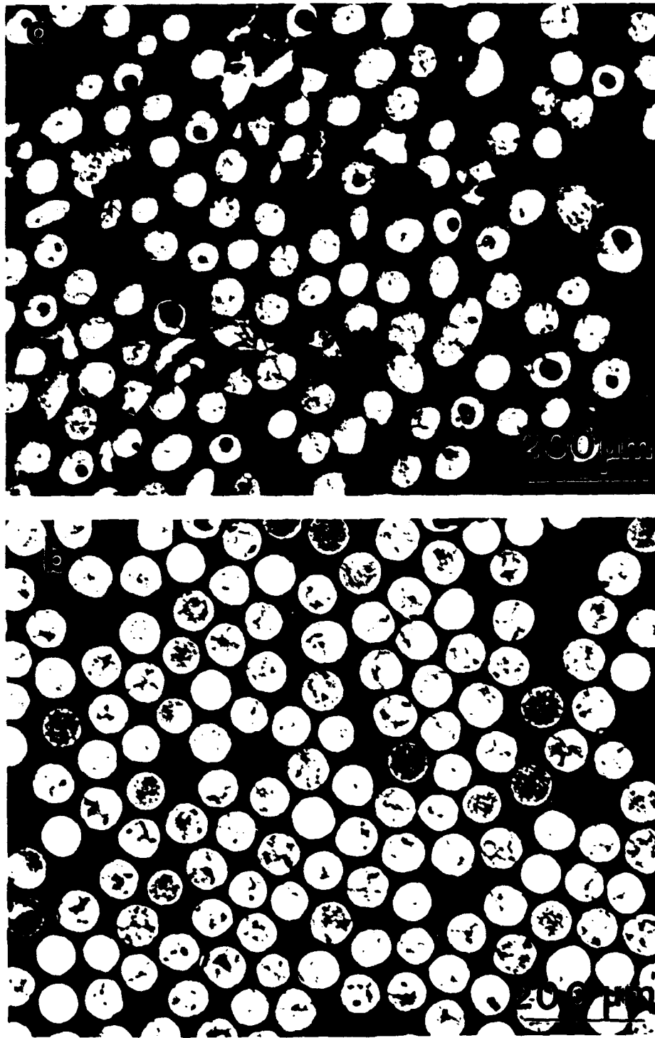
Figure 3. Cross sections of 63 \mu m to 75 \mu m size powders; (a) RSR, (b) REP.
