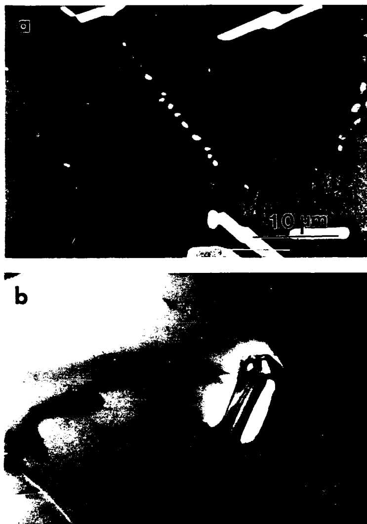
Figure 12.- Precipitation of equiaxed Ti_2AlC in Ti-50.8Al-2.8C after heat treatment (1473 K/100 hrs.) (a) BEI of precipitates at grain boundary. (b) TEM view of carbide particle and matrix devoid of fine clustering (compare with Figure 8a).
